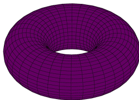
Figure 9. Torus
