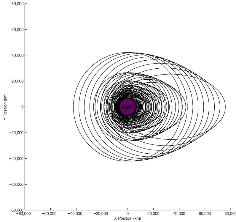
Figure 4. Resonant Orbits
