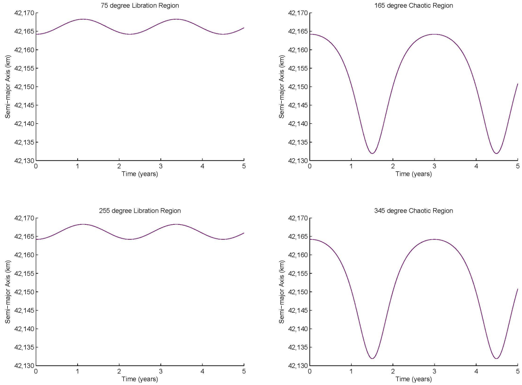
Figure 7. Semimajor Axis of Orbits near Equilibrium Points
