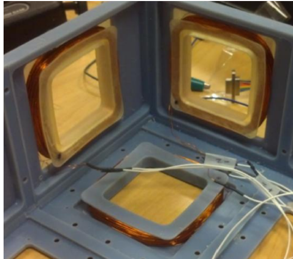
Figure 68. Three Magnetic Torque Coils Installed in a Plastic Chassis [12]
