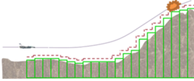
Figure 16. The Auto GCAS Automatic Maneuver and Terrain Projection Comparison
