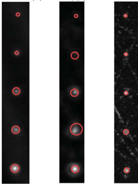
Figure 67. Sample L-41 as-manufactured top surface with roughness of 11.1\ \mu\text{m RMS} (a) 2.25 MHz, (b) 5 MHz, (c) 10 MHz
