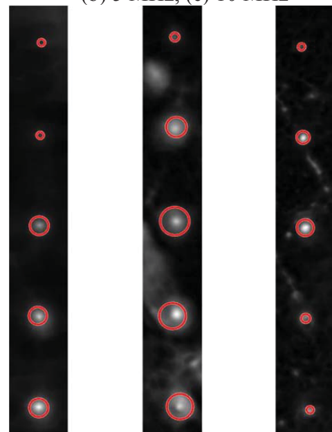
Figure 69. Sample M-41 as-manufactured top surface with roughness of 18.3\ \mu\text{m RMS} (a) 2.25 MHz, (b) 5 MHz, (c) 10 MHz
