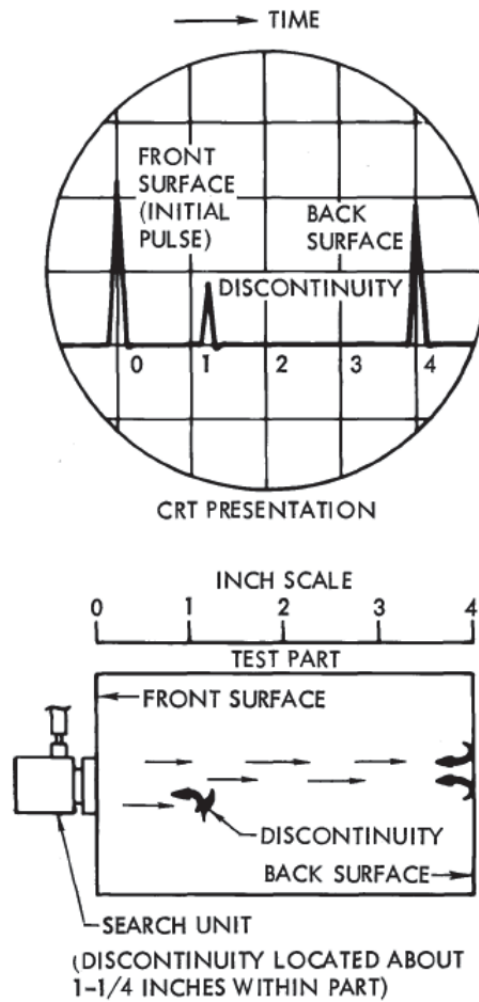
Figure 7. Example of A-Scan indication of imbedded flaw in sample [13]
