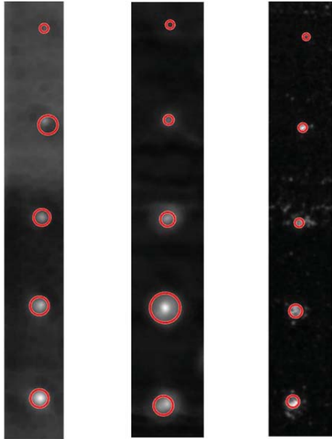
Figure 66. Sample E-42 as-manufactured top surface with roughness of 15.5\ \mu\text{m RMS} (a) 2.25 MHz, (b) 5 MHz, (c) 10 MHz
