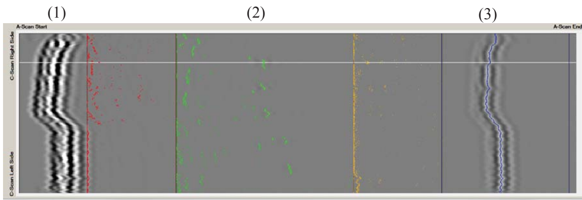
Figure 8. Example of ultrasonic B-Scan scan through top surface (1) signal return of top surface, (2) flaw indication, (3) signal return of back surface
