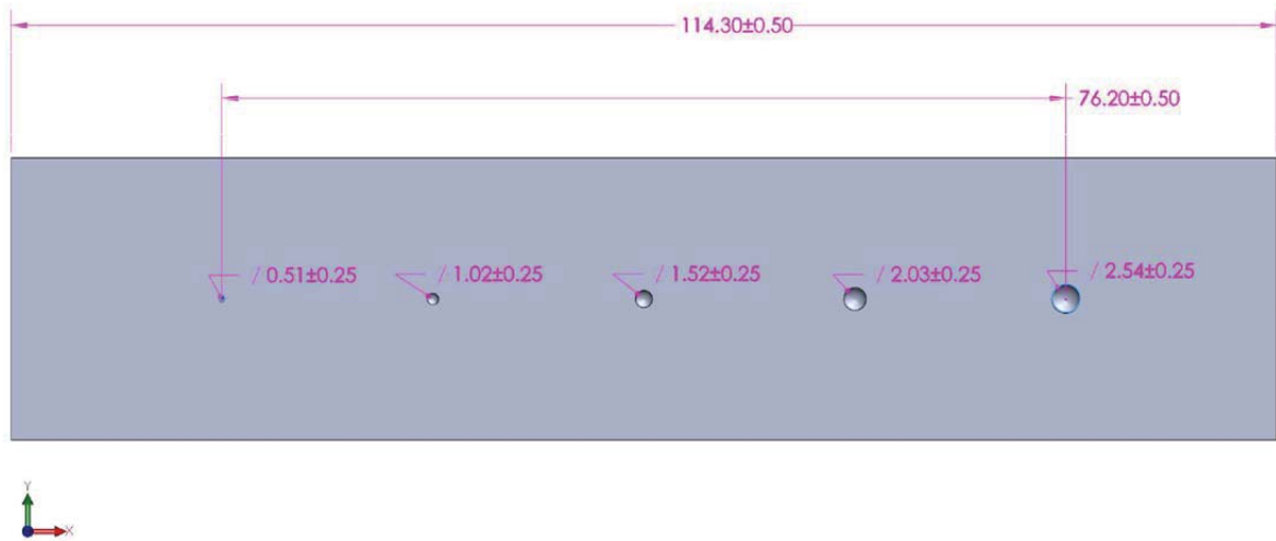
Figure 13. CAD design of samples to include defects with dimensions in mm
