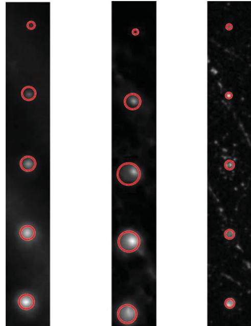
Figure 68. Sample L-42 as-manufactured top surface with roughness of 16.5\ \mu\text{m RMS} (a) 2.25 MHz, (b) 5 MHz, (c) 10 MHz
