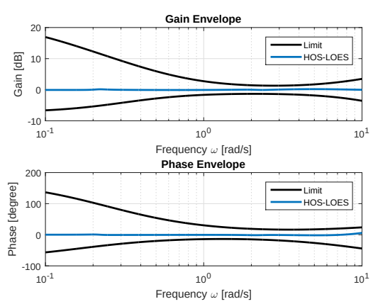
Figure 99. Envelope \phi/\delta_a at 8000 ft
