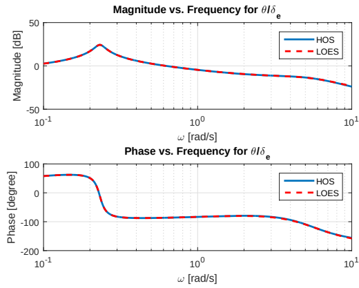
Figure 108. Bode Plot for \theta/\delta_e at 20000 ft
