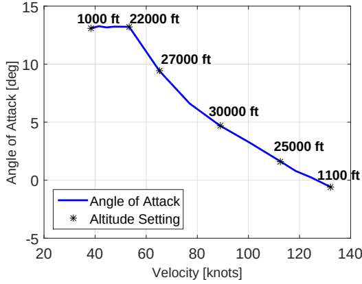
Figure 36. Angle of Attack at Trim for T-41
