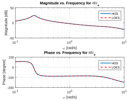
Figure 100. Bode Plot for \theta/\delta_e at 12000 ft
