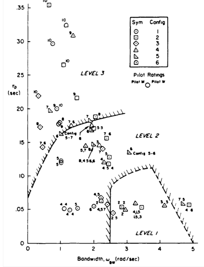
Figure 9. Bandwidth Requirements [1]
