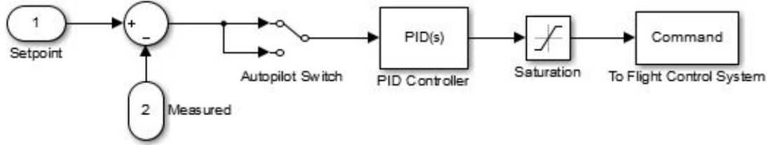
Figure 27. Outer Autopilot Controller Structure
