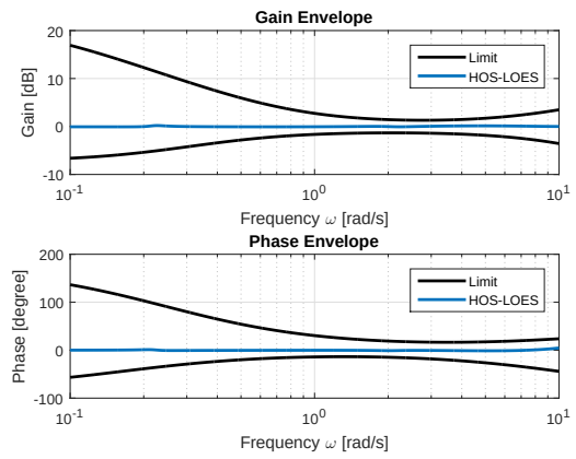
Figure 103. Envelope \phi/\delta_a at 12000 ft
