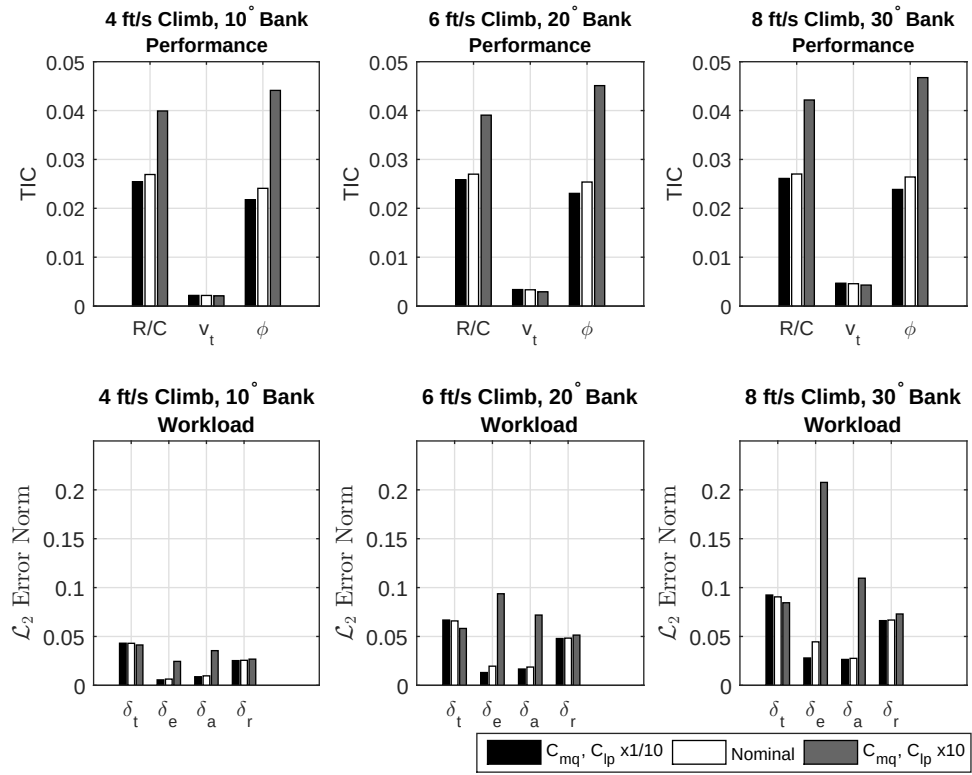
Figure 88. Coupled Maneuver: Performance and Workload Comparison of Nominal and C_{mq} , C_{lp} Variation
