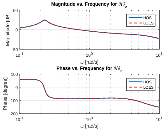
Figure 104. Bode Plot for \theta/\delta_e at 16000 ft
