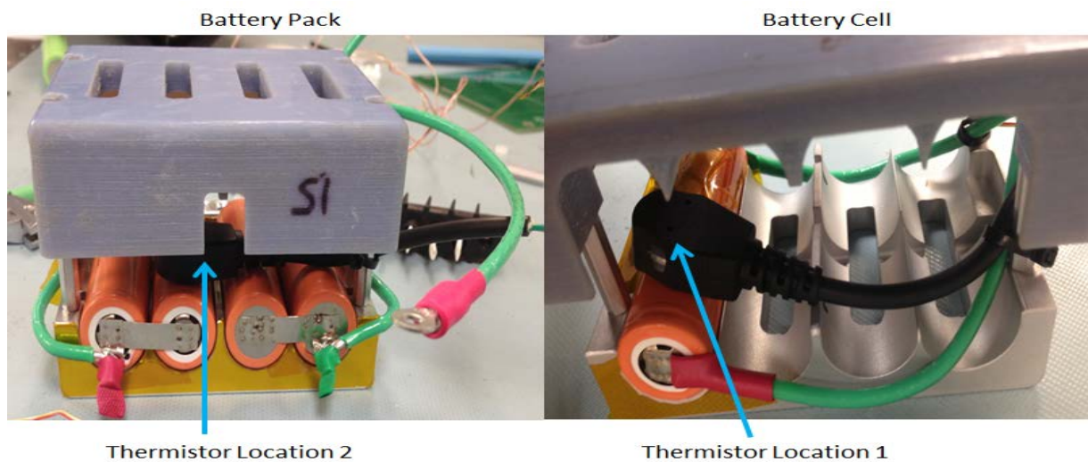
Figure 32: Thermistor Locations
