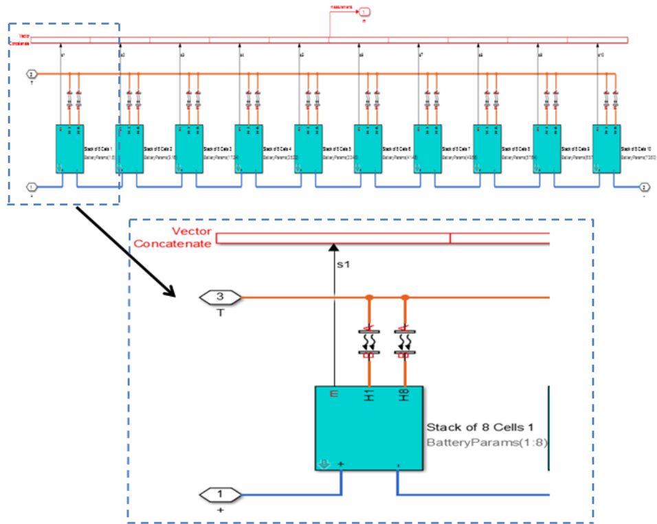
Figure 11: Battery Pack (2S2P) mask contents before modification. The original HJGC model contained 10 Stack of 8 Cells masks each containing 8 Lithium Cell masks.
