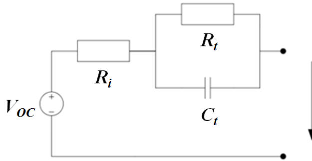
Figure 6: Thevenin Equivalent Circuit Model
