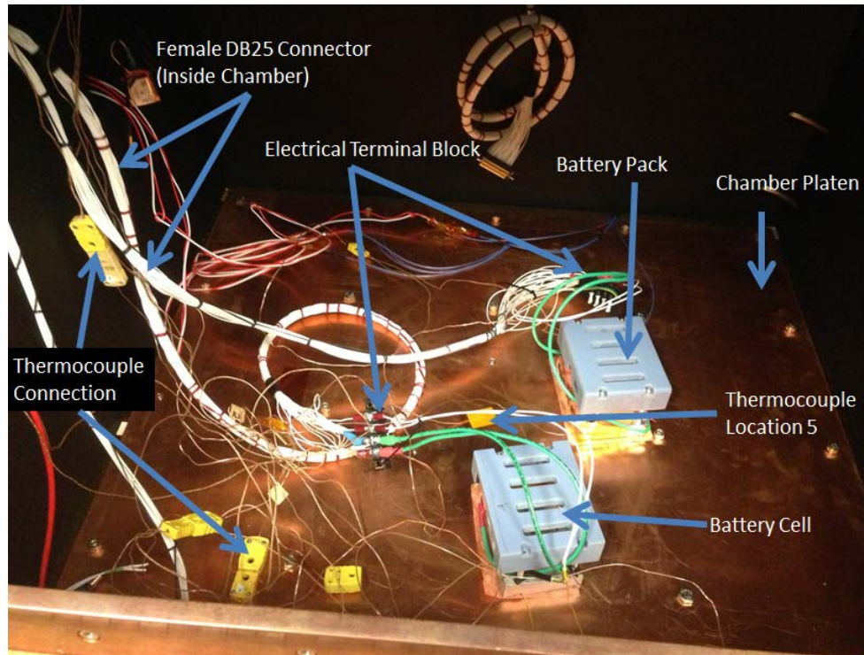
Figure 34: Test Setup inside Chamber without Metal Block Weight
