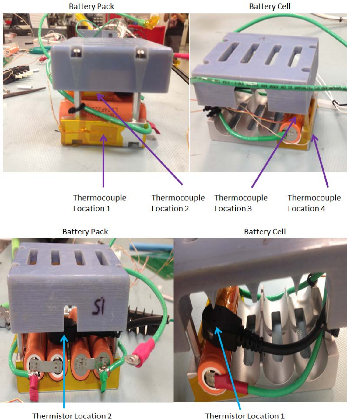
Figure 65: Thermocouple and Thermistor Location
