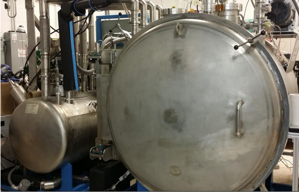
Figure 12. Space simulator vacuum system.
