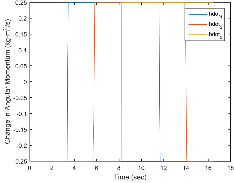
Figure 4.29: Experimental and Simulated Open Loop Optimal Controller 90 Degree Z-Axis Reorientation \dot{\vec{h}} Trajectory
