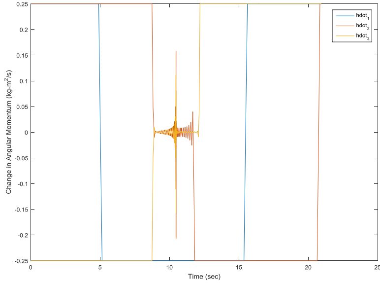
Figure 4.34: Experimental and Simulated Open Loop Optimal Controller 180 Degree Z-Axis Reorientation \dot{\vec{h}} Trajectory
