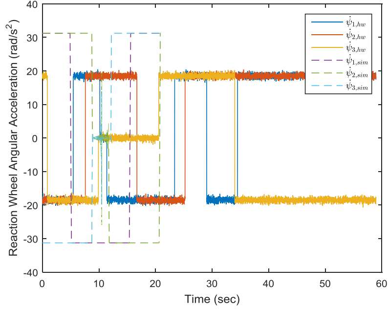
Figure 4.33: Experimental and Simulated Open Loop Optimal Controller 180 Degree Z-Axis Reorientation Reaction Wheel Angular Accelerations
