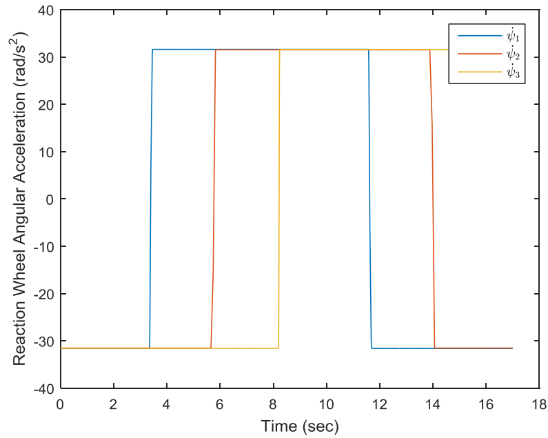
Figure 4.12: Simulated Open Loop Optimal Control 90 Degree Z-Axis Reorientation Reaction Wheel Angular Accelerations
