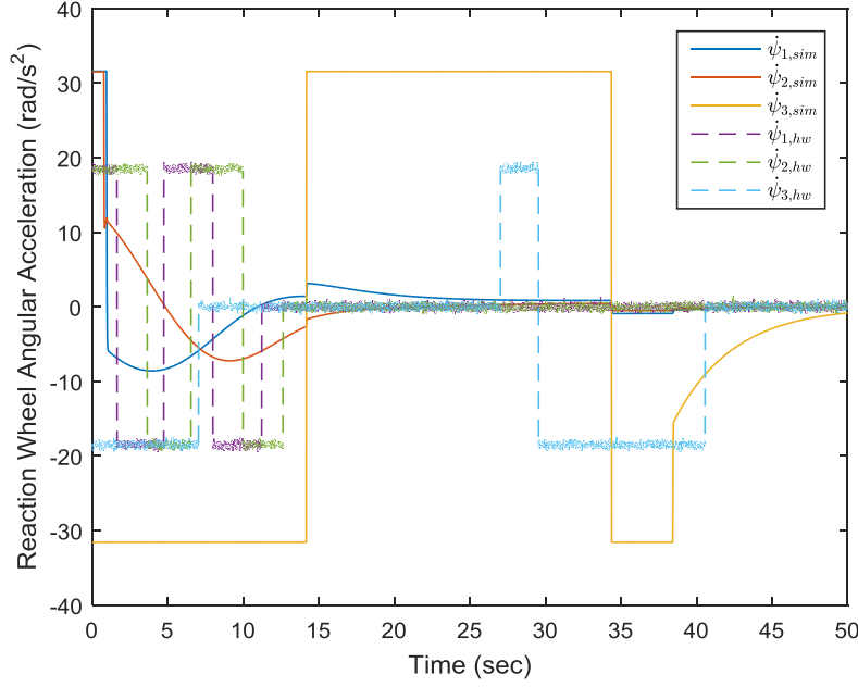
Figure 4.20: Experimental and Simulated PID Controller 90 Degree Z-Axis Reorientation Reaction Wheel Angular Accelerations
