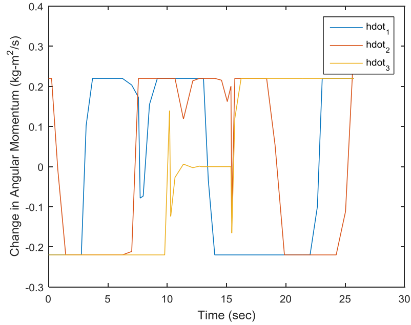
Figure 4.46: Hardware Near RTOC Controller 180 Degree Z-Axis Reorientation \dot{h} Trajectory 1
