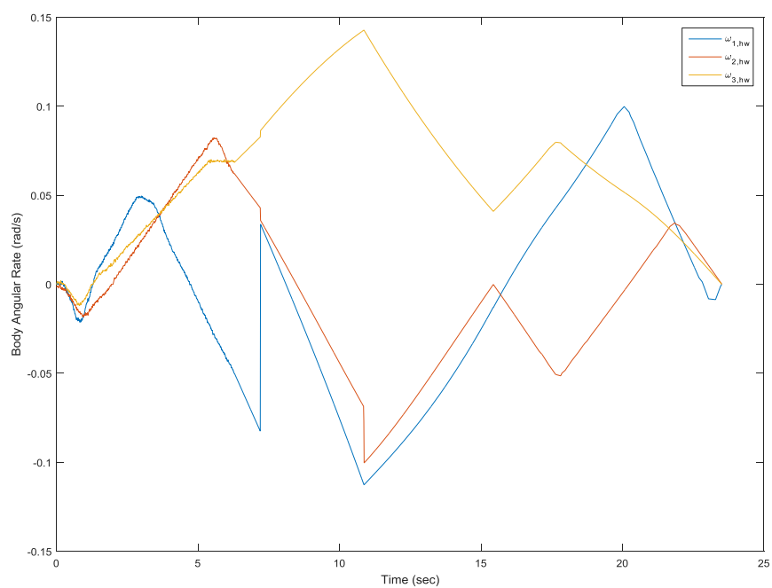
Figure 4.36: Hardware Near RTOC Controller 90 Degree Z-Axis Reorientation Body Angular Rates
