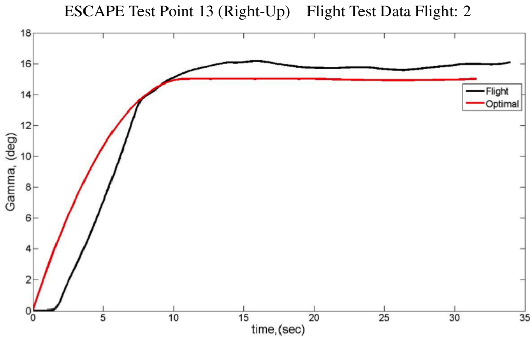
Figure 4.24: Flight Test Flight Path Angle vs Optimal Flight Path Angle
