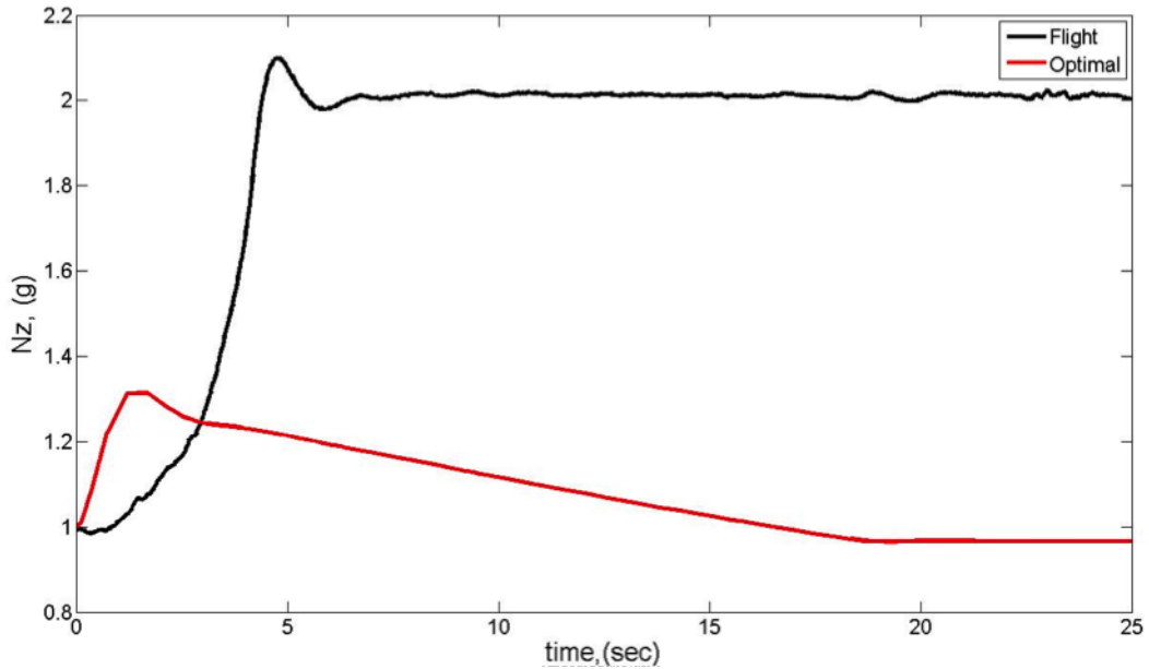
Figure 4.19: Flight Test N_z vs Optimal N_z
