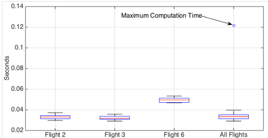
Figure 4.11: Overall Processing Time for the 3-TPA Algorithm
