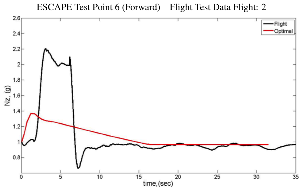
Figure 4.15: Flight Test N_z vs Optimal N_z
