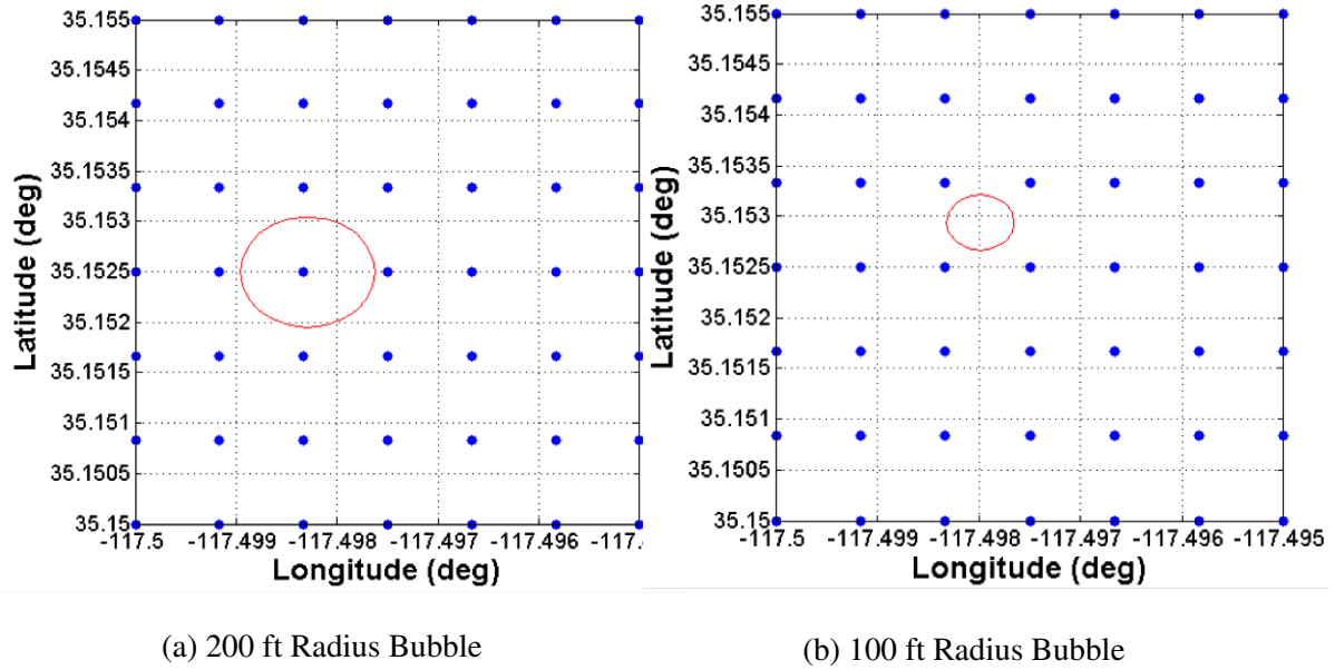
Figure 4.10: Minimum Post Identification for Level 1 DTED
