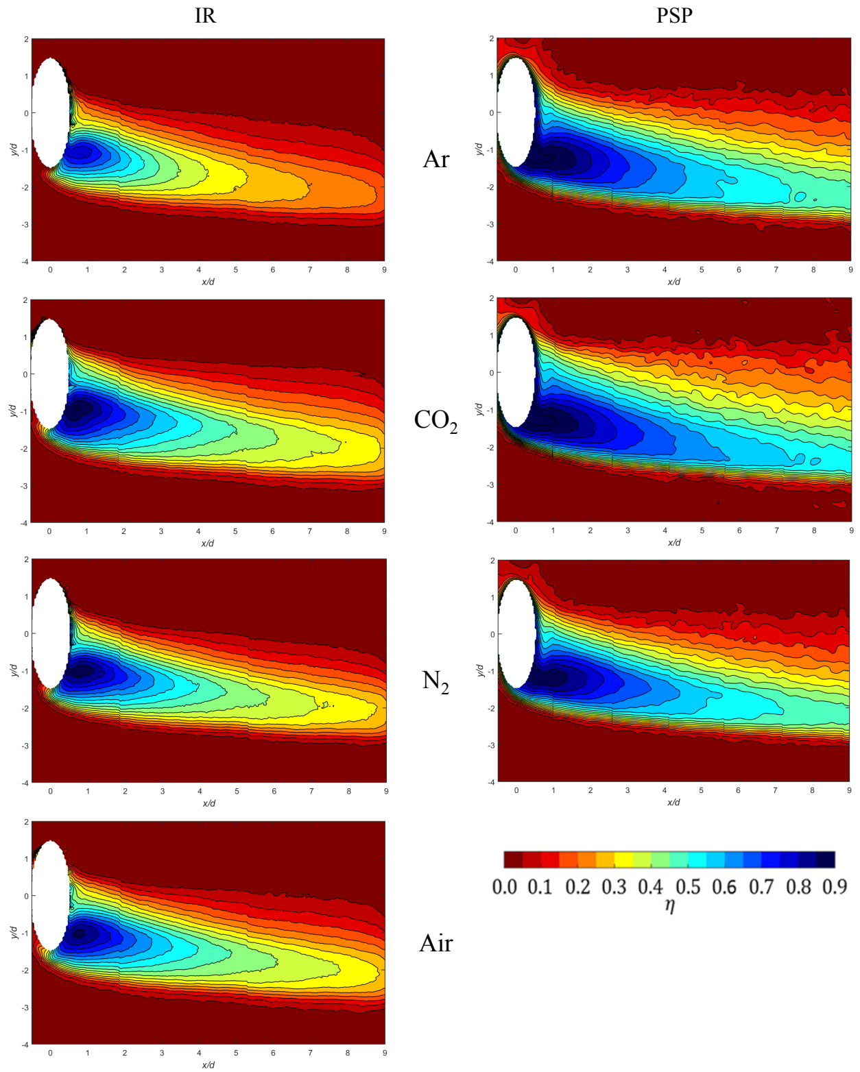
Figure 4.16. Adiabatic effectiveness contours at I = 1.0 , IR (Left) and PSP (Right) methods
