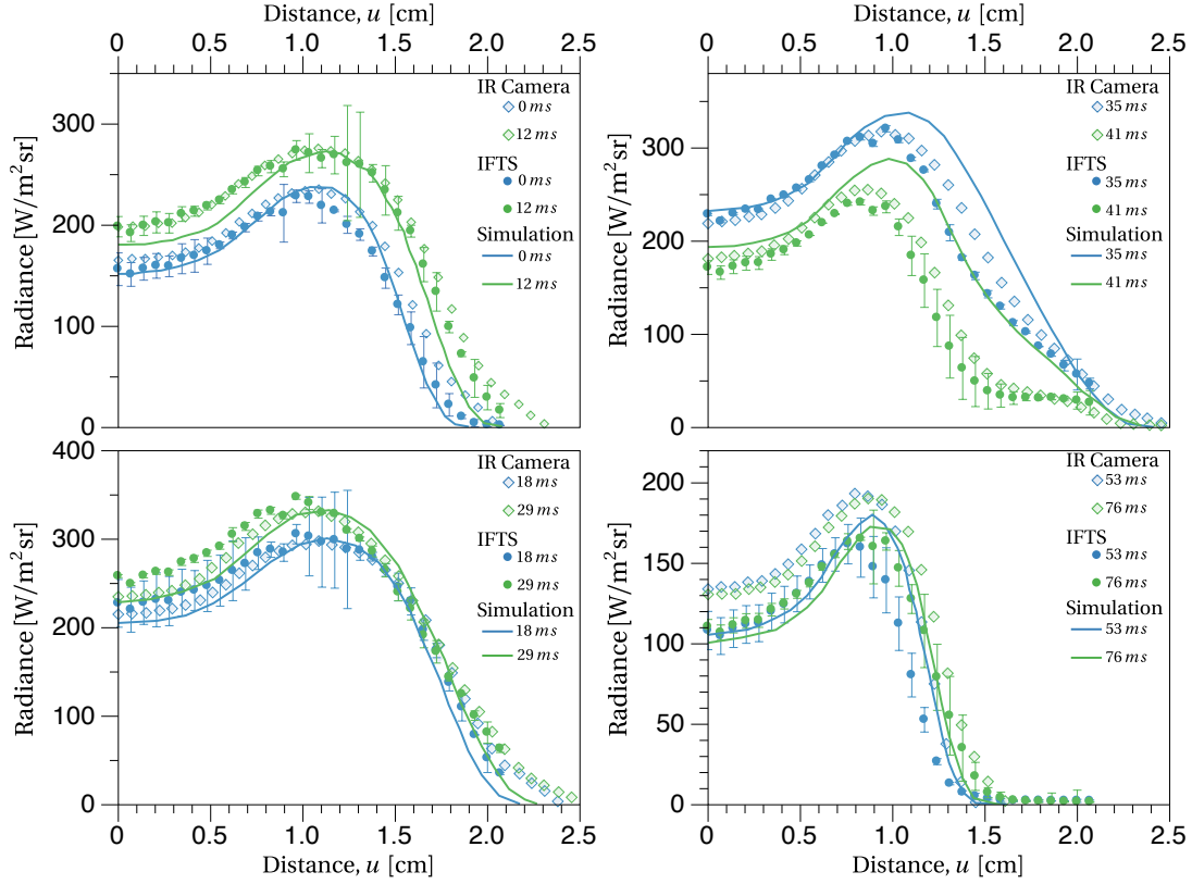
Figure 33. Comparison of reconstructed, previous experimental [2], and simulated LOS flame radiance profiles for several times in a single flame period at a height of v = 4.5 cm. Error bars represent the one standard deviation confidence interval.
