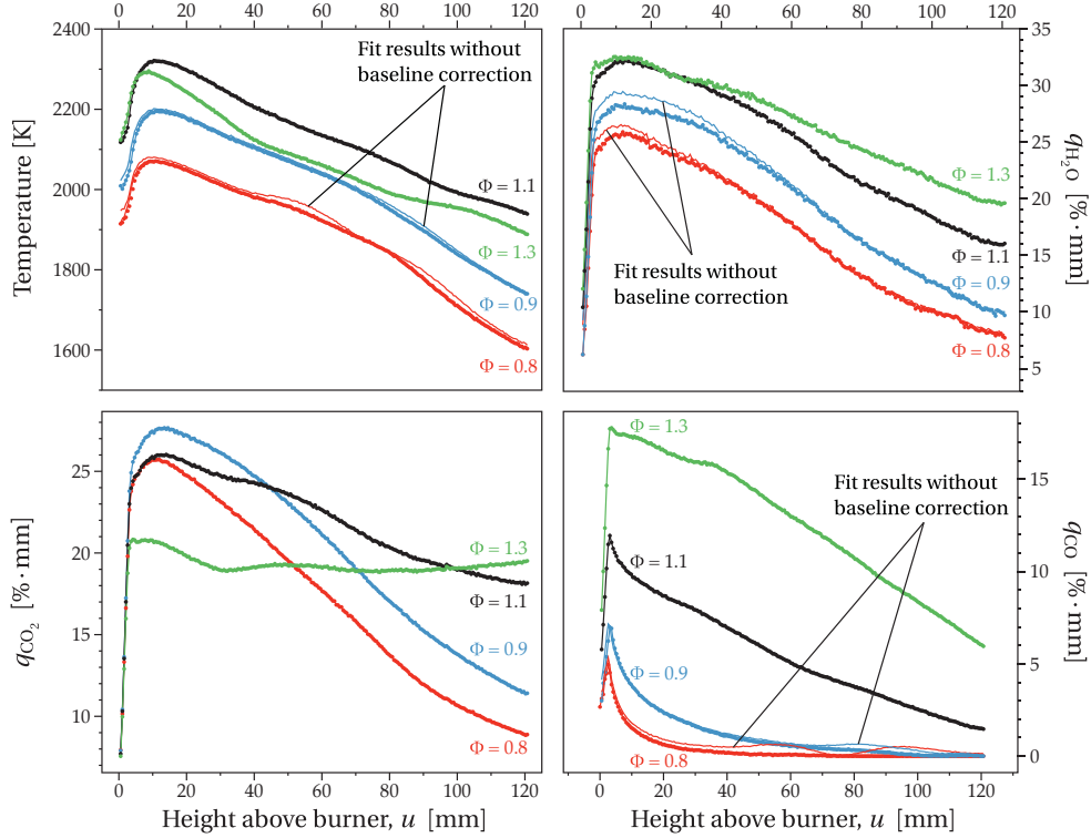
Figure 21. Spectrally-retrieved scalar values of the \text{C}_2\text{H}_2/\text{air} flame, along the centerline ( v = 0 ), for \Phi = 0.8 (● red), \Phi = 0.9 (● blue), \Phi = 1.1 (● black), and \Phi = 1.3 (● green). Error bars are omitted for clarity. Fit results obtained without the polynomial baseline correction for \Phi = 0.8 (— red) and \Phi = 0.9 (— blue) are annotated.
