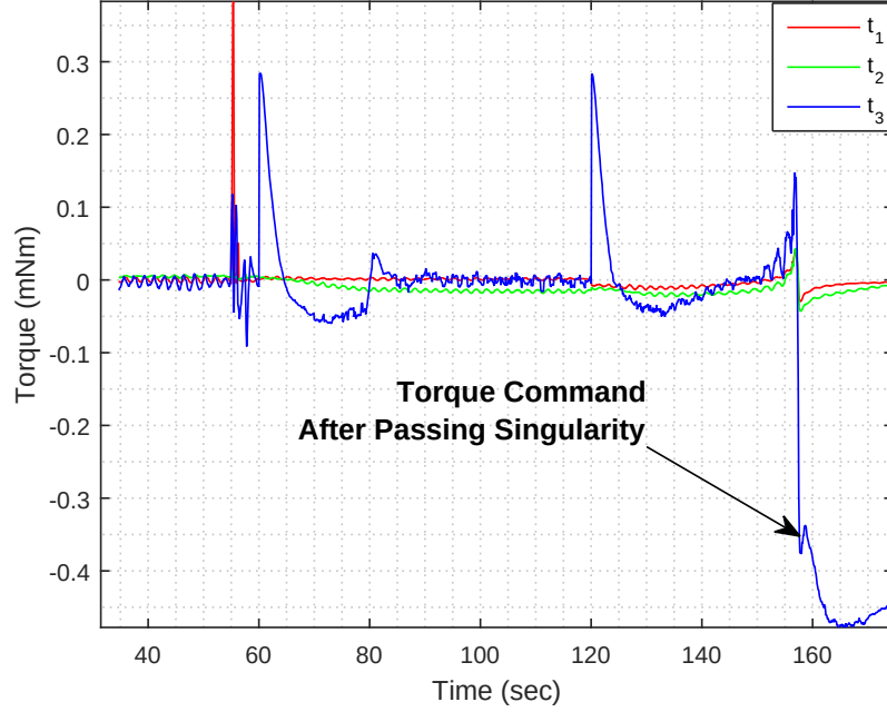
Figure 60. Commanded Torque During Test 1
