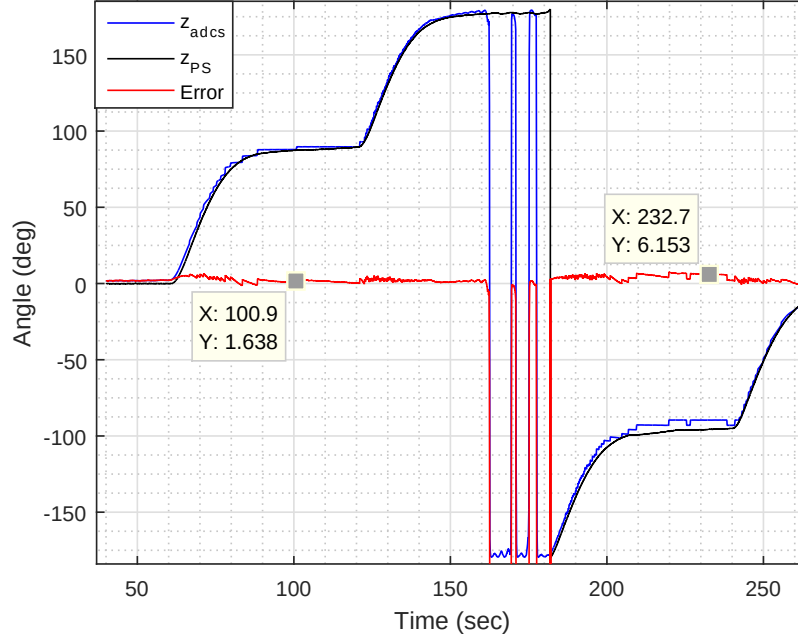
Figure 77. Angle Error During 360° Rotation
