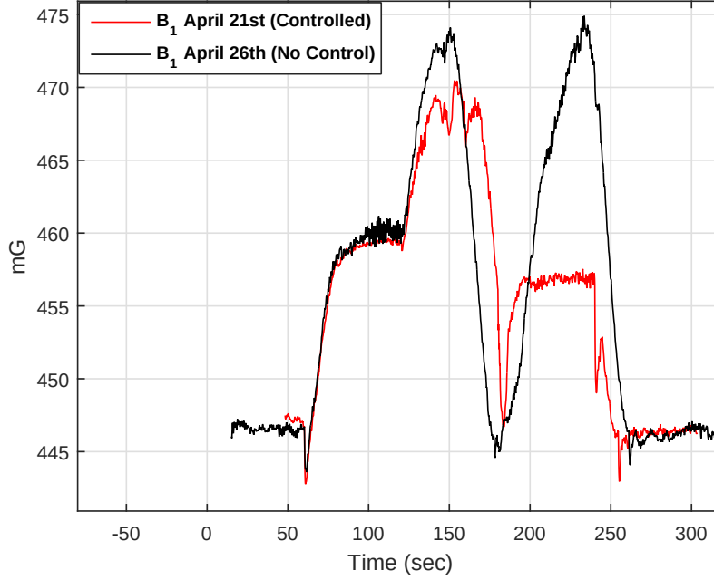
Figure 79. B_1 Plot Before and After Solar Activity 360° Rotation
