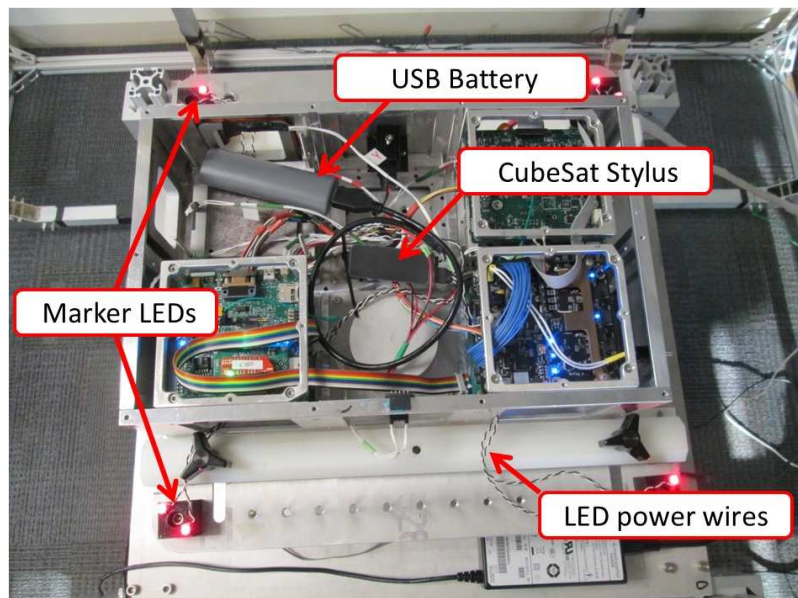
Figure 26. PhaseSpace LED Placement on ADCS Test Bed
