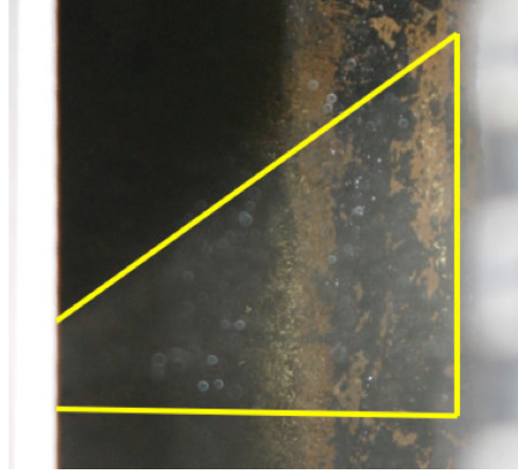
Figure 37. Devalan Nozzle Spray Cone Half-Angle Highlighted
