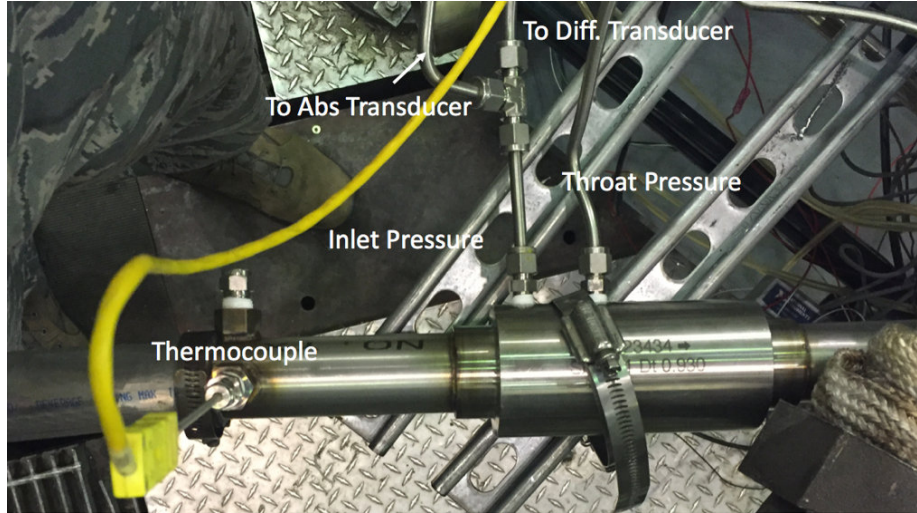
Figure 35. Venturi Calibration Set Up
