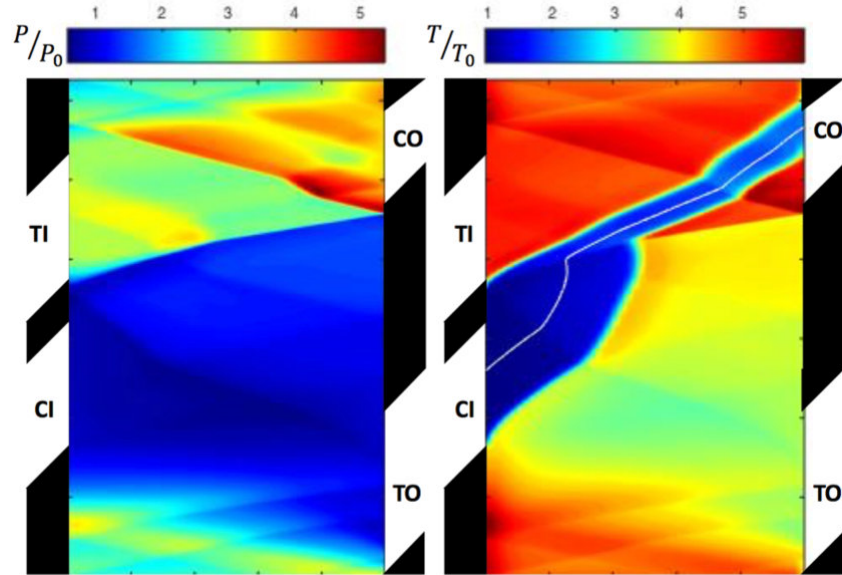
Figure 47. Cycle Temperature of Four x-t Diagram
