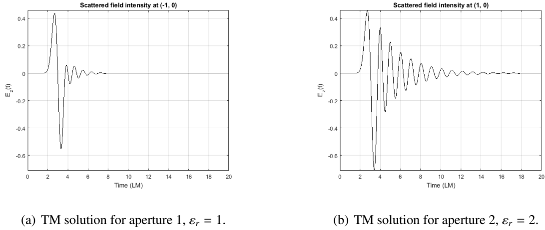
Figure 5.16: Field values at midpoints of apertures.
