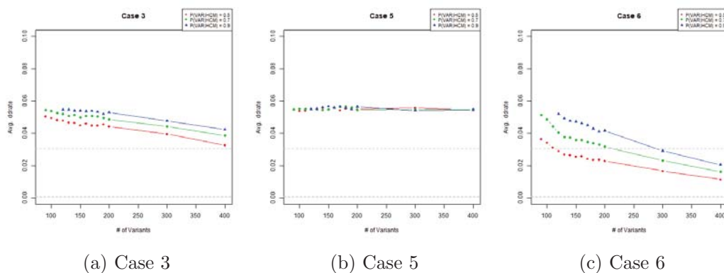
Figure S26: discharge deathrate, where the \# of variants were changed for three different constant values of P(VAR|HCM) . Notice that the slopes of the lines for Case 6 are the most negative, and the slopes of the lines for Case 3 have smaller magnitudes, while Case 5 has nearly flat lines. Increasing P(VAR|HCM) shifts the curves up. Lower Dotted grey line is the average value of DDrate for Case 2, upper dotted grey line is the average value of DDrate for Case 4.
