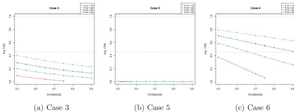
Figure S19: FDR, where the P(VAR|HCM) was changed for four different constant values of # of variants . Cases 3 and 6 have negative slopes, with Case 6 having a greater slope and more variation in intercepts for different values of # of variants . Case 5 has flat lines at approximately 0. The lower dotted grey line represents the average value for the FDR of Case 4, the upper dotted grey line represents the average value for the FDR of Case 2.
