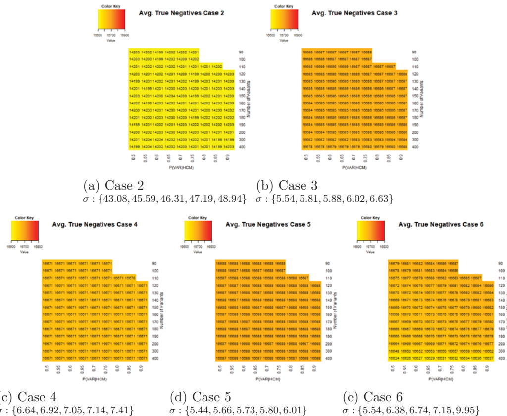
Figure S41: Heatmaps of the average number of True Negatives for each Officer case. Standard deviation summary given as: \sigma : \{\text{min, 25th quantile, median, 75th quantile, maximum}\} .
