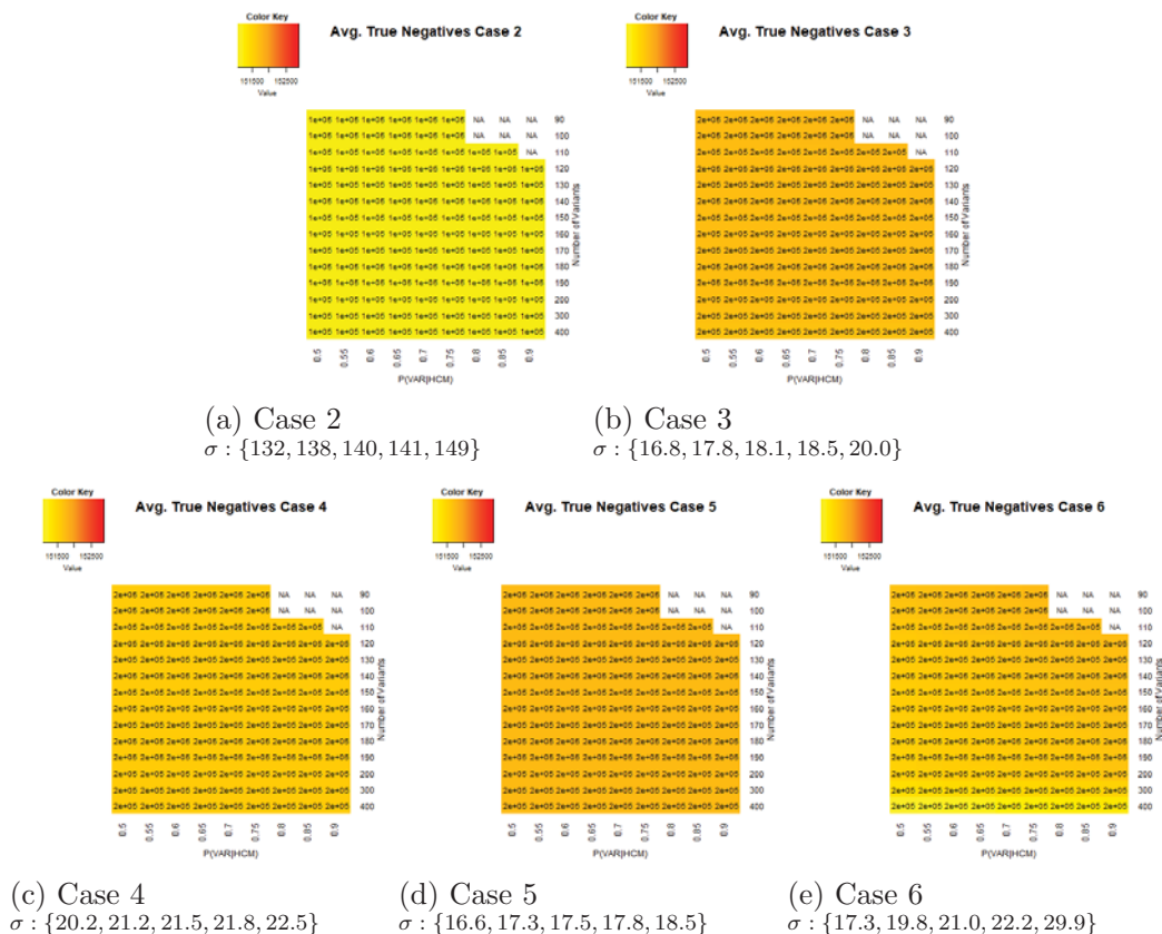
Figure S45: Heatmaps of the average number of True Negatives for each enlisted case. Standard deviation summary given as: \sigma : {min, 25th quantile, median, 75th quantile, maximum}.
