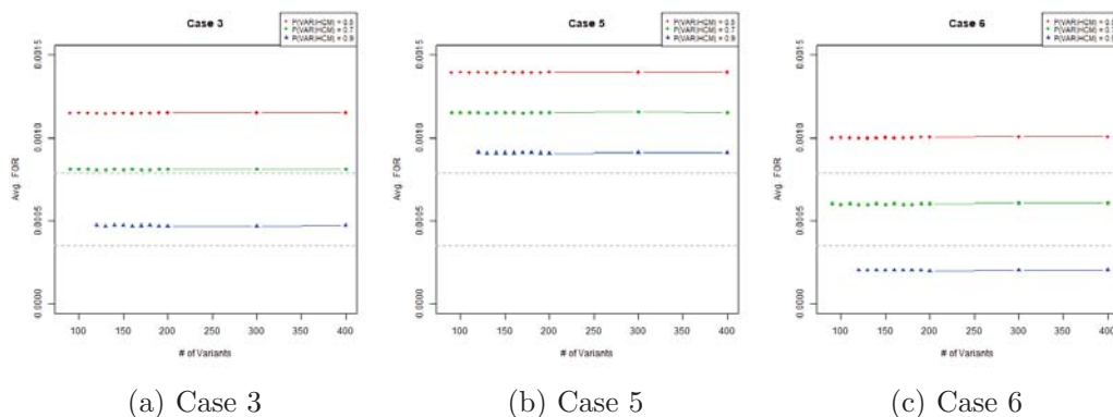
Figure S21: FOR, where the \# of variants were changed for three different constant values of P(VAR|HCM) . Notice that the slopes of the lines are approximately zero. Increasing P(VAR|HCM) shifts the curves up. Lower dotted grey line is the average value of FOR for Case 2, upper dotted grey line is the average value of FOR for Case 4.
