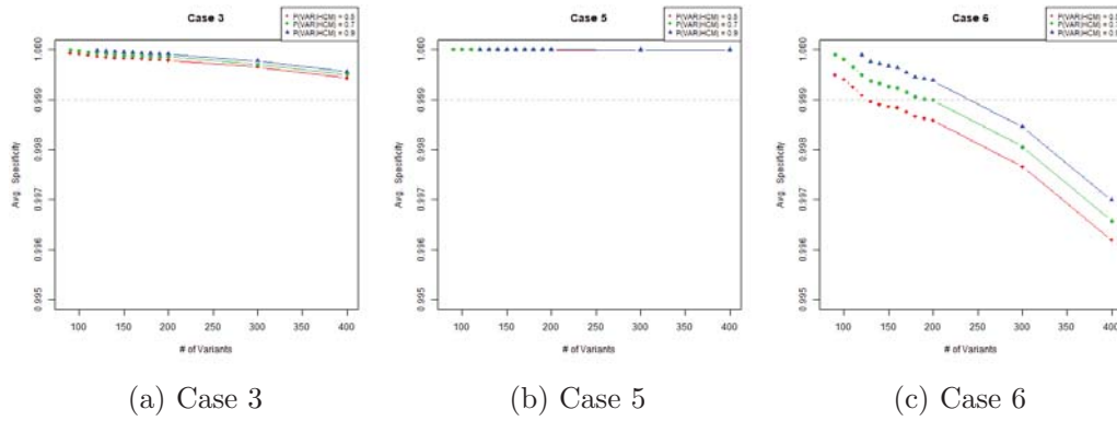
Figure 42: Specificity, where the \# \text{ of variants} were changed for three different constant values of P(VAR|HCM) . Notice that the slopes of the lines for Case 6 are the most negative, and the slopes of the lines for Case 3 have smaller magnitudes, while Case 5 has flat lines. Increasing P(VAR|HCM) shifts the curves up. Dotted grey line is the average value of specificity for Case 4.
