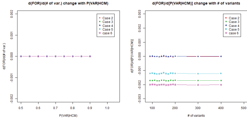
Figure S5: \frac{\partial FOR}{\partial \# \text{ of variants}} is seen to be most negative for Case 6, followed by Case 3 and Case 5, and zero for cases 2, 4. \frac{\partial FOR}{\partial P(VAR|HCM)} is seen to be approximately zero. All values appear to be constant for the variation of the constants for the partial derivatives.
