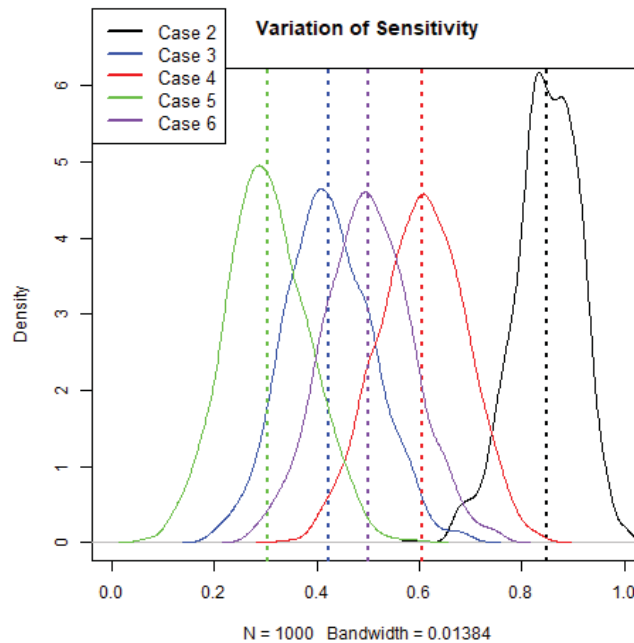
Figure 81: Variation among the 1000 officer simulations for sensitivity for a values P(VAR|HCM) = 0.5 and \# of variants = 130 . The means of the sensitivities of the cases are displayed as dotted vertical lines. Notice how the sensitivities vary among many values for each case, due to random differences in each simulation.
