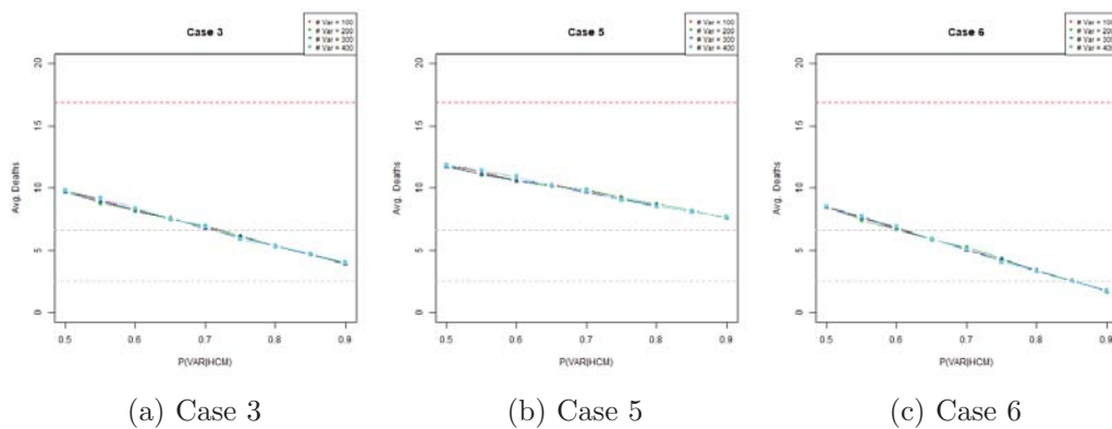
Figure S24: deaths, where the P(VAR|HCM) was changed for four different constant values of # of variants . Notice how all Cases have negative slopes.
