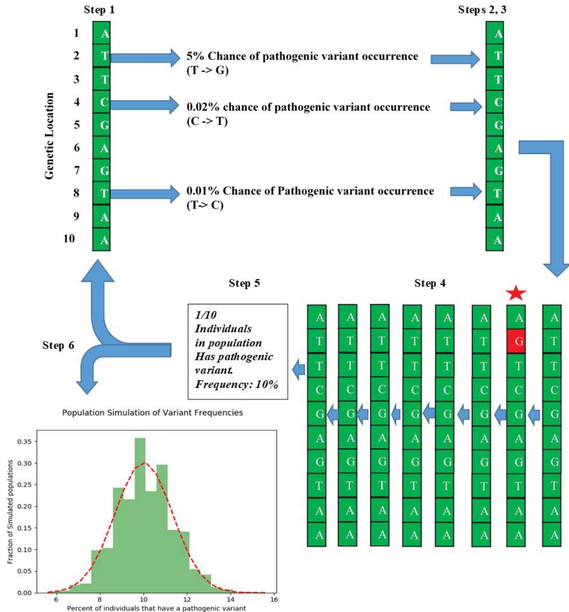
Figure 24: Simulation of populations. Certain locations in the reference genome have independent chances of being pathogenic for each individual. For each population, the frequency of individuals with a pathogenic variant was calculated. For a large number of random populations, the frequency of pathogenic variants in each population should have a range of values. Populations and genomes in this figure are not to scale.
