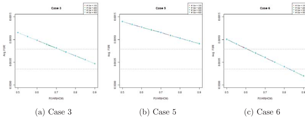
Figure S22: FOR, where the P(VAR|HCM) was changed for four different constant values of \# of variants. Cases 3, 5 and 6 all have negatives slopes, with the largest magnitude of slope of Case 6, followed by cases 3 and then 5. Notice how FOR does not change with changing values of \# of variants. Lower dotted grey line is the average value of FOR for Case 2, upper dotted grey line is the average value of FOR for Case 4.
