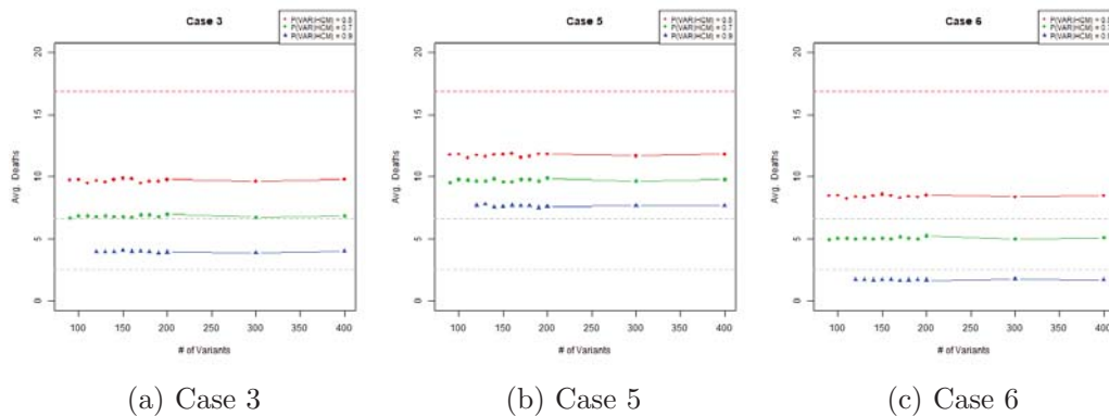
Figure S23: deaths, where the # of variants were changed for three different constant values of P(VAR|HCM) . Notice how the curves shift down for increasing P(VAR|HCM) and have relatively constant slopes.
