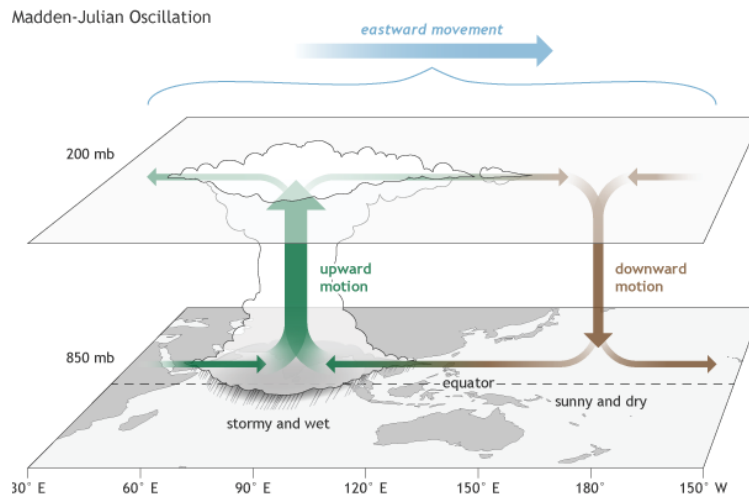
FIGURE 1: Atmospheric circulation and resultant convective activity typical of the active envelope of the MJO as it propagates through the MC. 2014 NOAA graphic by Fiona Martin.
