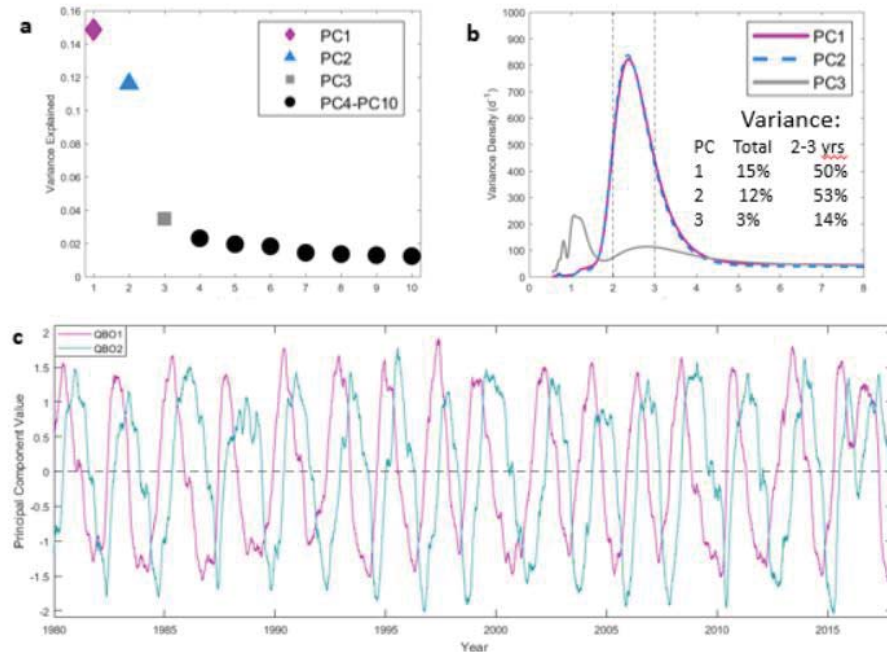
FIGURE 8: (a) Total variance of stratospheric winds from 1980-2017 accounted for by the first ten principal components of the EOF analysis, (b) variance density spectra of the first three principal components, and (c) daily time series of the first two principal components, normalized by their respective standard deviations (QBO1 and QBO2, respectively). Vertical lines in panel b denote periods between 2 and 3 years.
