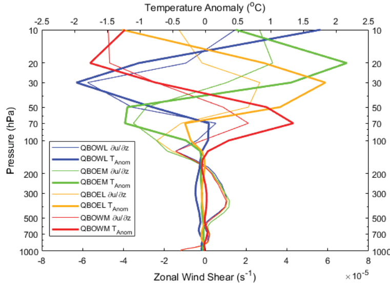
FIGURE 17: Mean (10°S-10°N, 0°E-360°E) zonal wind shear ( s^{-1} ; thin lines) and temperature anomalies ( ^{\circ}C ; thick lines) for the QBO phase pairs (QBOWL, QBOEM, QBOEL, and QBOWM), in all months from 1980-2017.
