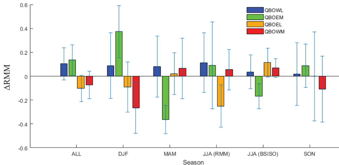
FIGURE 19: Mean amplitude change difference from climatological (1980-2017) average for initially active MJO events, binned by QBO phase pair and seasonal subset. Amplitude changes are presented for the full year (ALL), December-February (DJF), March-May (MAM), June-August (JJA), and September-November (SON). Boreal summer (JJA) analysis is repeated using MJO RMM amplitudes and BSISO amplitudes.
