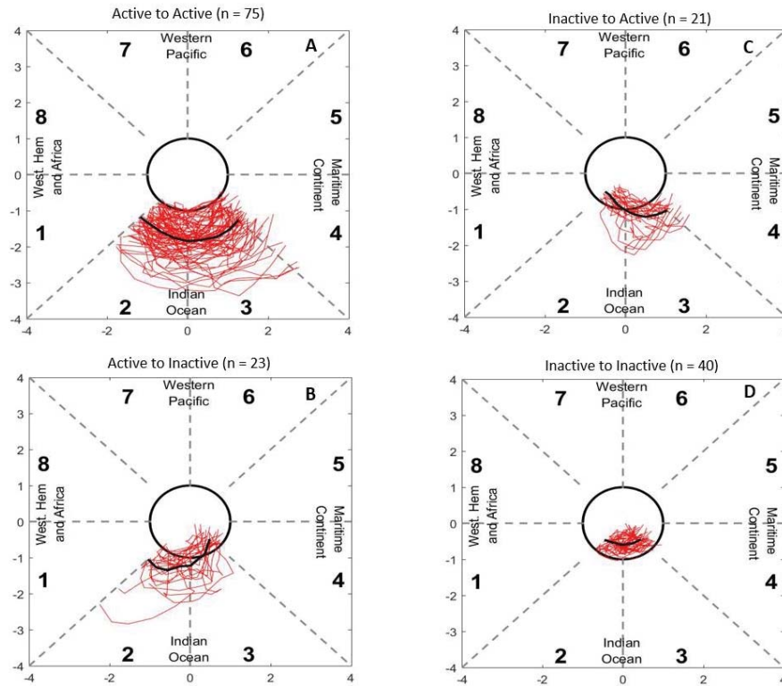
FIGURE 11: As in Figure 6, but for MJO events over the Indian Ocean (MJO phases 2 and 3).
