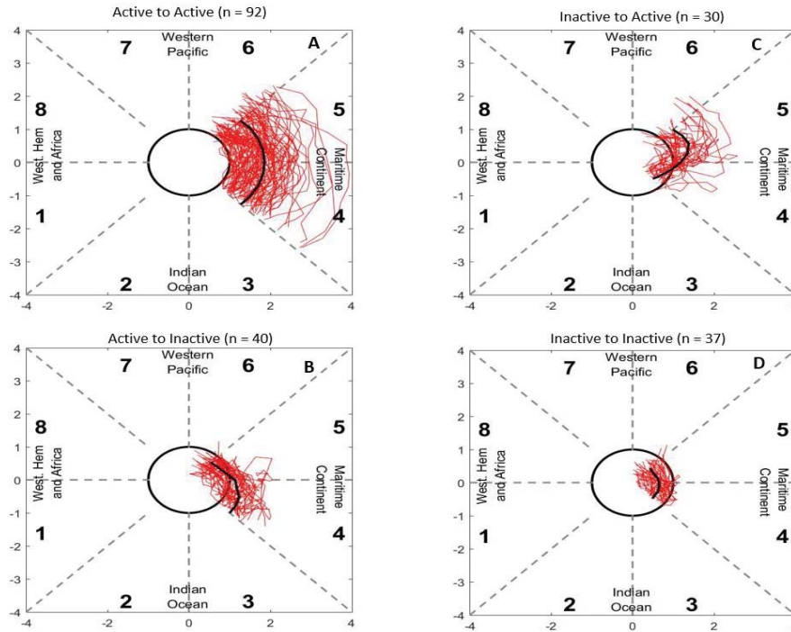
FIGURE 10: MJO events over the Maritime Continent (MJO phases 4 and 5) from 1980-2015, categorized as either active-active (AA, a), active-inactive (AI, b), inactive-active (IA, c), or inactive-inactive (II, d). Black lines denote case averages.
