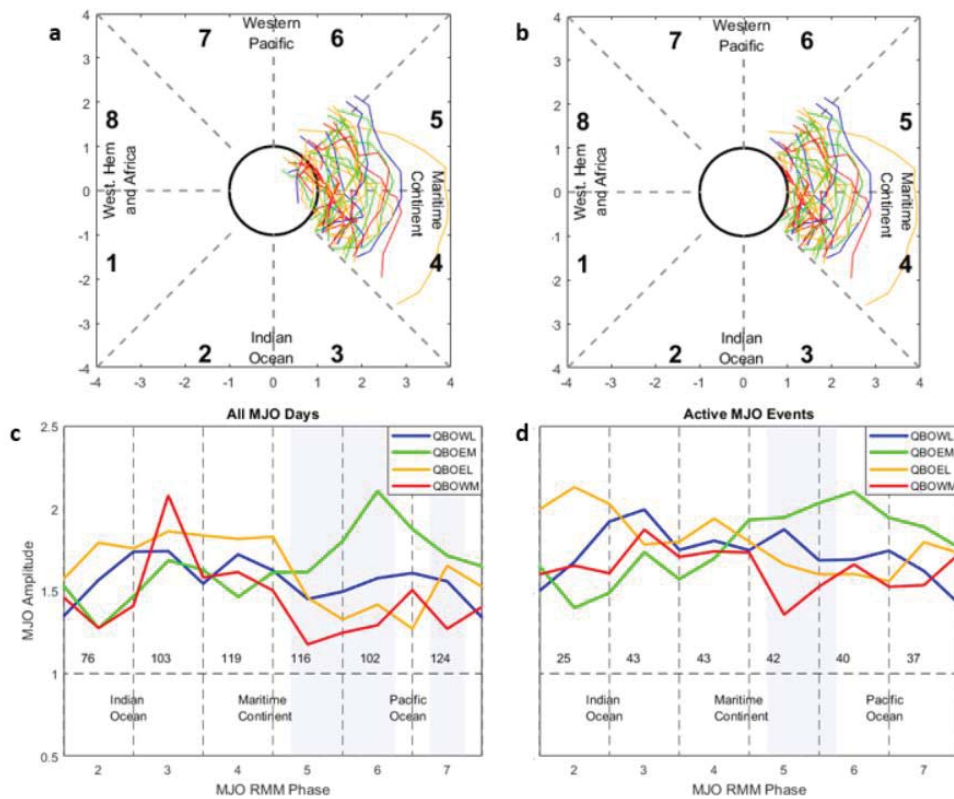
FIGURE 18: Mean RMM amplitudes of each QBO phase pair from MJO phases 2-7 for all MJO days (c) and all active MJO events (d) which entered MJO phase 4 active during boreal winter (DJF) from 1980-2017. Numbers above the dashed line represent the sample size of MJO event datapoints at the center of each phase. Shading denotes MJO phases where RMM amplitudes for QBOEM and QBOWM are statistically significant from one another, as indicated with a Welch's t -test. Phase space diagrams show all MJO event data over the MC included in each analysis (panels a and b, corresponding to panels b and d, respectively).
