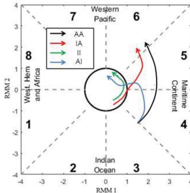
FIGURE 7: Idealized WH04 RMM signatures for each of the four cases of MJO events over the MC.
