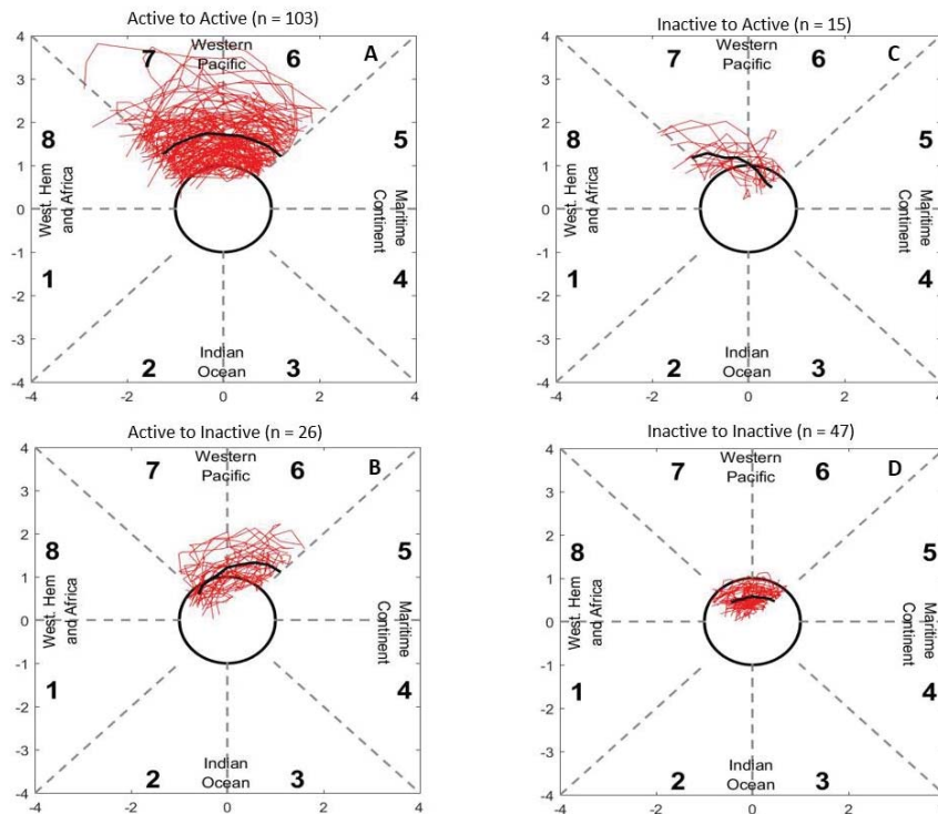
FIGURE 12: As in Figure 6, but for MJO events over the western Pacific Ocean (MJO phases 6 and 7).
