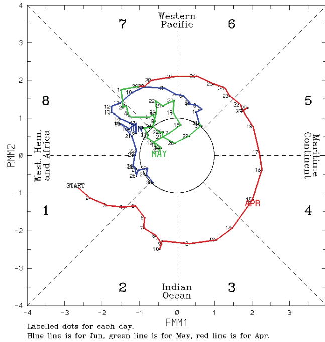
FIGURE 4: RMM Index for April 2009. Quadrant and distance from center for each point correspond to MJO location and strength for that day (Australian BOM website: www.bom.gov.au/climate/MJO ).
