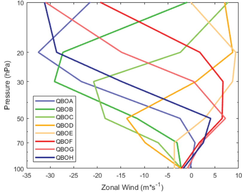
FIGURE 15: Mean ( 10^{\circ}\text{S} - 10^{\circ}\text{N} , 0^{\circ}\text{E} - 360^{\circ}\text{E} ) zonal winds in all months from 1980-2017 for each of the eight QBO phases defined in Fig. 9.
