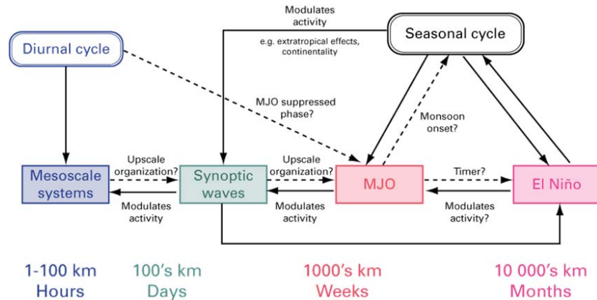
FIGURE 2: Positioning of the MJO in the major atmospheric temporal and spatial scales (adapted from Moncrieff et al. 2007).
