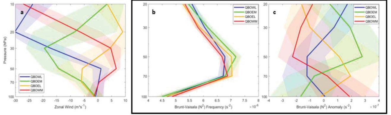
FIGURE 16: Boreal winter zonal wind speeds (a), mean Brunt-Vaisala (BV) frequency values (b) and BV anomalies (c) for each of the four QBO phase pairs from 1980-2017. Values within \pm 1 standard deviation are shaded, and BV anomalies were calculated relative to a 31-day sliding mean to minimize seasonal variability. Note the different y-axis scale between panel a and panels b and c, annotated with a black box surrounding panels b and c.
