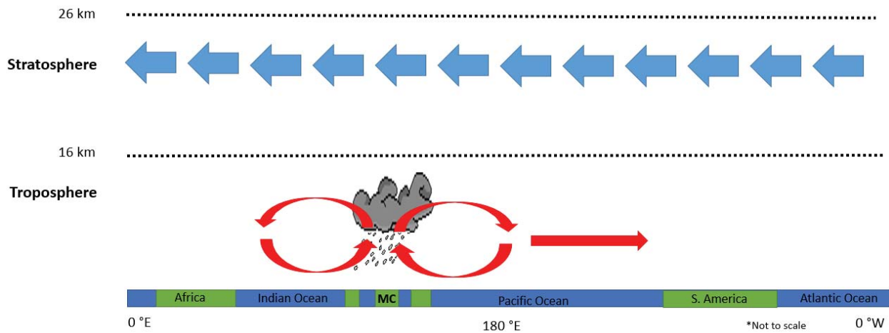
FIGURE 3: Zonal flow associated with the QBO (blue arrows represent flow associated with the easterly QBO) relative to MJO atmospheric circulation and convection (represented by the red arrows and cloud, respectively).
