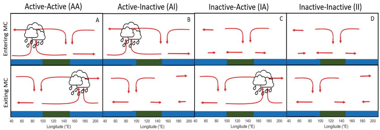
FIGURE 6: Zonal and vertical wind anomalies (red arrows) and resultant convective activity in each of the four cases of MJO events: active-active (AA, A), active-inactive (AI, B), inactive-active (IA, C), and inactive-inactive (II, D). Left and right blue shading represents the Indian and Western Pacific Oceans, respectively, and green shading represents the MC.
