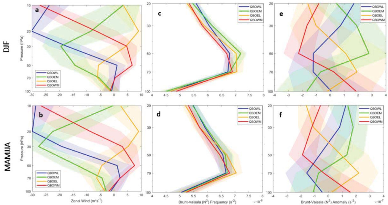
FIGURE 20: Zonal wind speeds (a,b), mean Brunt-Vaisala (BV) frequency values (c,d), and BV anomalies (e,f) for boreal winter (DJF; panels a,c,e) and boreal spring and summer (MAMJJA; panels b,d,f) based on a zonal mean ( 10^{\circ}\text{S} - 10^{\circ}\text{N} ) from 1980-2017. Values within \pm 1 standard deviation are shaded, and BV anomalies were calculated relative to a 31-day sliding mean to minimize seasonal variability. Note the y-axis difference between panels a and b and panels c-f.
