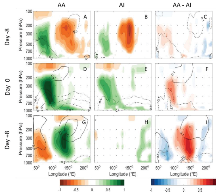
FIGURE 13: Specific humidity (color-filled) and geopotential height (unfilled contours, positive represented by solid lines) standard anomaly contours averaged from 15 °S to 15 °N as the MJO active envelope crosses the western boundary of the MC (100 °E). Anomalies are shown for AA (A, D, G) and AI (B, E, H) MJO events, as well as the differences between the two (C, F, I) at -8 (A-C), 0 (D-F), and 8 (G-I) days relative to MJO active envelope entrance to the MC.
