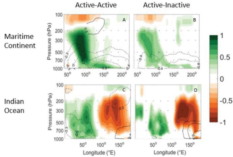
FIGURE 14: As in Fig. 13, but for background atmospheric anomalies during AA (panels a and c) and AI (panels b and d) MJO events over the MC (panels a and b) and Indian Ocean (panels c and d).
