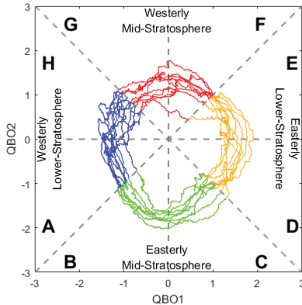
FIGURE 9: Phase space diagram of QBO1 and QBO2 from 1980-2017. Eight phases (separated by dashed lines) divide the QBO zonal winds by direction and altitude of the wind maxima. Distance from the center of the figure corresponds to zonal wind anomaly magnitude. Similar QBO wind profiles are binned into four phase-pair subsets, denoted by color as: blue (Westerly Lower-Stratosphere; QBOWL), green (Easterly Mid-Stratosphere; QBOEM), orange (Easterly Lower-Stratosphere; QBOEL), and red (Westerly Mid-Stratosphere; QBOWM).
