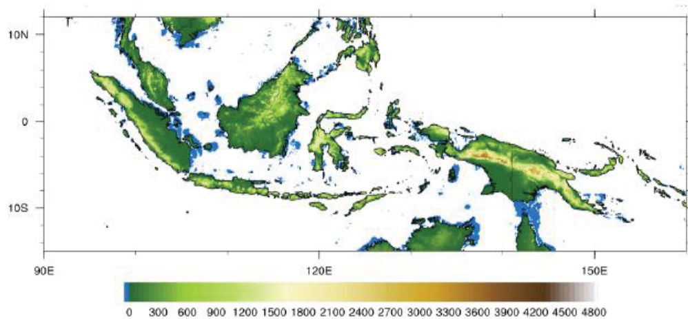
FIGURE 5: Maritime Continent boundaries and topography. Altitude is in meters (Ray et al. 2010)
