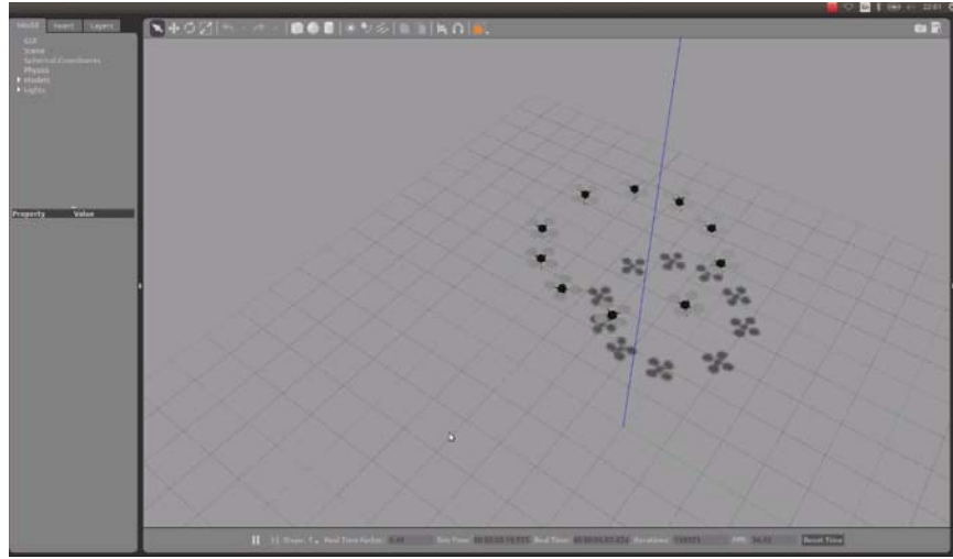
Figure 19: Quadrotors following the limit cycle of the nonlinear parabolic potential swarm in Gazebo. The agents are controlled by ROS, which feeds velocity and position data between Gazebo and Mathematica. Note the similarity to the limit behavior pictured in Figure 6.
