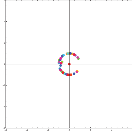
Figure 6: Limit behavior of the parabolic potential model. Agents rotate both ways, but we can decouple the system into all agents rotating in one direction, and all agents rotating in the opposite direction. Both groups should have a stationary center of mass.
