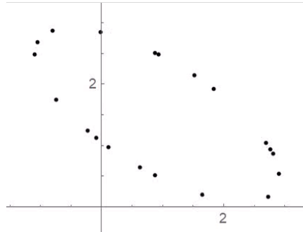
Figure 16: Modifying the parabolic potential model to produce a swarm with oval limit cycles.
