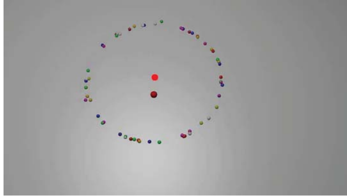
Figure 1: Limit behavior of the parabolic potential model, rendered in Blender. Each small colored dot represents an agent. The dull red dot is the original center of mass. The bright red dot is the current center of mass. The agents rotate in a circle of radius 1, at speed 1, around the center of mass. We believe that this behavior is locally attracting.
