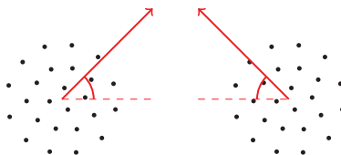
Figure 10: The incident angle of the collision, \theta , which we vary as a parameter.
