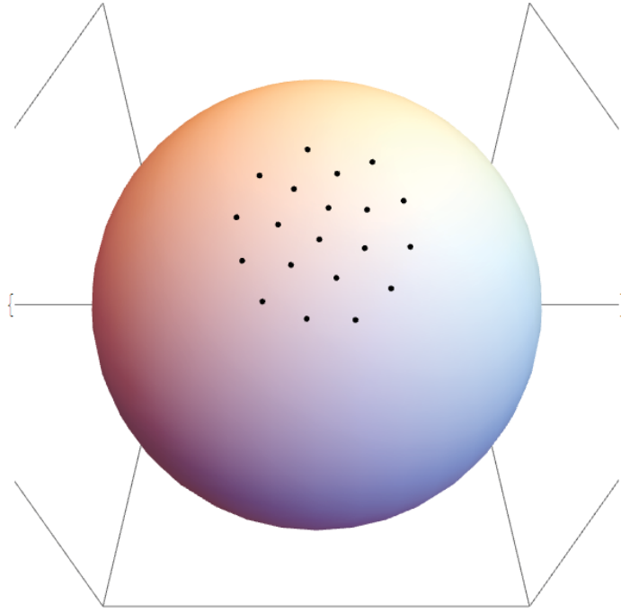
Figure 17: A Morse swarm on a sphere
