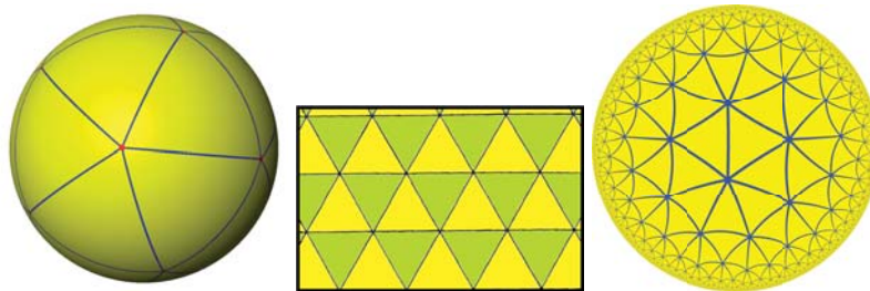
Figure 2: Examples of Riemannian manifolds, each tiled by triangles. From left to right, the sphere, the Euclidean plane, and the Poincaré disk representation of the hyperbolic plane (images from Wikipedia).
