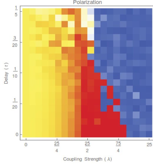
Figure 14: A plot of polarization as a function of \lambda and \tau for fixed \theta . Note that flocking behavior all but disappears above \tau \approx 0.1 .
