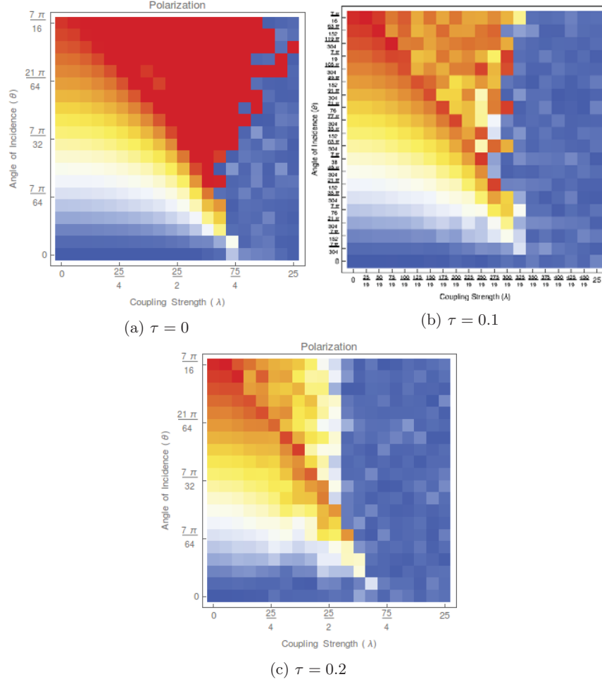
Figure 13: Polarization as a function of \lambda and \theta for 3 distinct values of \tau .
