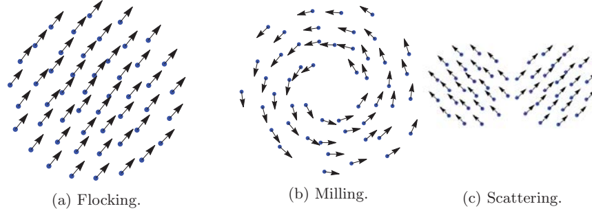
Figure 11: Flocking, milling, and scattering behavior in a Morse swarm.
