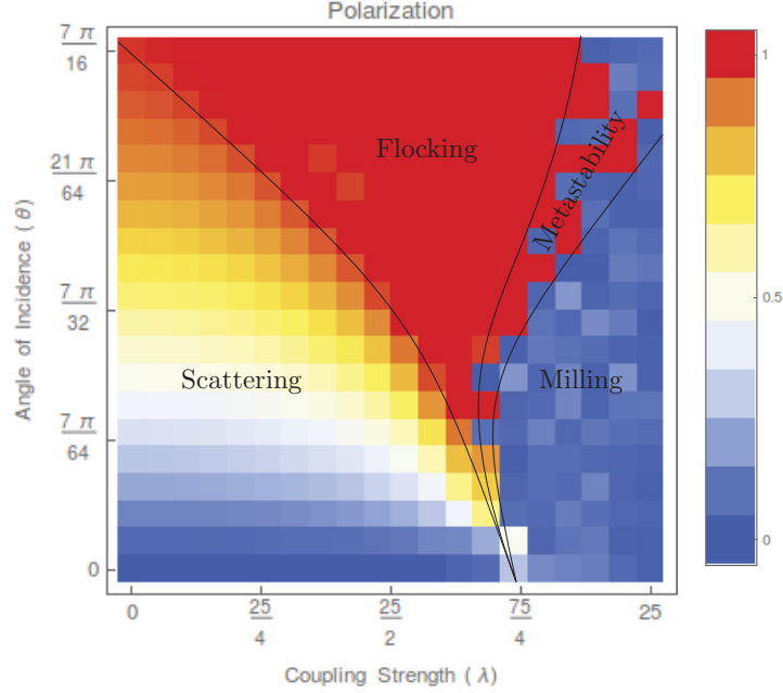
Figure 12: Polarization as a function of \lambda and \theta for an instantaneously-interacting swarm. Note the distinct regions of flocking, milling, scattering, and metastability.
