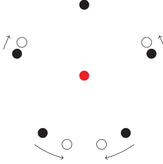
Figure 9: A perturbation which keeps the center of mass constant in a five-agent system.
