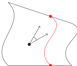
Figure 4: Two vectors on a Riemannian manifold. Their angle and lengths can be calculated using the inner product. A geodesic is shown in red.
