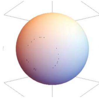
(b) Swarm on sphere
