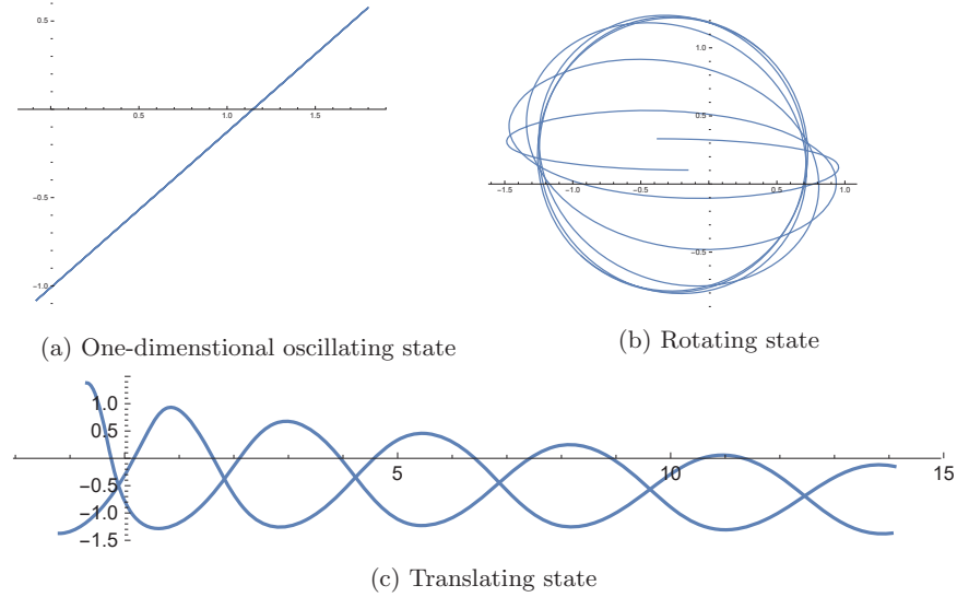
Figure 7: Different behaviors of a swarm of two agents. Different initial conditions produce these behaviors. The plotted lines are the trajectories of two agents on the plane, with varying initial conditions.
