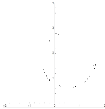
(a) Swarm in hyperbolic half-plane
