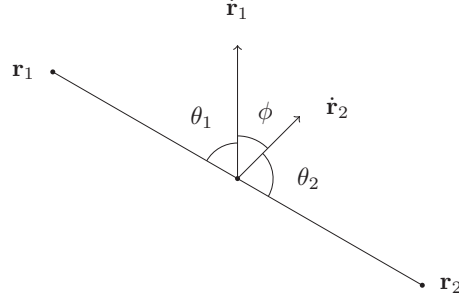
Figure 8: Calculating the angle between \dot{\mathbf{r}}_1 and \dot{\mathbf{r}}_2 .
