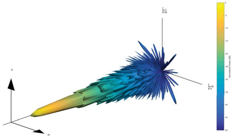
(a) PPA 35 GHz Two Dimensional Representation of Pattern (Zero Elevation Line)
