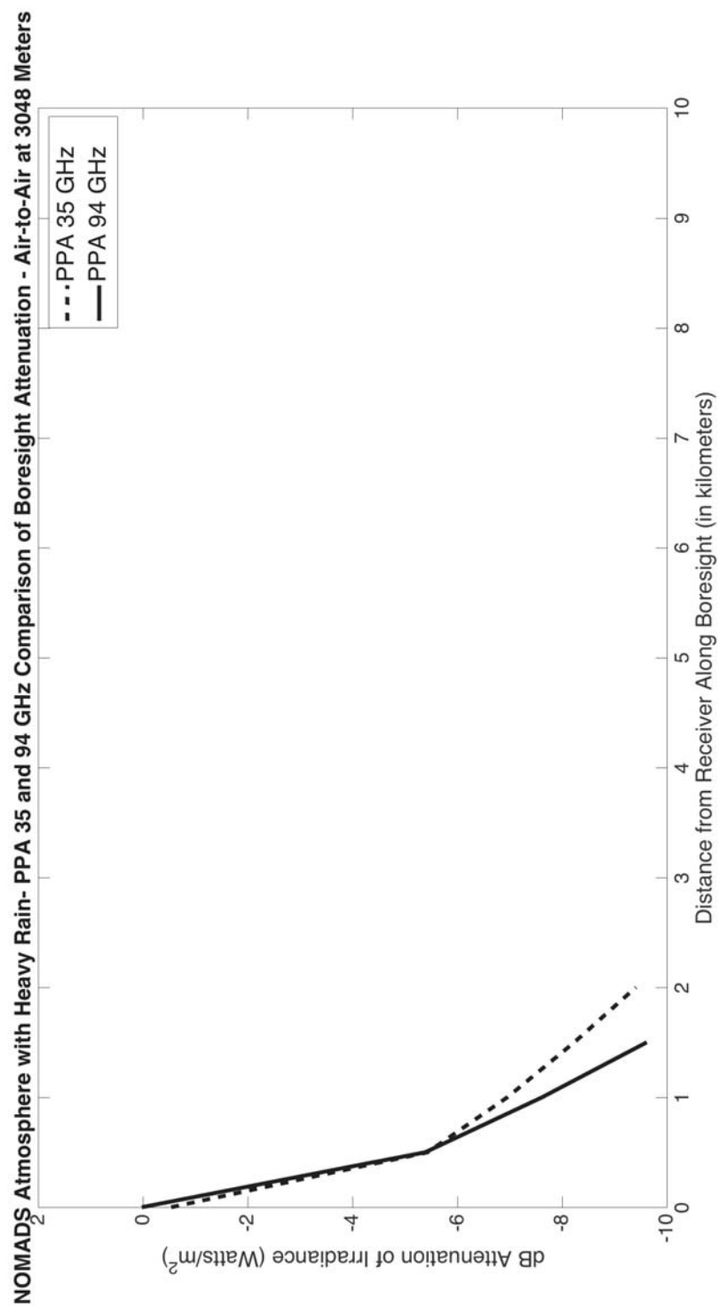
Figure 53. Decibel Attenuation Comparison for Main Beam in Varying Levels of Rain for PPA 94 GHz
