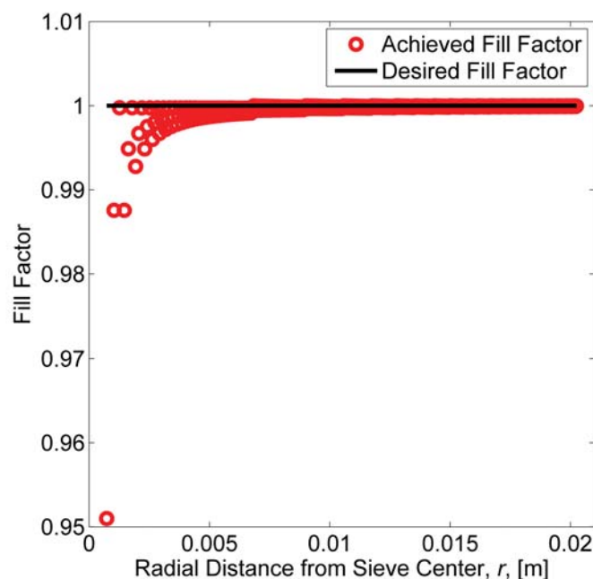
Figure 33. The fill factor is shown as a function of Fresnel zone radius for a controlled unapodized photon sieve. The fill factor remained within a percent of one, except for the innermost zones where there were so few holes that the approximation was poor. This method was used to generate the square and circular photon sieves, which also provided the baselines for the apodized sieves.
