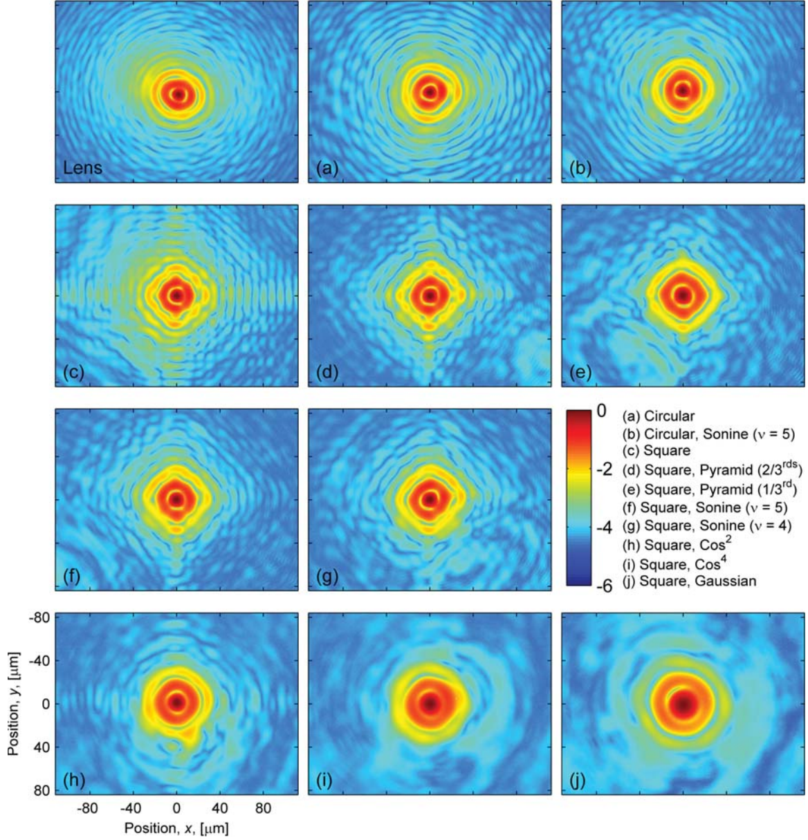
Figure 53. Log 10 colormapped, HDR scaled-and-spliced images of the point spread functions produced by the control lens and the photon sieves. The positions given are in the plane of the PSF (the focal plane). The labels of the colorbar denote the value of the exponent, e.g., “-6” on the colorbar corresponds to a data point with a value at 10^{-6} of the peak value. All images are displayed at the same scale.
