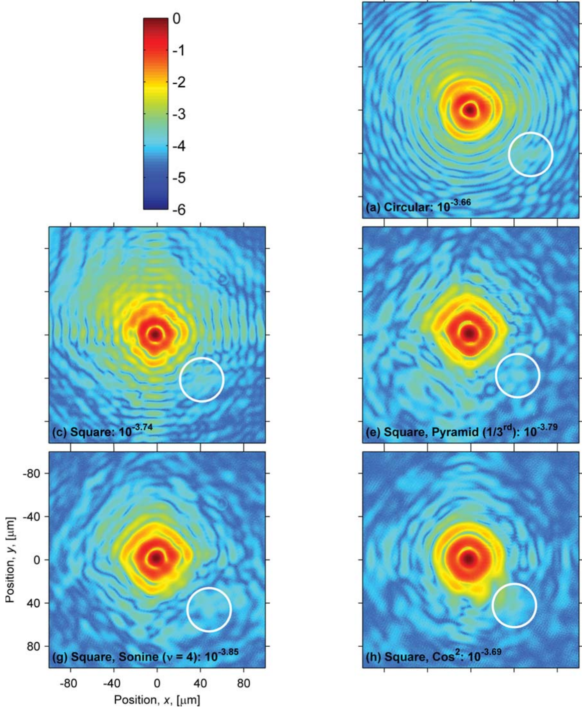
Figure 74. \text{Log}_{10} colormapped, HDR scaled-and-spliced images from the two-beam 10^{-3.5} illumination test. The positions given are in the plane of the PSFs (the focal plane) and all images are displayed at the same scale. The labels of the colorbar denote the value of the exponent, e.g., “-6” on the colorbar corresponds to a data point with a value at 10^{-6} of the peak value. The dim PSF’s peak is shown circled in white in each image.
