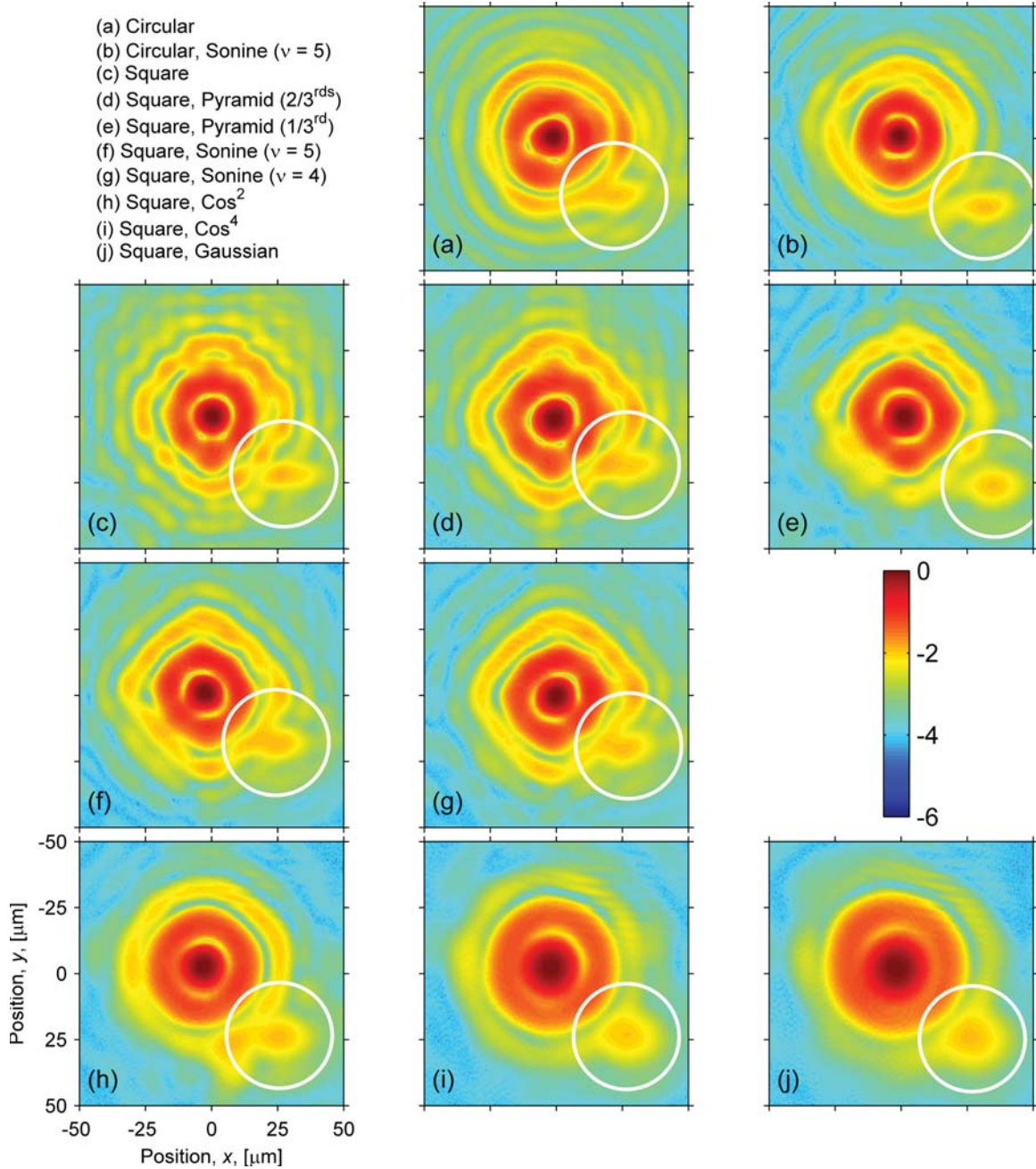
Figure 70. Log 10 colormapped, HDR scaled-and-spliced images from the two-beam illumination test. The positions given are in the plane of the PSFs (the focal plane) and all images are displayed at the same scale. The labels of the colorbar denote the value of the exponent, e.g., “-6” on the colorbar corresponds to a data point with a value at 10^{-6} of the peak value. The power in the dim beam was decreased relative to the power in the bright beam using ND filters until the peak of its PSF was at roughly 10^{-2} of the bright PSF’s peak. The bright PSF’s peak is centered in each image, while the dim PSF’s peak is shown circled in white.
