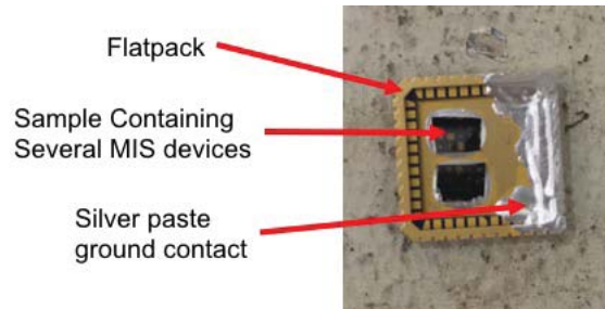
Figure 12. Prepared hBN MIS device sample for measurement and irradiation.
