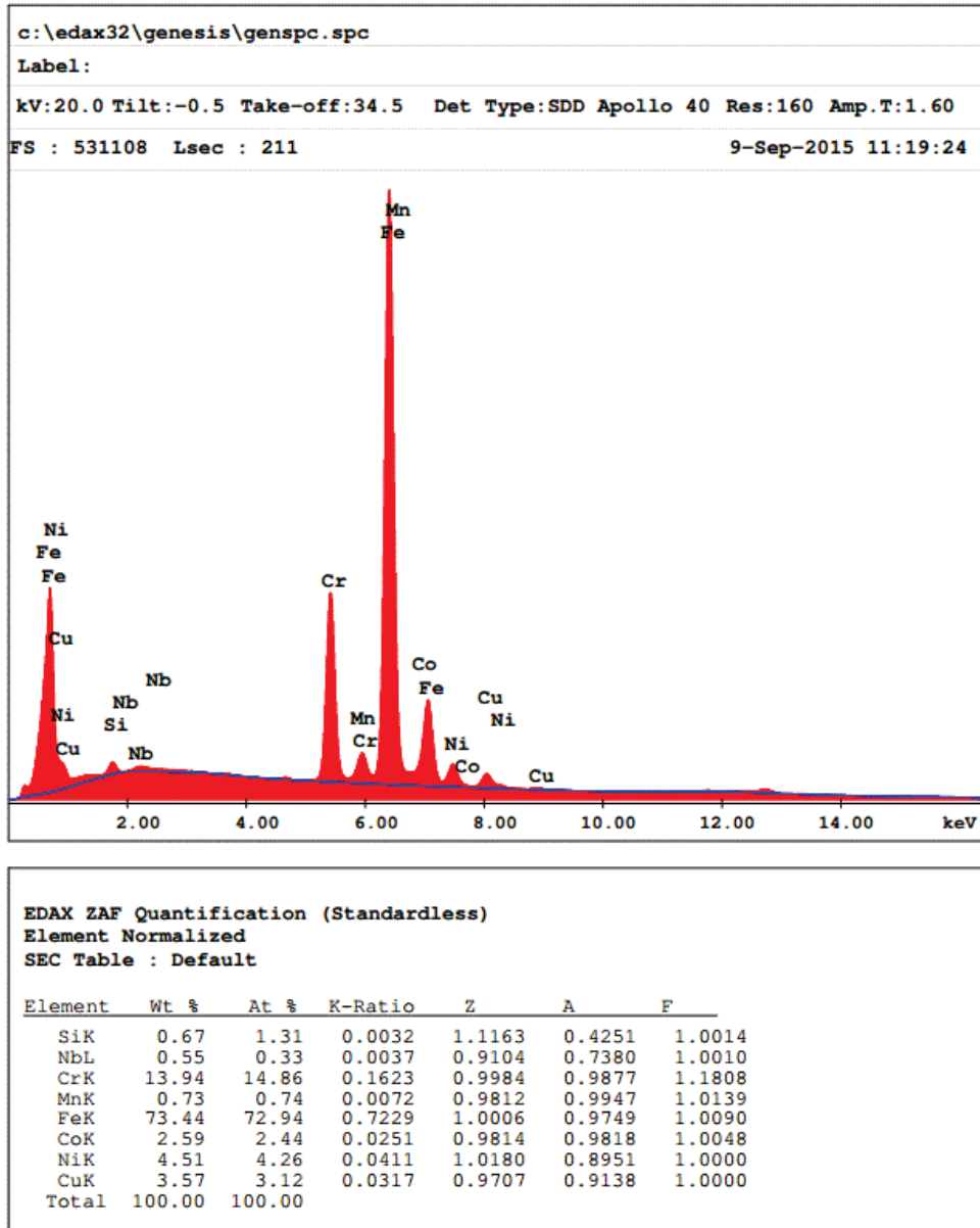
Figure 7. EDS spectrum for Build 3 material
