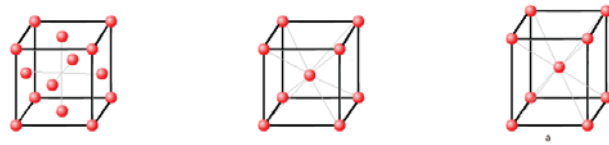
(a) FCC Crystalline Unit Structure (b) BCC Crystalline Unit Structure (c) BCT Crystalline Unit Structure
