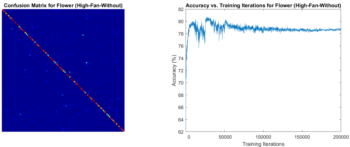
Figure 62. Results from the flower high-fan-without network. Left: The confusion matrix generated by the best model for flower with initialization from the high-fan superset network without flower data. Right: The accuracy on the test set over training.
