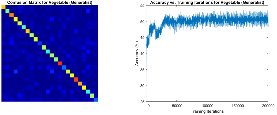
Figure 38. Results from the vegetable generalist network. Left: The confusion matrix generated by the best model for vegetable with initialization from the generalist superset network. Right: The accuracy on the test set over training.
