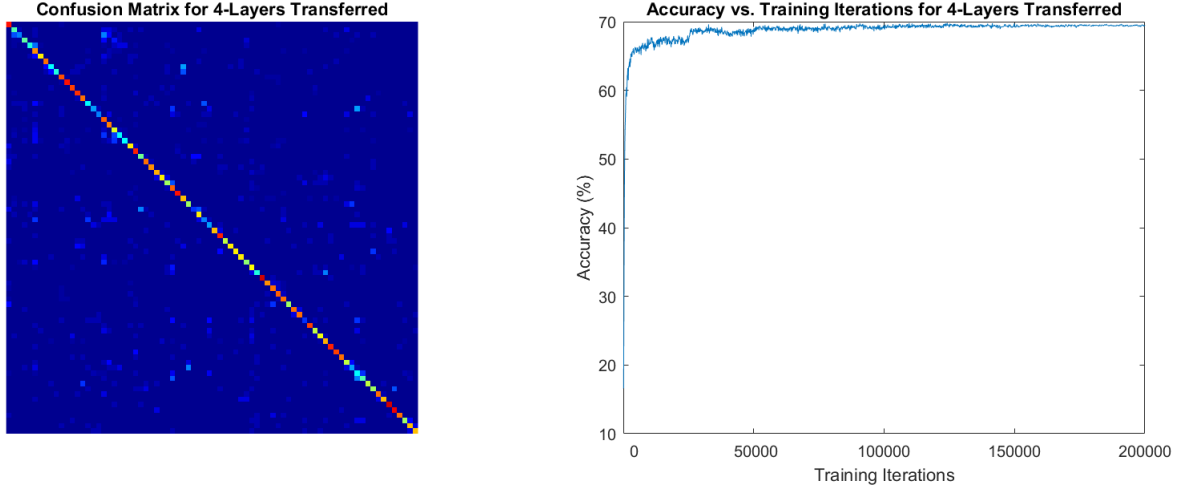
Figure 19. The results of the 4-layer network. Left: The confusion matrix generated by the best model with only 4-layers transferred. Right: The accuracy on the test set over training.
