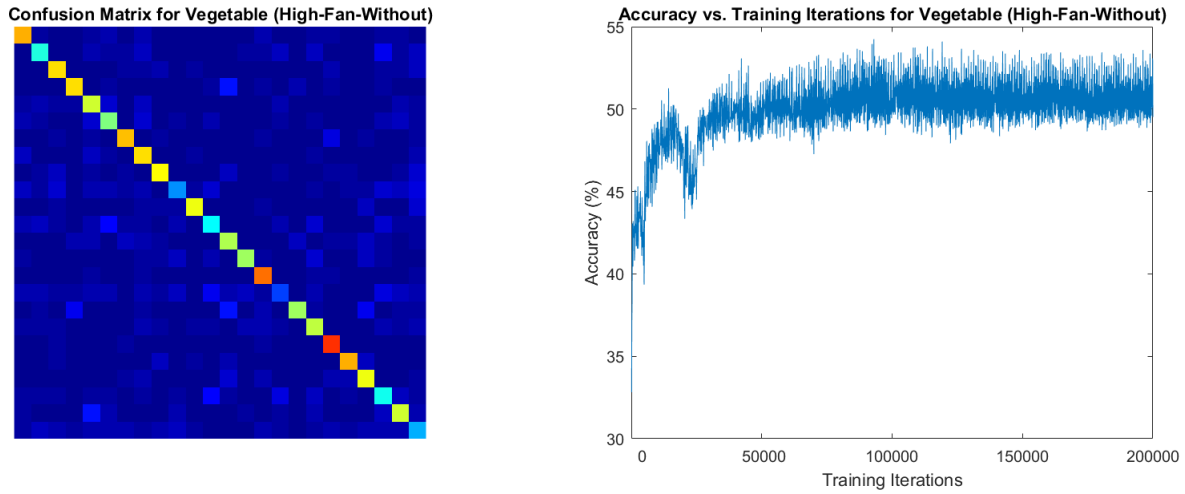
Figure 41. Results from the vegetable high-fan-without network. Left: The confusion matrix generated by the best model for vegetable with initialization from the high-fan superset network without vegetable data. Right: The accuracy on the test set over training.
