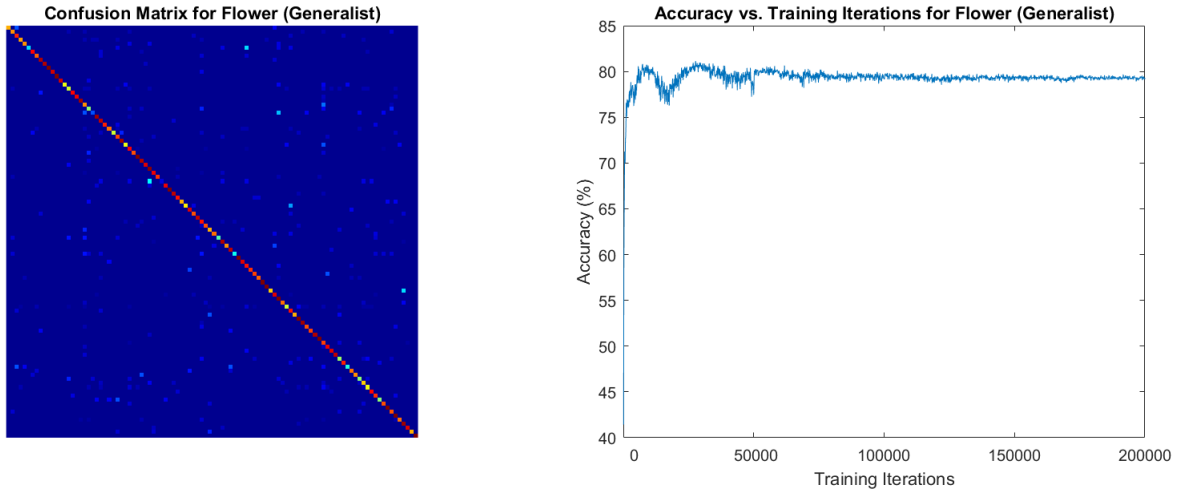
Figure 59. Results from the flower generalist network. Left: The confusion matrix generated by the best model for flower with initialization from the generalist superset network. Right: The accuracy on the test set over training.
