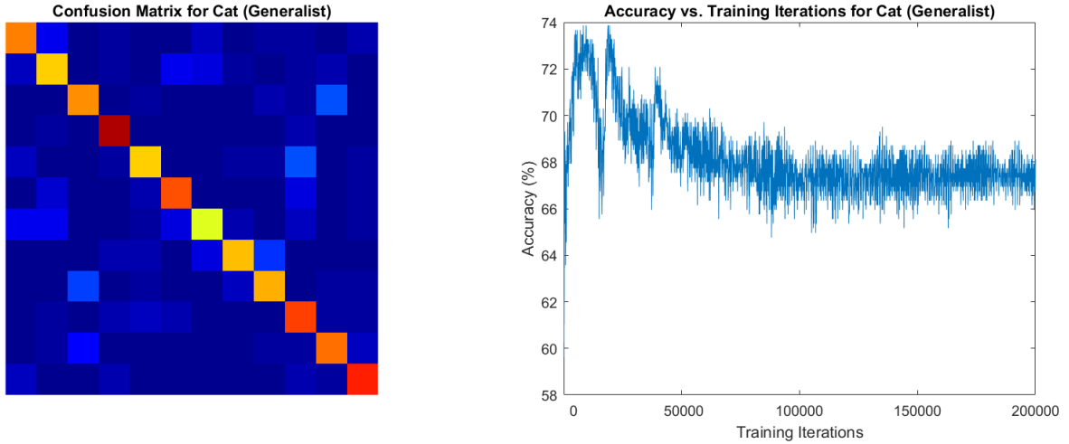
Figure 52. Results from the cat generalist network. Left: The confusion matrix generated by the best model for cat with initialization from the generalist superset network. Right: The accuracy on the test set over training.
