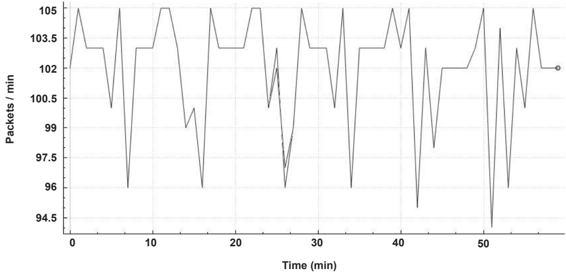
Figure 9. Production Trace and Tcpsreplay Generated Trace transmission rate.
