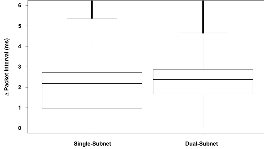
Figure 18. Difference in timing between Production Trace and Generated Trace intervals.
