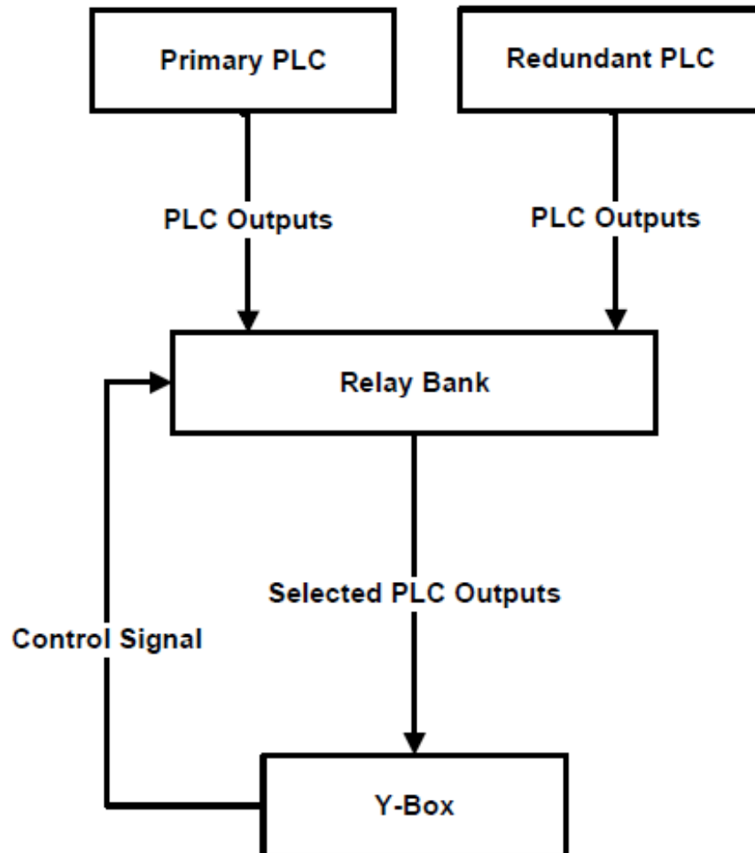
Figure 7. Switchover implementation.
