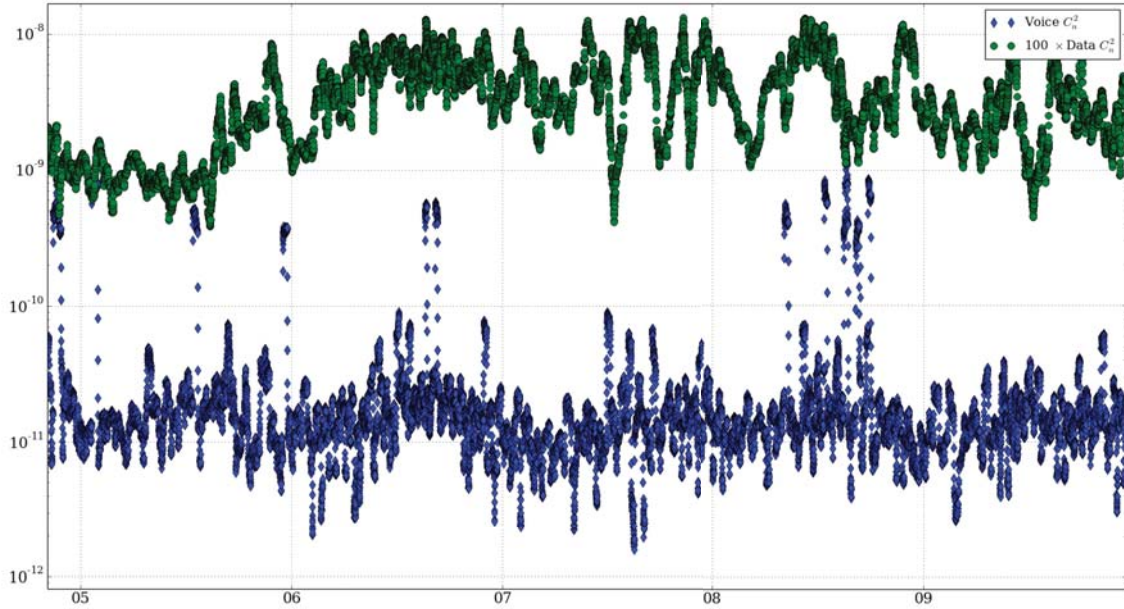
Figure 72. C_n^2 vs time calculated based on 5 days of scintillation in cell phone voice and data power. Data were taken from the third cell phone path, operating on the Verizon ® network. Data C_n^2 are multiplied by 100 in order to provide separation on the plot.
