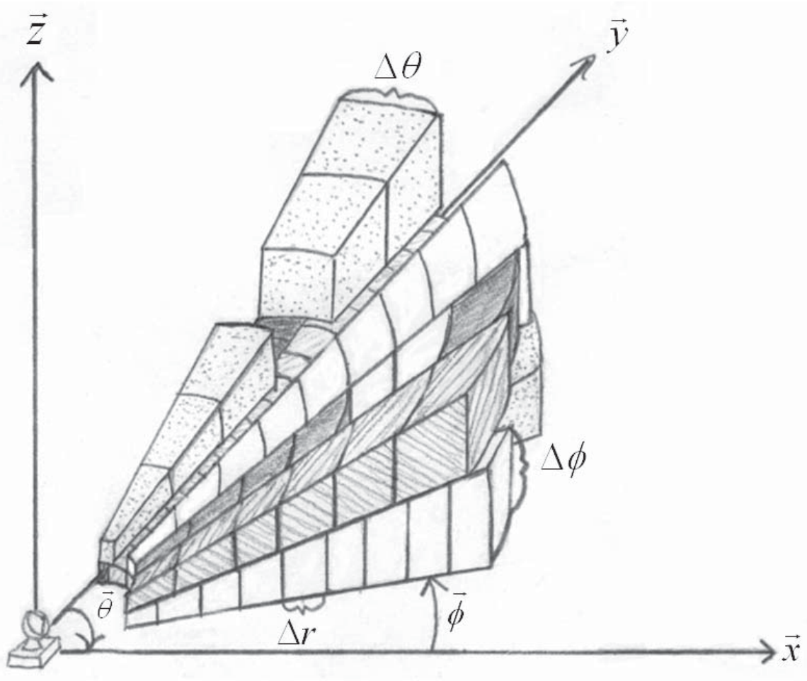
Figure 17. A quadrant of a NEXRAD measurement volume . The volume is divided by elevation angle into sweeps . Each sweep is subdivided by azimuthal angle into rays . Each ray is subdivided by range into individual bins . The spacing of sweeps, rays, and bins is irregular, and there are many structures which are 'empty', having no data.
