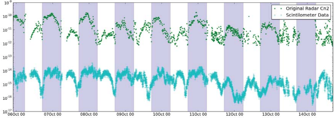
Figure 50. C_n^2 vs time from the UD scintillometer (teal) and NEXRAD radar (green dots) using the method of Doviak [16]. Dark bands indicate nighttime.
