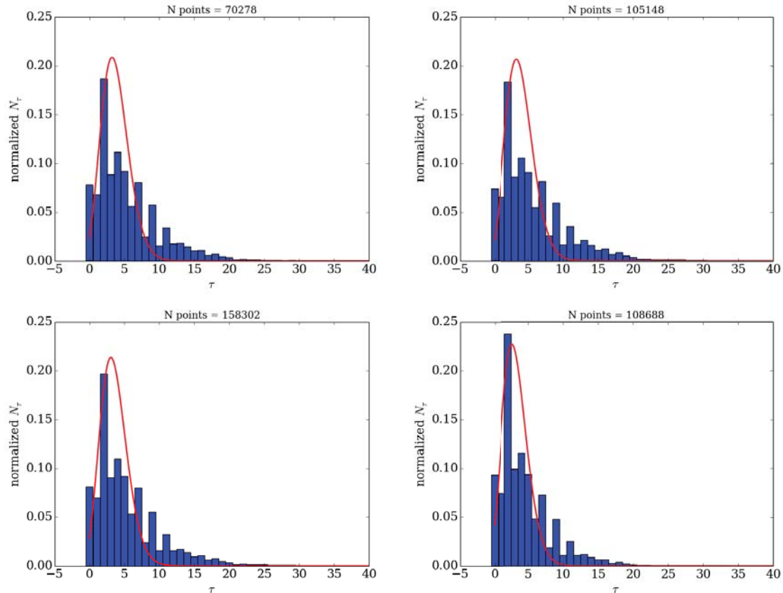
Figure 22. Four distributions of \tau , the temporal spacing (in seconds) between cell phone RSSI samples. Blue bars indicate the histogram of relative number of samples (times > 40s were omitted from the histogram, maximum observed \tau = 200s ). The red line indicates a Poisson process curve fit to the histogram data. Plots are drawn from different months of the year. Clockwise from top left the corresponding months are March, May, July, and September.
