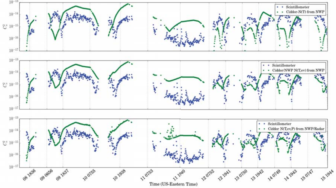
Figure 66. C_n^2 vs time (axis ticks indicate sunrise and sunset) from March 2013. Blue dots indicate scintillometer data from the Dayton site, and green dots are estimates created using NEXRAD and NWP data and the Ciddor N(T) (top), Ciddor N(T, e_v) (middle), and Ciddor N(T, e_v, P) (bottom) methods.
