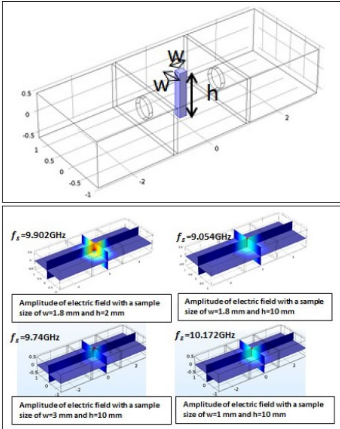
Figure 2.11. Rectangular cavity with sample material (top) used with permission; Rectangular cavity electric field amplitudes (bottom) used with permission [11].
