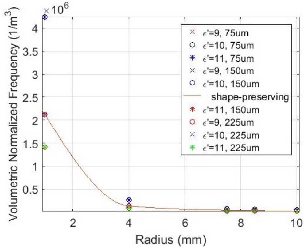
Figure 4.7. Normalized frequency, f'_s , for disk heights of 75 \mu\text{m} , 150 \mu\text{m} , and 225 \mu\text{m} in radius (top); volumetric normalized frequency, f''_s (bottom).
