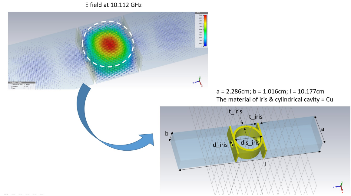
Figure 3.3. Computer Simulation Technology (CST) rendering of empty cylindrical cavity E-field resonating at 10.112 GHz used with permission.
