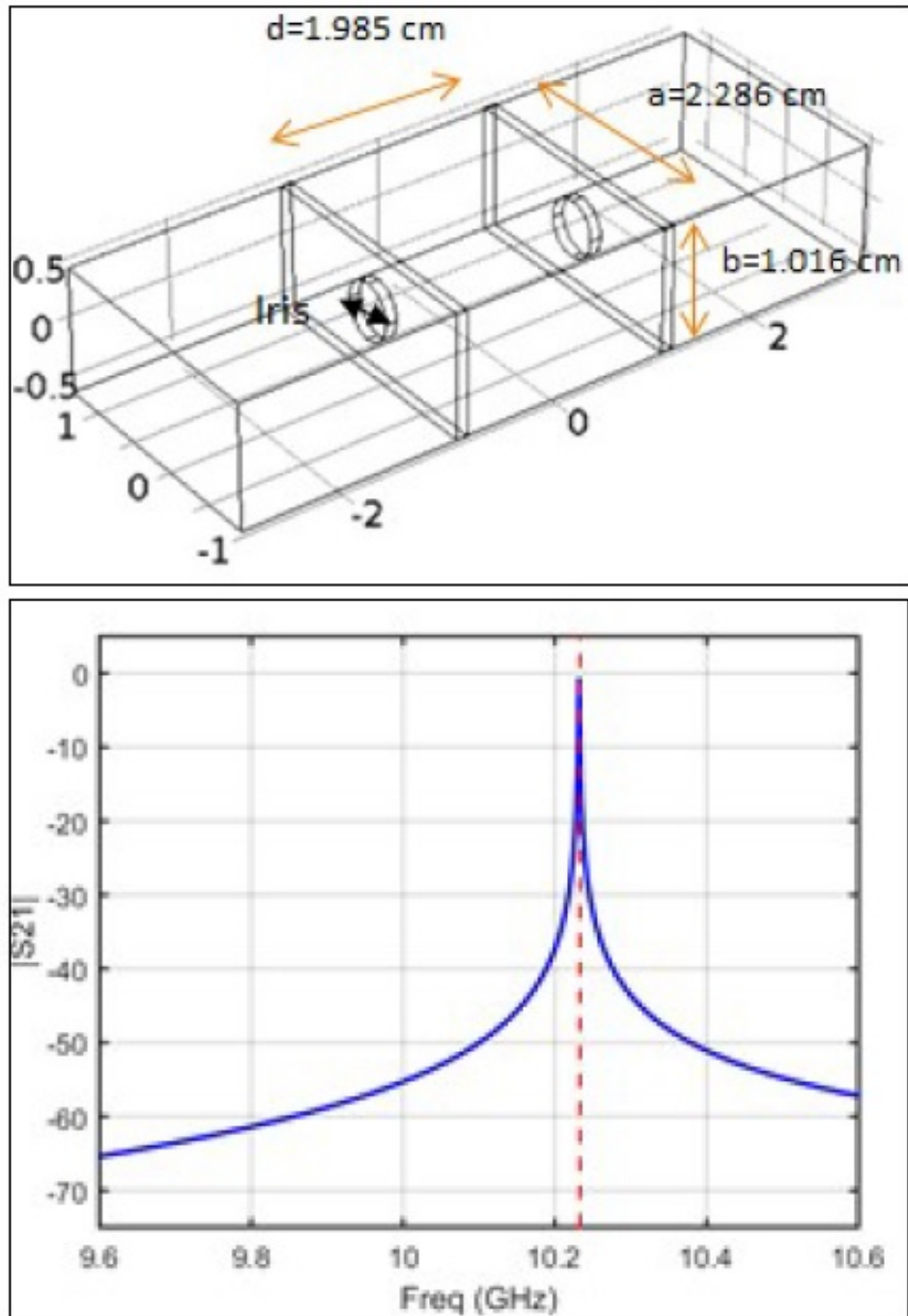
Figure 2.10. AFRL/RYM's rectangular cavity design (top) used with permission; Empty rectangular cavity resonant frequency, 10.23 GHz (bottom) used with permission [11].
