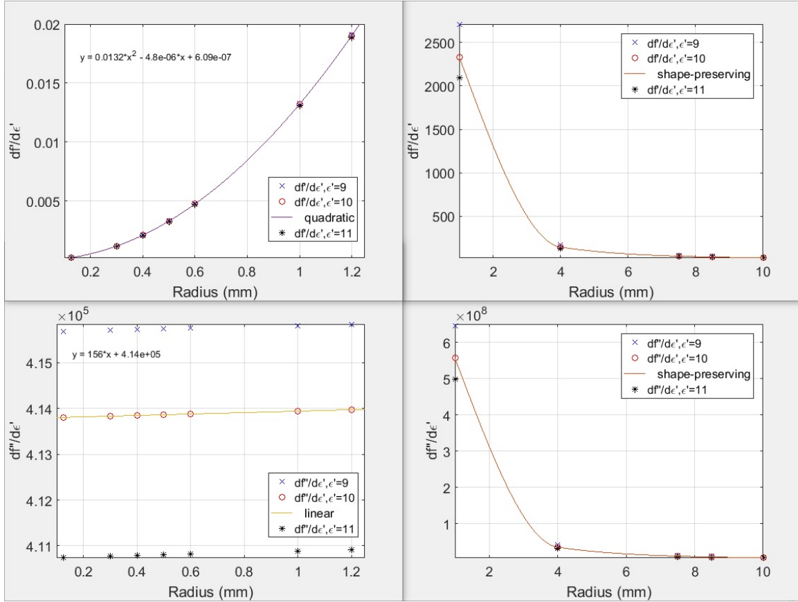
Figure 4.4. Rod sample plots of \frac{df_s'}{d\epsilon'} that shows f_s' is only a function of the radius and \frac{df_s''}{d\epsilon'} shows that f_s'' is a constant (left column); Disk sample plots of \frac{df_s'}{d\epsilon'} and \frac{df_s''}{d\epsilon'} that shows both f_s' and f_s'' are both functions of radius and \epsilon' (right column).
