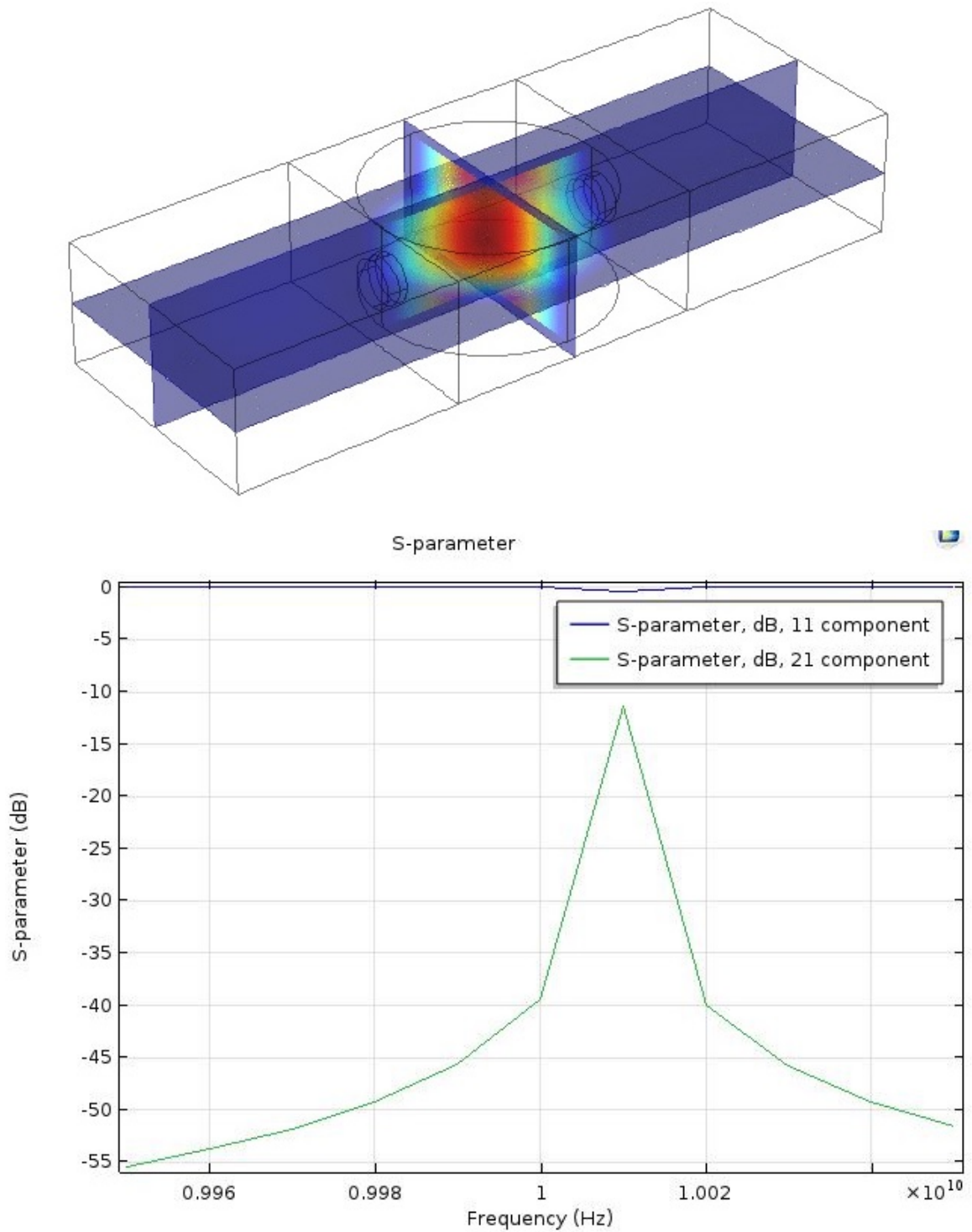
Figure 3.2. COMSOL Multiphysics® model of empty cylindrical cavity E-field (top); empty cylindrical cavity S-parameter (dB) at 10.01 GHz (bottom).
