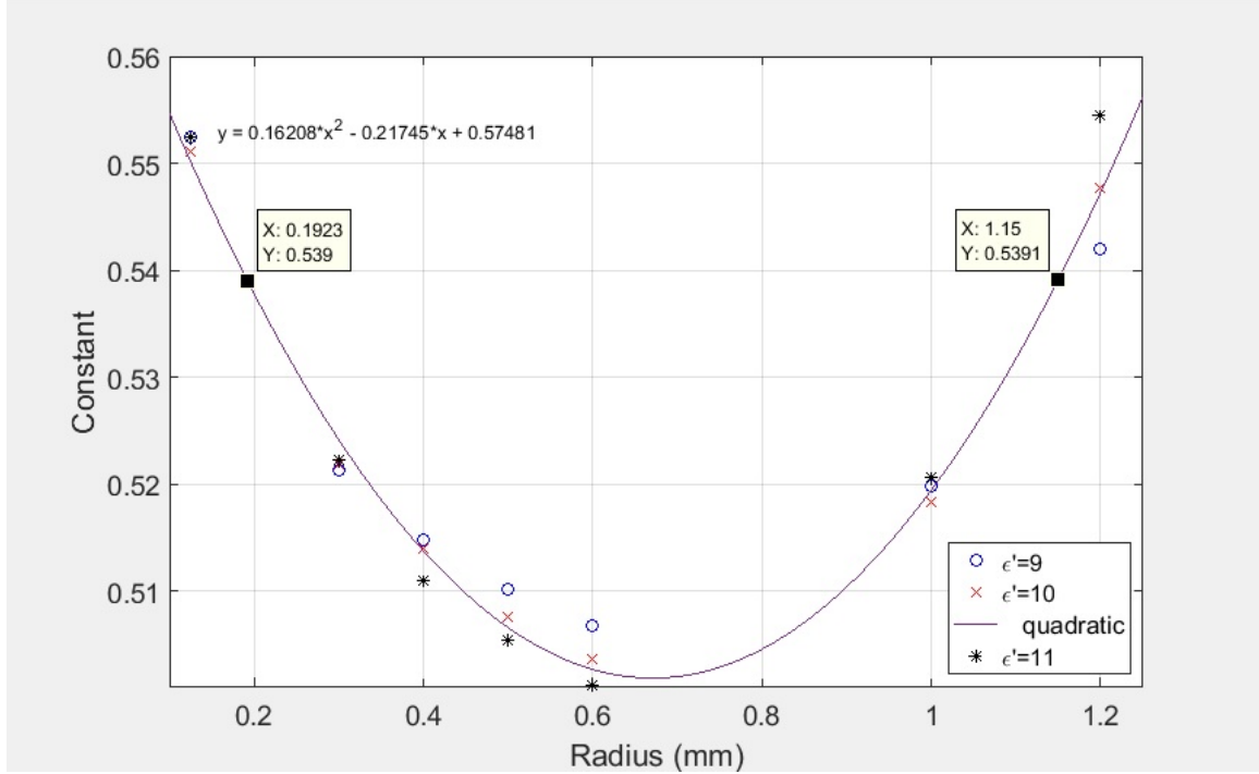
Figure 4.3. Rod sample plot shows quadratic curve of different c_2 constant for each radii that can be used to modify Equation 2.12.
