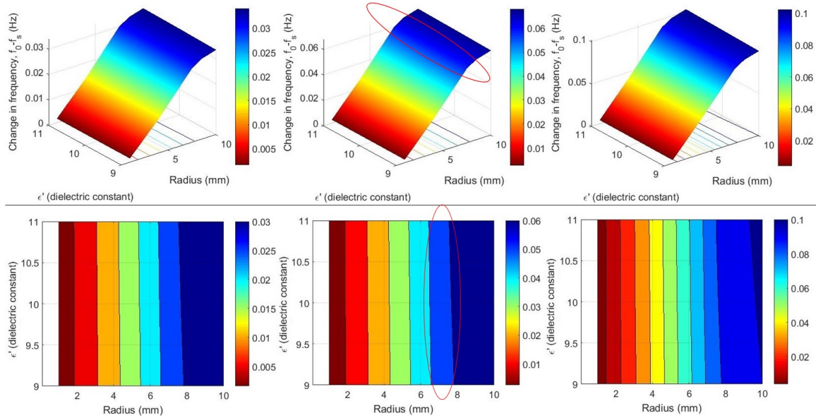
Figure 4.5. Disk sample plots that all show f_0 - f_s is greater at the larger radii: 75\ \mu\text{m} height (left column); 150\ \mu\text{m} height (middle column); 225\ \mu\text{m} height (right column). The color bars represent the change in frequency, or f_0 - f_s , in Hz.
