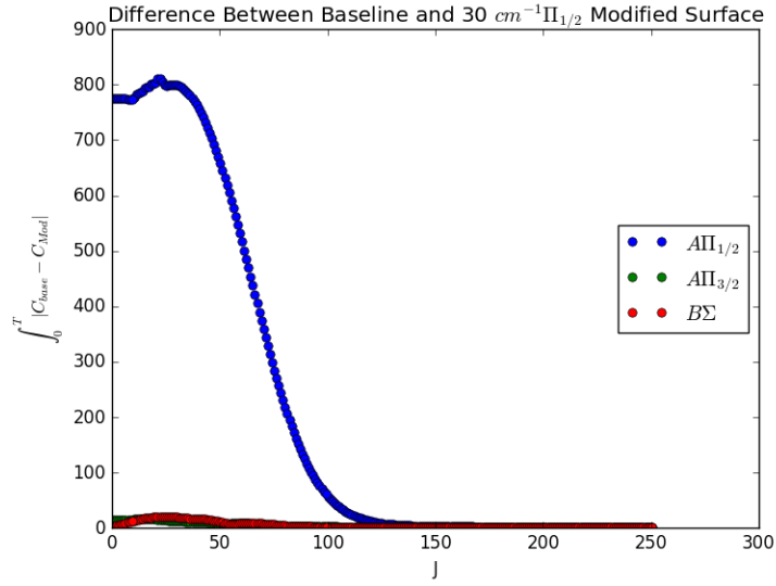
Figure 23. The difference between the baseline correlation and the 30\text{cm}^{-1} modification falls off as J increases and the angular potential dominates.
