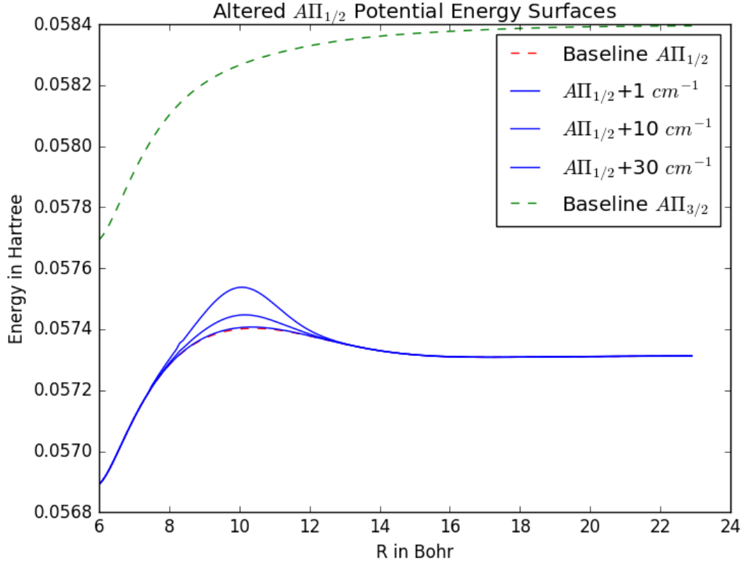
Figure 13. The barrier at the top of the well on the A\Pi_{1/2} surface is increased by 1, 10, and 30 \text{ cm}^{-1} to determine sensitivity of the line broadening and shifting coefficients to changes in the barrier height. The heights were chosen so that surfaces did not cross, insuring the modification did not violate the adiabaticity.
