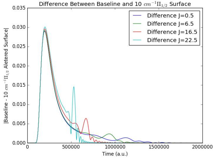
Figure 25. Differences in the correlation function for select J 's show oscillations of different magnitude and duration. These oscillations increase in magnitude as J increases. This peak is caused by the low energy portion of the wave packet spending less time interacting with the potential due to the increased barrier.
