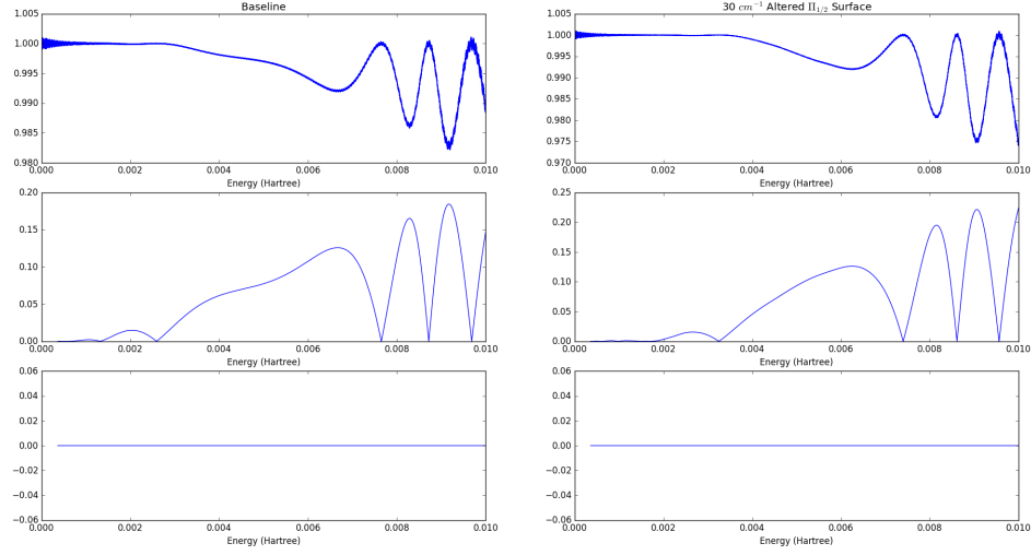
Figure 28. S-matrix elements at J=0.5 for both the baseline and 30\text{ cm}^{-1} altered surface are plotted against each other, with the top plots being the \Pi_{1/2} to \Pi_{1/2} reflection, then working down the \Pi_{1/2} to \Pi_{3/2} transmission, and finally the \Pi_{1/2} to \Sigma_{1/2} transmission.
