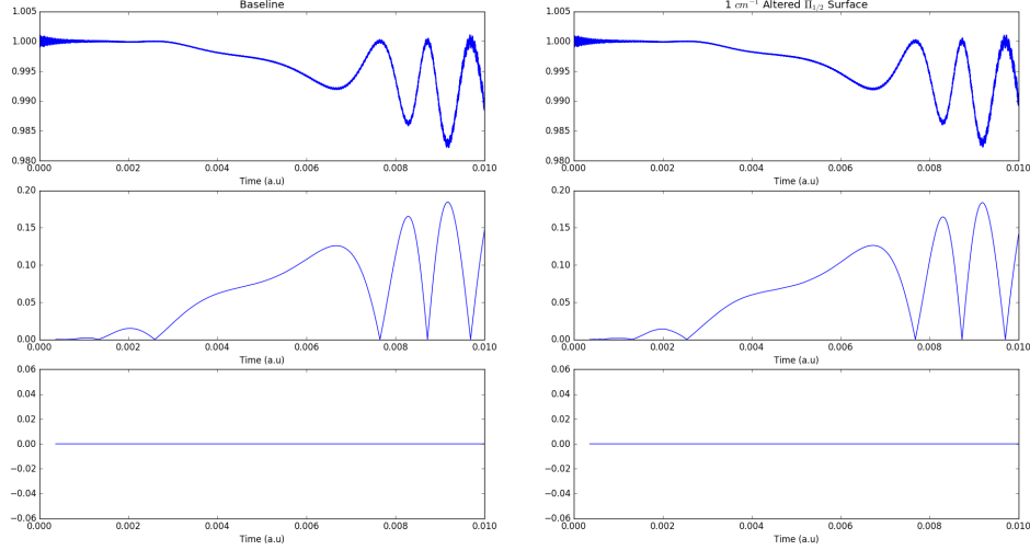
Figure 27. S-matrix elements at J=0.5 for both the baseline and 1 \text{ cm}^{-1} surface are plotted against each other, with the top plots being the \Pi_{1/2} to \Pi_{1/2} reflection, then working down the \Pi_{1/2} to \Pi_{3/2} transmission, and finally the \Pi_{1/2} to \Sigma_{1/2} transmission.
