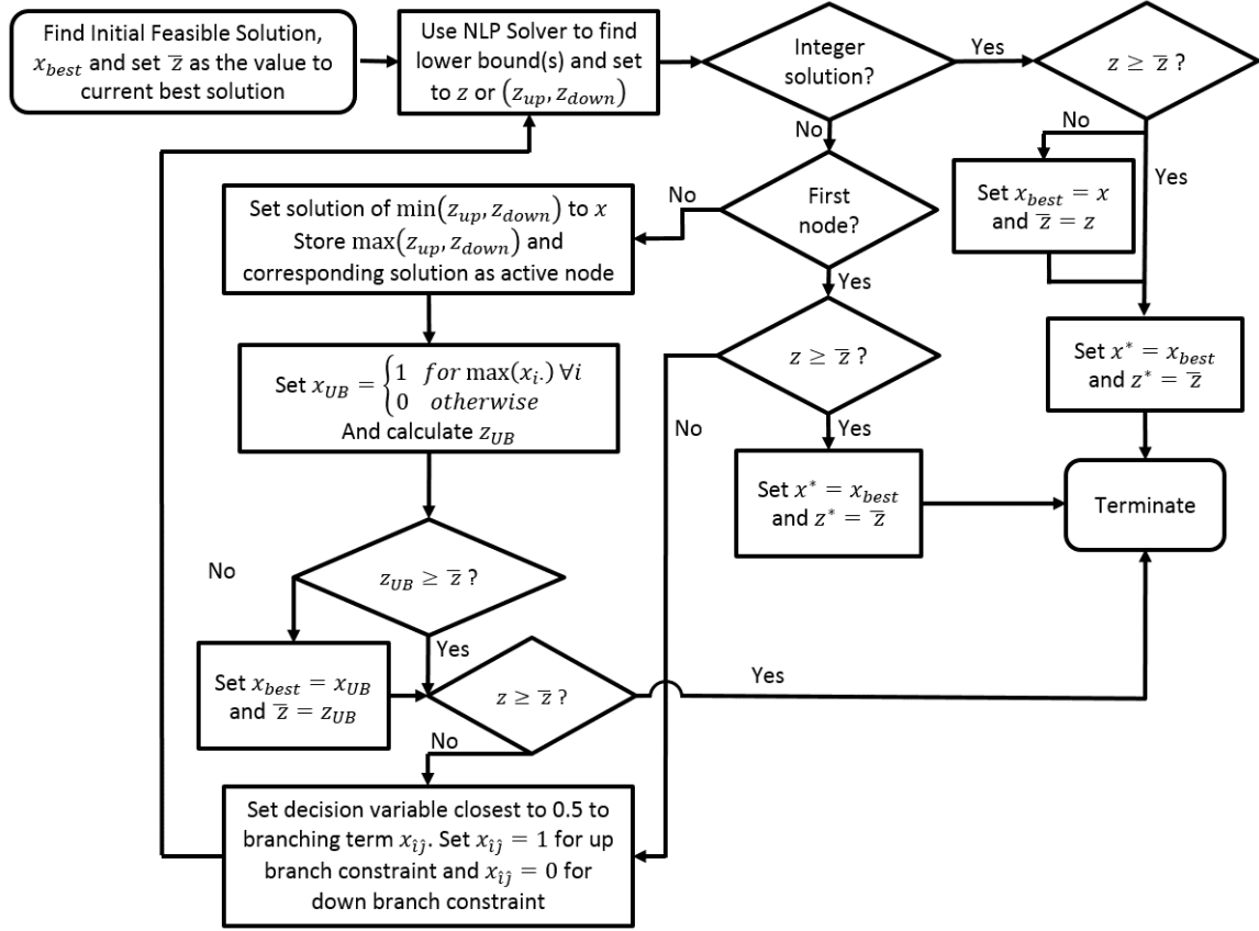
Figure 3. Greedy Branch and Bound Heuristic
