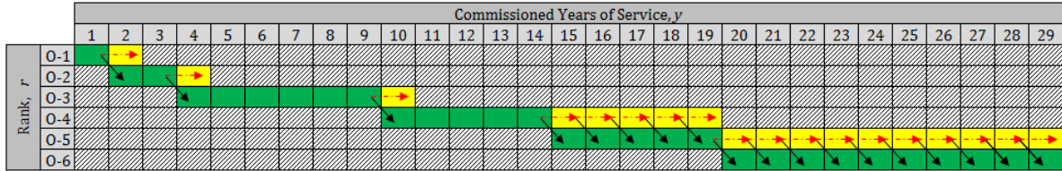
Figure 2. Feasible rank-CYOS combinations
