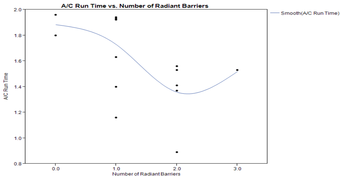
Figure 19: A/C runtime vs. number of radiant barriers
