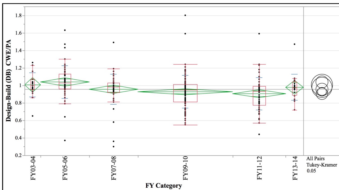
Figure 13 - Design-Bid-Build (DBB) CWE/PA Ratios by FY Category
