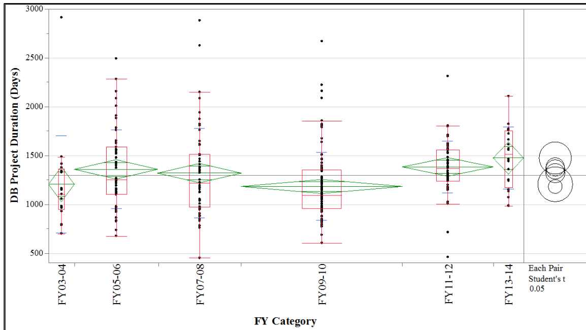
Figure 22 - Design-Build (DB) Project Duration (Days) by FY Category
