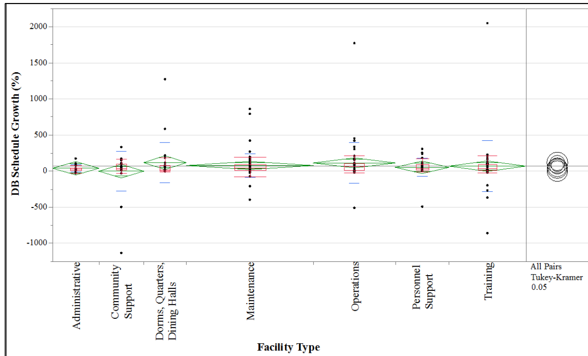
Figure 28 - Design-Build (DB) Schedule Growth (%) by Facility Type
