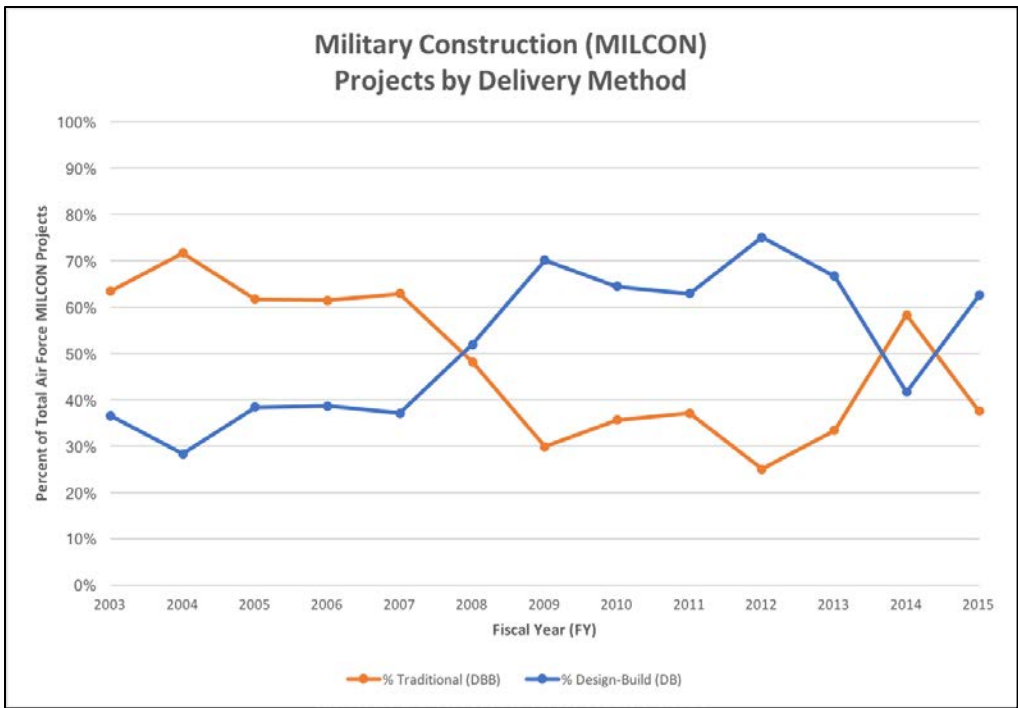
Figure 5 - Air Force MILCON Delivery Method Use (FY 2003-2015)
