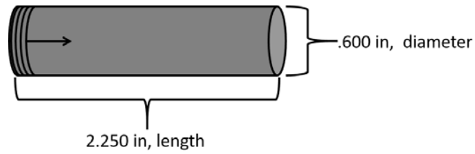
(a) Vertical orientation raw material rod for quasi-static tension testing dimensions
