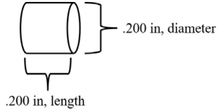
(b) Horizontal orientation raw material rod for SHPB compression testing dimensions
