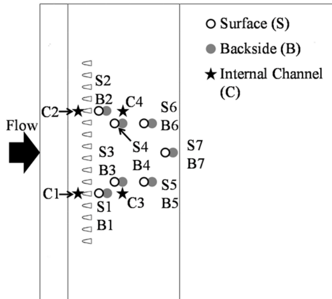
Figure 3-26: Thermocouple instrumentation scheme (modified from Ashby [2])
