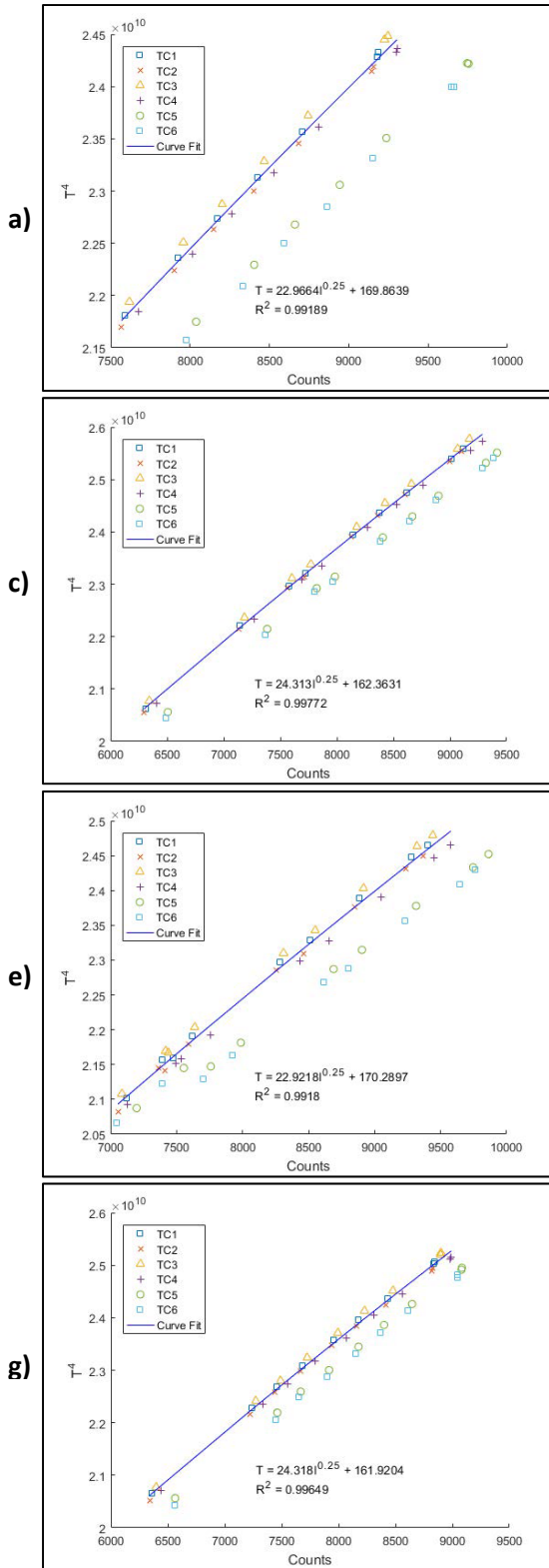
Figure 3-11: Calibration curves and sample IR pictures at equivalent freestream conditions with (a, b) no window, (c, d) sapphire window, (e, f) silicon window, (g, h) tilted sapphire window
