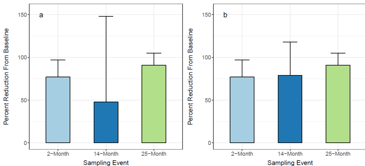
Figure 8. Reduction (%) in Surface Sediment (0-7 cm) Total DDX Concentrations Compared to Baseline: (a) Including All Data, and (b) Excluding Increase of DDX Concentrations at One Station during the 14-month Event.
