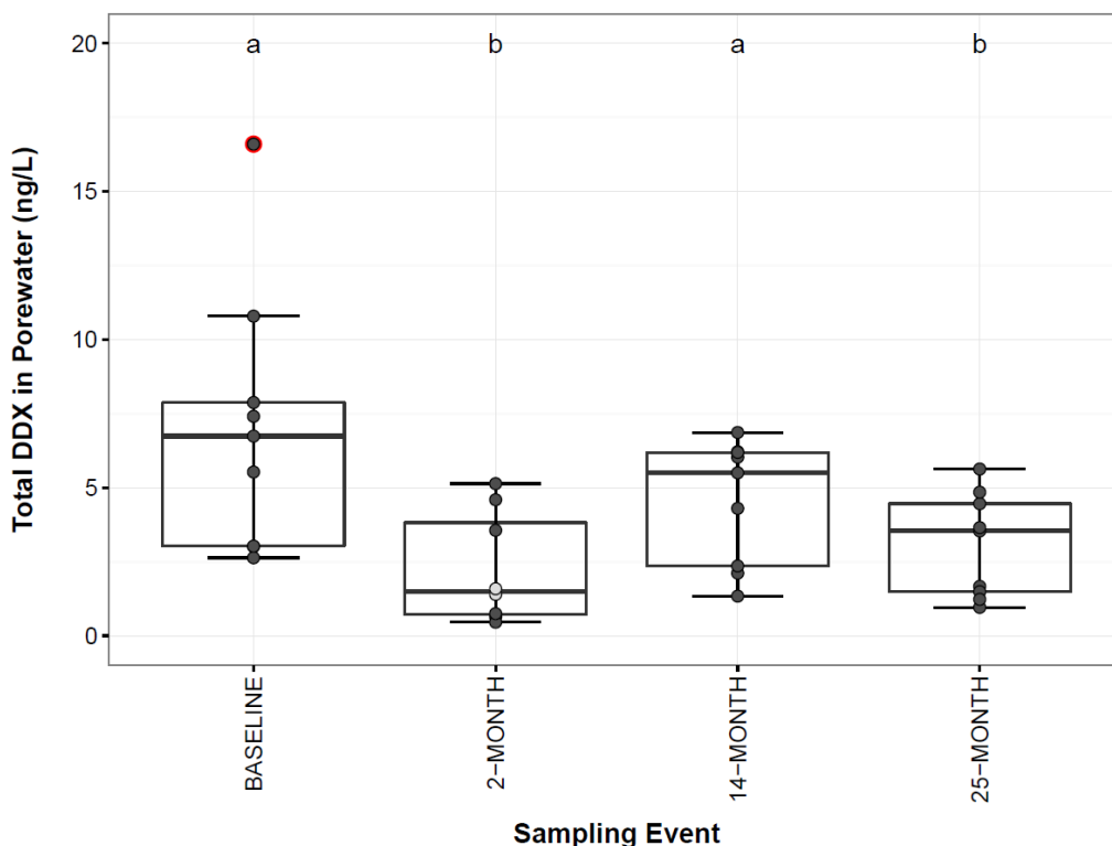
Figure 11. Comparison of Total DDX Concentrations in Surface Porewater (0–2 cm, 2–5 cm, 5–7 cm) for On-cap Stations (2, 3, and 5). Significant differences ( p < 0.05 ) represented as different letters above boxes. Results are plotted as the median (horizontal bar), IQR (limits of boxes are 25th and 75th percentiles), and error bars extend from the IQR to the lowest value within 1.5 * IQR . Data beyond the end of the whiskers are outliers and plotted with a red outline (as specified by Tukey). Notes: Stations 1 and 4 do not have baseline results and were excluded from this graph. Two samples were not detected during the 2-month event and are plotted as grey points.
