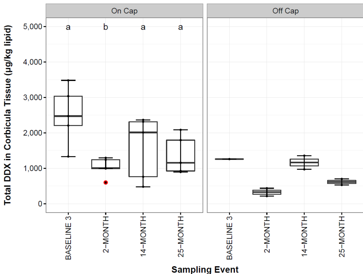
Figure 10. Concentrations of Total DDX in C. fluminea Tissue (µg/kg lipid) for All Available On- and Off Cap Stations. Significant differences ( p < 0.05 ) represented as different letters above boxes. Results are plotted as the median (horizontal bar), IQR (limits of boxes are 25th and 75th percentiles), and error bars extend from the IQR to the lowest value within 1.5 * IQR . Data beyond the end of the whiskers are outliers and plotted as red points (as specified by Tukey).
