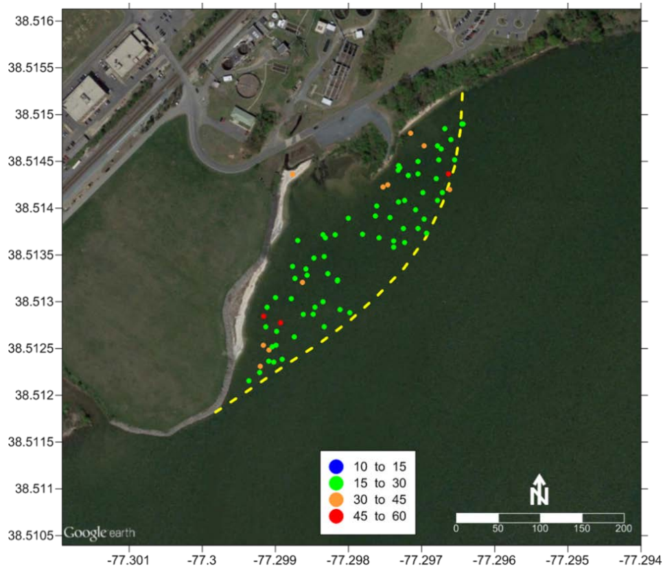
Figure 5. Results for Cap Thickness Measurements Collected by the Site Contractor Immediately Following Construction of the Cap in 2014 (units are in cm).
