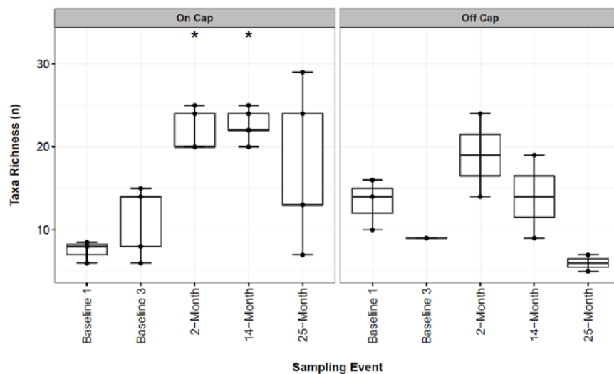
Figure 13. Taxa Richness from the Benthic Community Census, Separated by Stations On and Off the Cap Footprint. Significant differences ( p < 0.05 ) from either baseline event represented as a star (*) above box. Results are plotted as the median (horizontal bar), IQR (limits of boxes are 25th and 75th percentiles), and error bars extend from the IQR to the lowest value within 1.5 * \text{IQR} . Data beyond the end of the whiskers are outliers and plotted as red points (as specified by Tukey).
