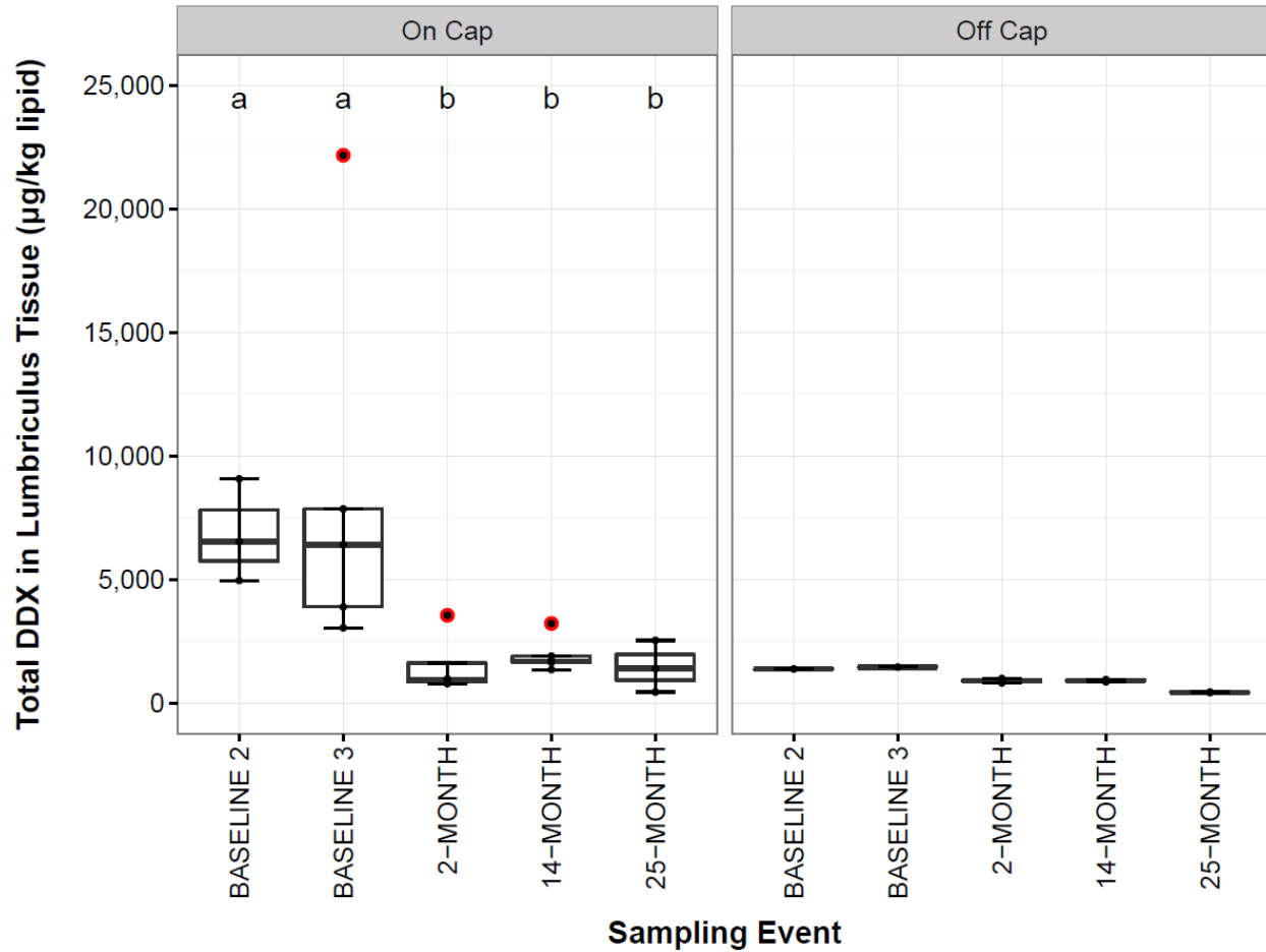
Figure 9. Concentration of Total DDX in L. variegatus Tissue (µg/kg lipid) for All Available On- and Off Cap Stations. Significant differences ( p < 0.05 ) represented as different letters above boxes. Results are plotted as the median (horizontal bar), IQR (limits of boxes are 25th and 75th percentiles), and error bars extend from the IQR to the lowest value within 1.5 * IQR . Data beyond the end of the whiskers are outliers and plotted as red points (as specified by Tukey).
