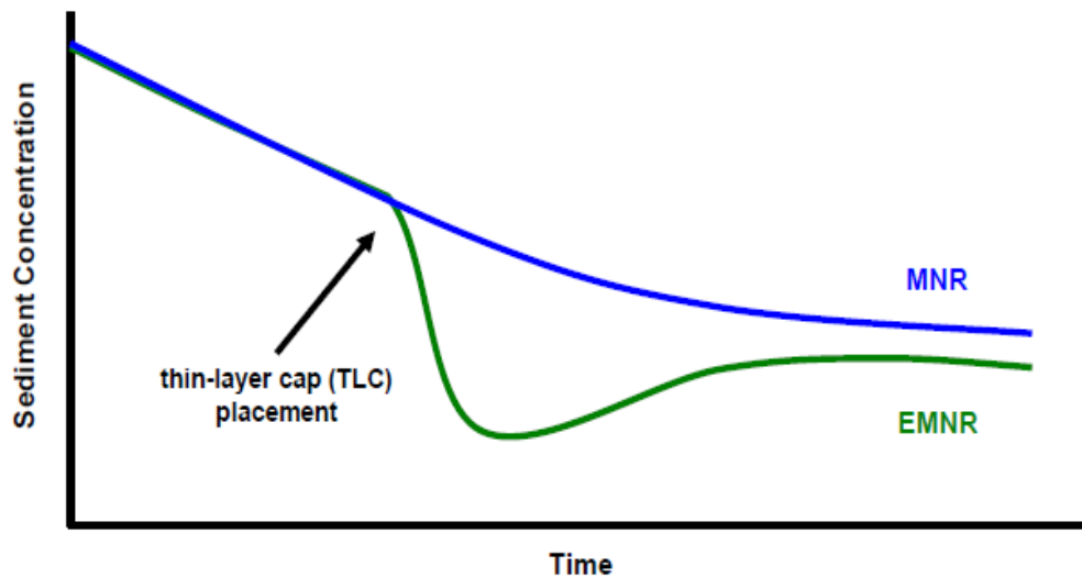
Figure 1. Hypothetical Relationship between Chemical Concentrations in Surface Sediment and Temporal Evolution of System Recovery under MNR and EMNR.
