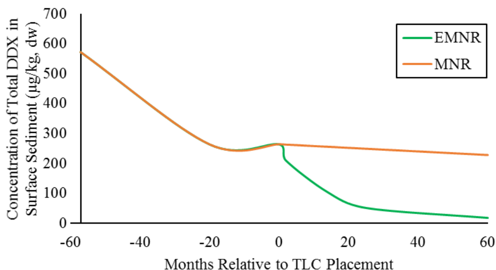
Figure 17. Illustration of EMNR and MNR Performance Relative to Total Sediment DDX Concentrations.
