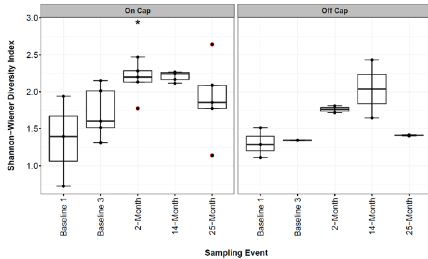
Figure 14. Shannon-Wiener Diversity Index from the Benthic Community Census, Separated by Stations On and Off the Cap Footprint. Significant differences ( p < 0.05 ) from either baseline event represented as a star (*) above box. Results for 2-month event are significantly greater than baseline 1 but not baseline 3. Results are plotted as the median (horizontal bar), IQR (limits of boxes are 25th and 75th percentiles), and error bars extend from the IQR to the lowest value within 1.5 * \text{IQR} . Data beyond the end of the whiskers are outliers and plotted as red points (as specified by Tukey).
