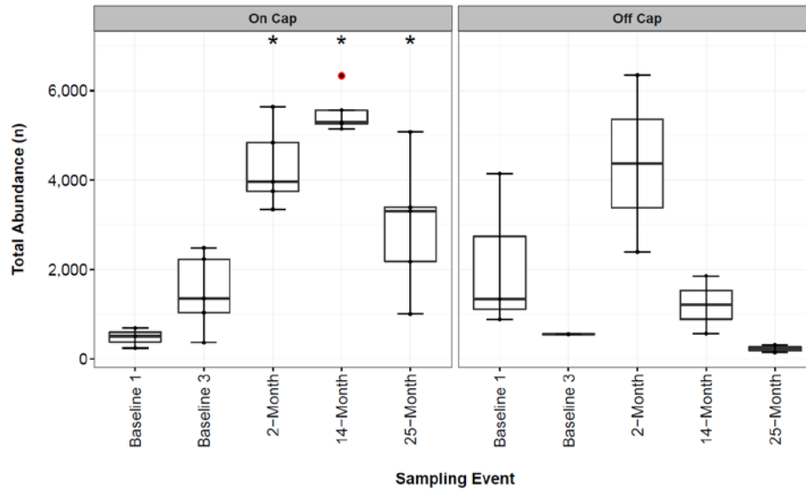
Figure 12. Total Abundance from the Benthic Community Census, Separated by Stations On and Off the Cap Footprint. Significant differences ( p < 0.05 ) from either baseline event represented as a star (*) above box. Results for 25-month event are significantly greater than baseline 1 but not baseline 3. Results are plotted as the median (horizontal bar), IQR (limits of boxes are 25th and 75th percentiles), and error bars extend from the IQR to the lowest value within 1.5 * \text{IQR} . Data beyond the end of the whiskers are outliers and plotted as red points (as specified by Tukey).
