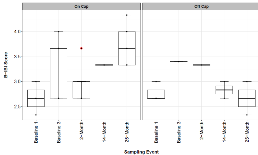
Figure 16. B-IBI Scores from the Benthic Community Census, Separated by Stations On and Off the Cap Footprint. Results are plotted as the median (horizontal bar), IQR (limits of boxes are 25th and 75th percentiles), and error bars extend from the IQR to the lowest value within 1.5 \times \text{IQR} . Data beyond the end of the whiskers are outliers and plotted as red points (as specified by Tukey).
