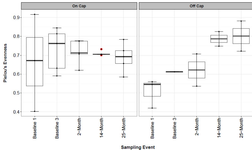
Figure 15. Pielou's Evenness Index from the Benthic Community Census, Separated by Stations On and Off the Cap Footprint. Results are plotted as the median (horizontal bar), IQR (limits of boxes are 25th and 75th percentiles), and error bars extend from the IQR to the lowest value within 1.5 * \text{IQR} . Data beyond the end of the whiskers are outliers and plotted as red points (as specified by Tukey).
