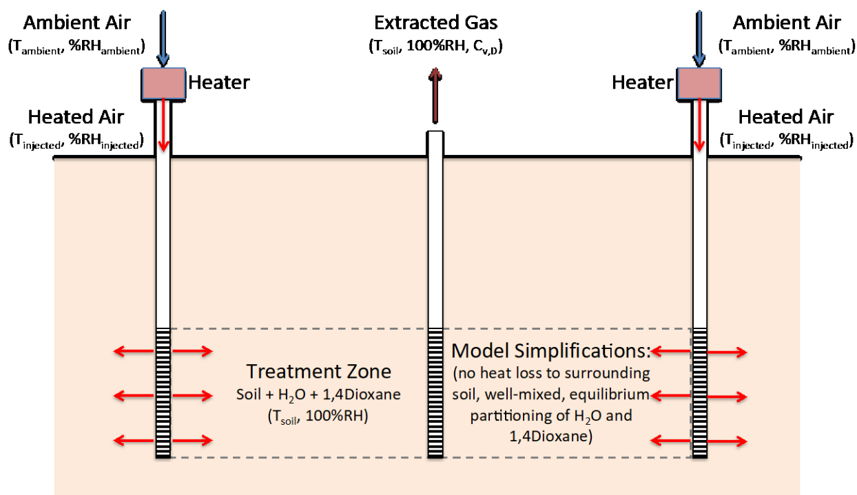
Figure 5.8.2. Simplified Conceptualization of the XSVE Treatment Process.
