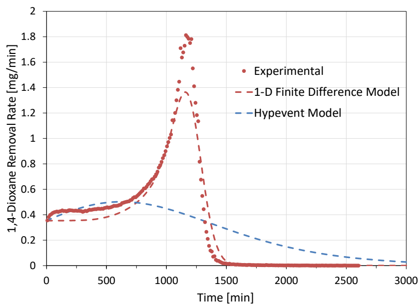
Figure 5.9.10. Experimental Column and Simulated 1,4-dioxane Removal Rates (HypeVent XSVE and 1-D models) for the 50°C 100% RH Column Run.
