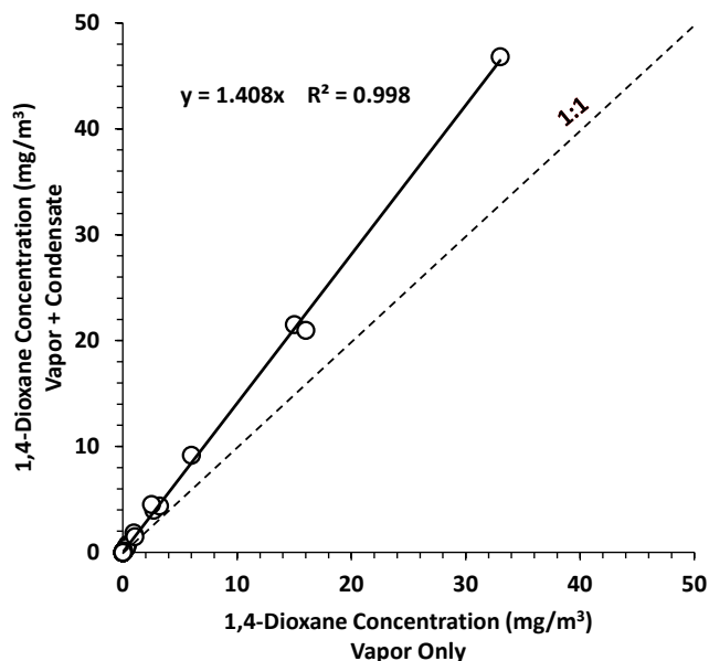
Figure 5.7.1. 1,4-Dioxane Concentrations (mg/m³) Obtained Using Vapor/Condensate Sampling Apparatus during XSVE Operation.
