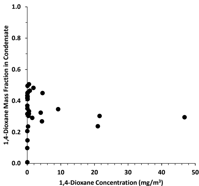
Figure 5.7.2. 1,4-Dioxane Mass Fraction in Condensate vs. 1,4-dioxane Concentration (mg/m³) Obtained Using Vapor/Condensate Sampling Apparatus During XSVE Operation for Samples with Detections in Both Vapor and Condensate Phases.
