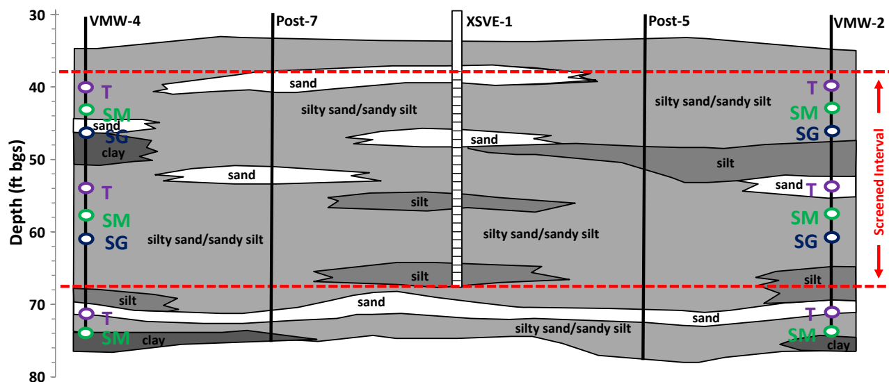
Figure 5.2.2. Geologic Cross-section for VMW-4 to VMW-2 Transect.
