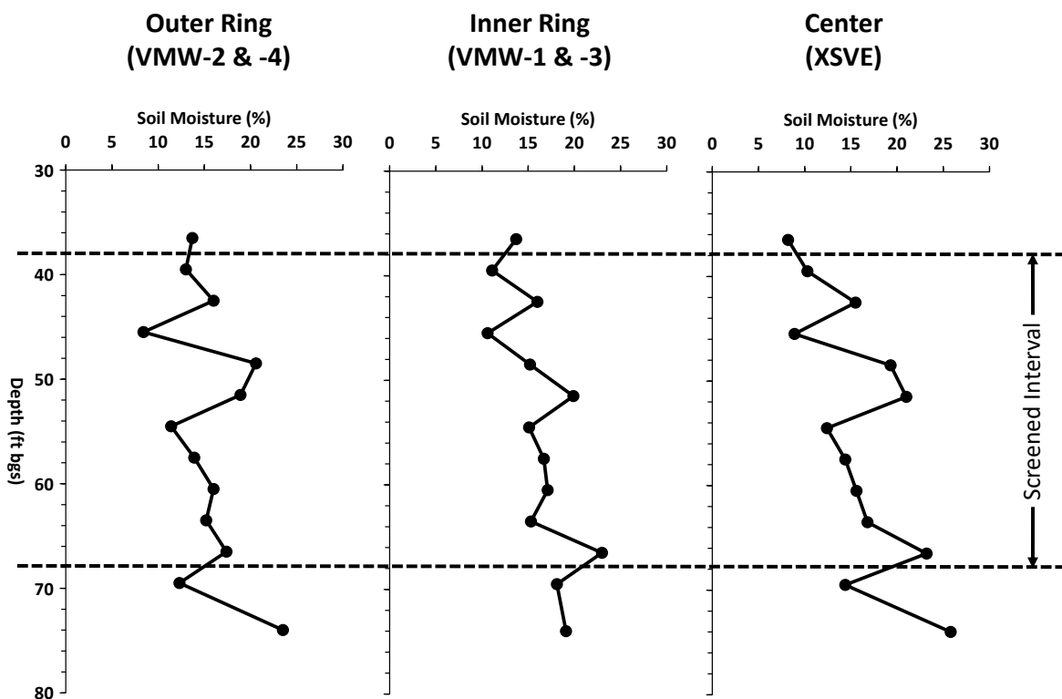
Figure 5.2.5. Soil Moisture Concentrations (%) prior to XSVE Operation.
