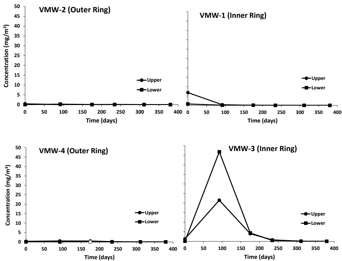
Figure 5.7.8 Treatment Zone 1,4-dioxane Concentrations (mg/m³) in Soil Gas during XSVE (open symbols are non-detects).
