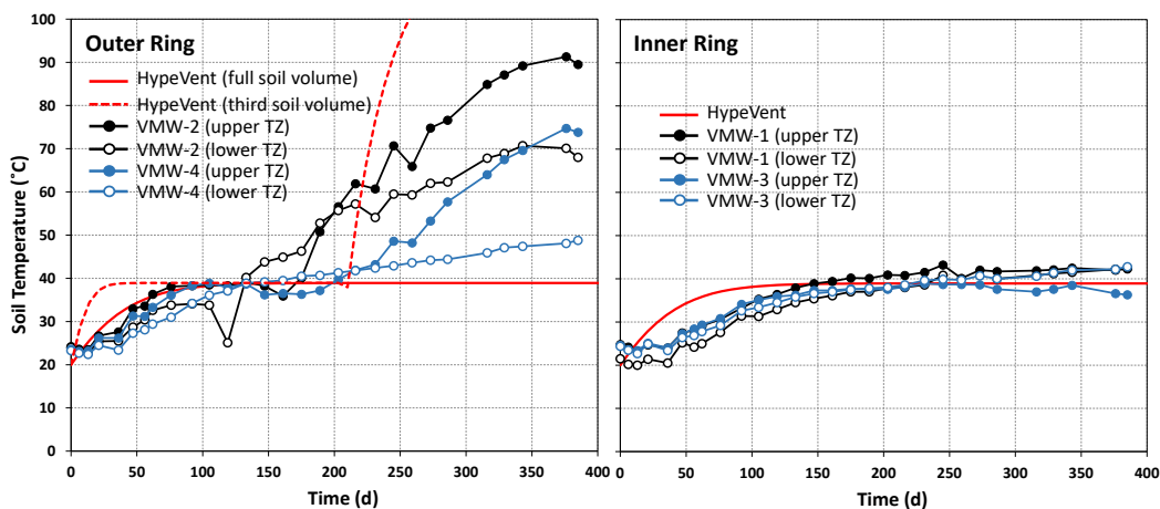
Figure 5.8.2. Soil Temperature Results for HypeVent XSVE and Actual Demonstration.
