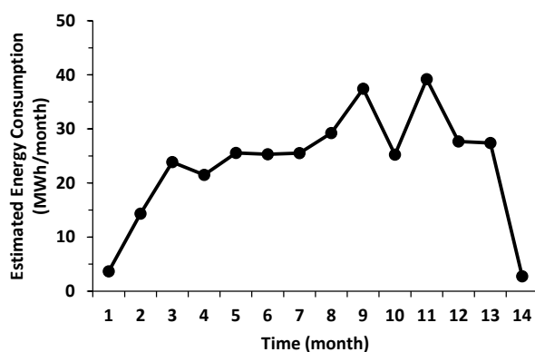
Figure 5.7.10. Estimated Power Consumption During XSVE Operation.
