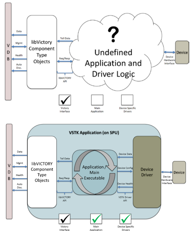
Figure 3: VSTK: Complete Picture
