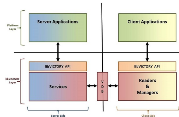
Figure 1: libVictory Software Design View [1]
