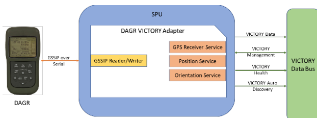
Figure 2: Example VICTORY Software Adapter
