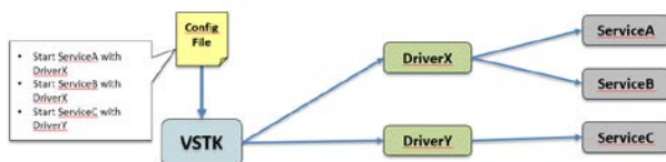
Figure 5: Configuring VSTK
