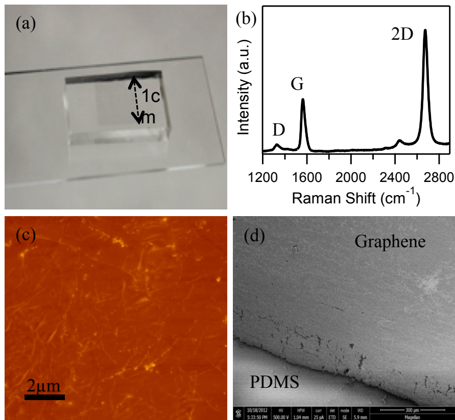
Figure 2.3. (a) Optical image of monolayer graphene on PDMS substrate. (b) Raman spectrum of monolayer graphene transfer-printed from PDMS to \text{SiO}_2/\text{Si} substrate. (c) AFM image of monolayer graphene surface on PDMS substrate. (d) SEM image of monolayer graphene border on PDMS substrate.
