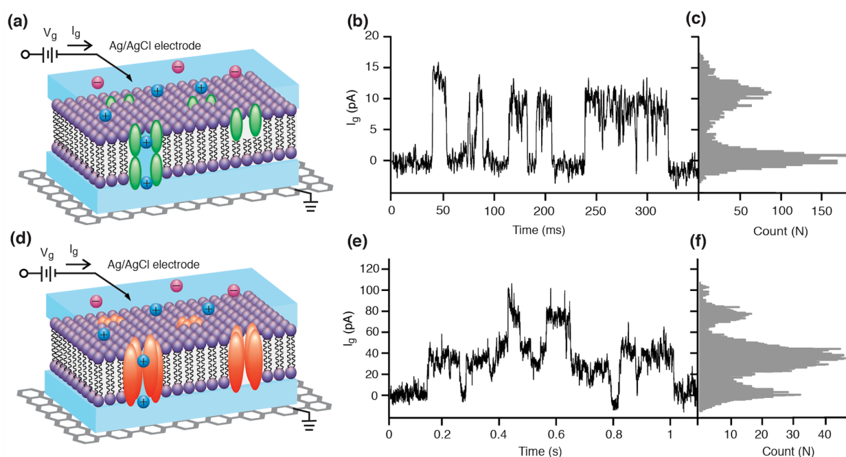
Figure 3.15. (a) Schematic diagram of SLBs with gA on graphene surface for ion channel activity detection. (b) Current trace for ion channel activity of gA at V_g = 100 mV in 1 M CsCl. (c) Histogram of current trace a. (d) Schematic diagram of SLBs with alamethicin on graphene surface for ion channel activity detection. (e) Current trace for ion channel activity of alamethicin at V_g = 100 mV in 100 mM KCl. (f) Histogram of current trace e.
