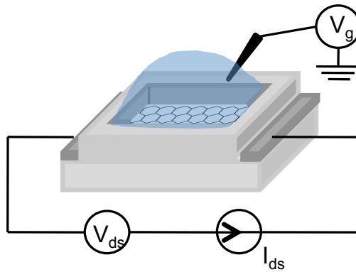
Figure 1.1. Schematic illustration of single layer graphene field-effect transistor on PDMS substrate.
