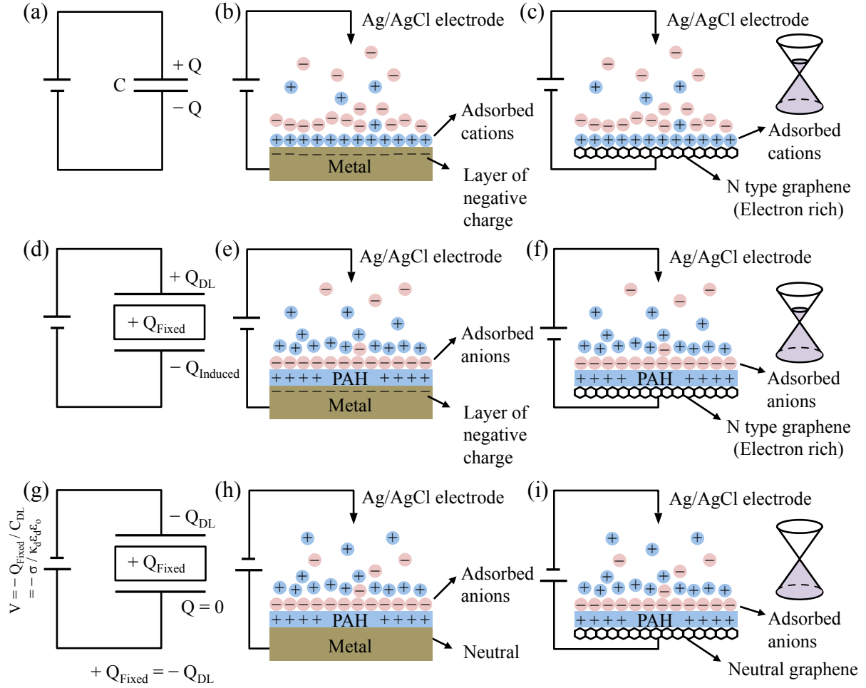
Figure 4.5. Explanation of electrostatic gating model of PAH on graphene. In the top row, for comparison, we show (a) the circuit model for an electrolyte in contact with an electrode, (b) the buildup of charge at a metal electrode in response to an applied voltage on the electrolyte, and (c) the analogous case for graphene in contact with an electrolyte. In the second row, we present the modification to the electrostatics when (d) a fixed charge is placed in between the capacitor plates, (e) a fixed charge of finite thickness is deposited on a metal in the presence of an electrolyte, and (f) a fixed charge of finite thickness is deposited on the surface of graphene. In the bottom row, we present the special case of a negative applied voltage that exactly cancels the induced charge. In circuit terms, (g), at a specific applied voltage, the fixed charge exactly
