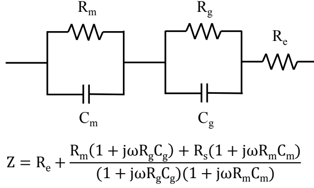
Figure 3.7. Equivalent circuit model with two time constants. R_e is the electrolyte resistance, R_g is the charge transfer resistance of the graphene/electrolyte interface, C_g stands for the double layer capacitance of the graphene/electrolyte interface in series with the quantum capacitance of the graphene sheet. R_m and C_m are the lipid layer resistance and capacitance.
