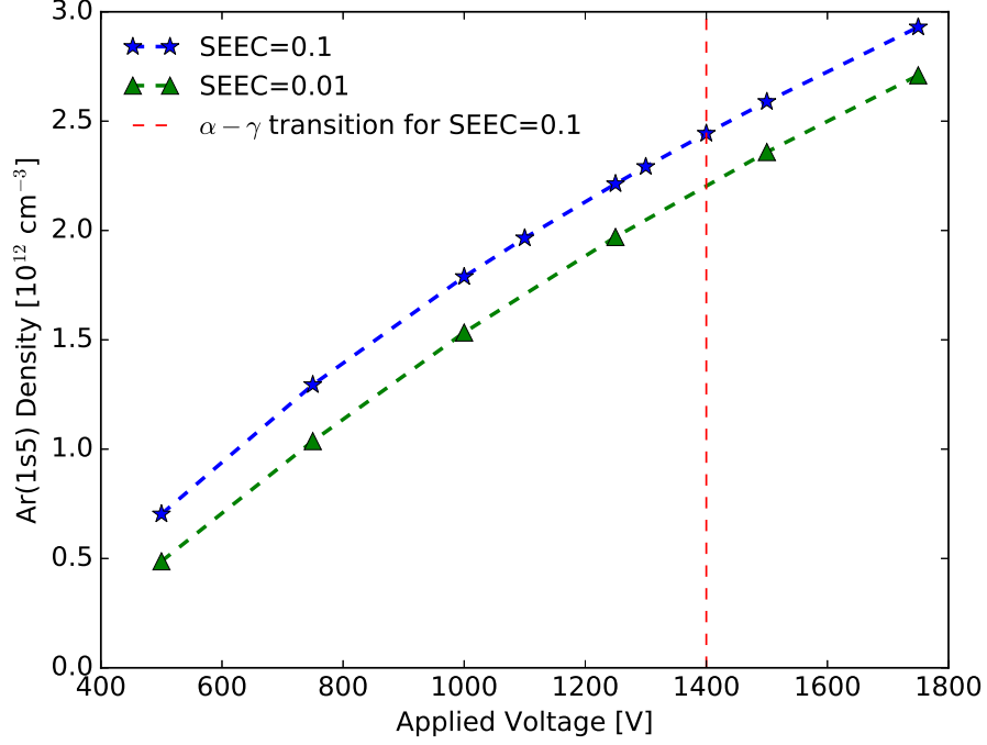
Figure 84. Cycle averaged bulk plasma metastable densities as a function of applied voltage for secondary electron emission coefficients (SEEC) of 0.1 and 0.01. The red dashed vertical line represents the onset of the \gamma -mode for the secondary coefficient of 0.1.
