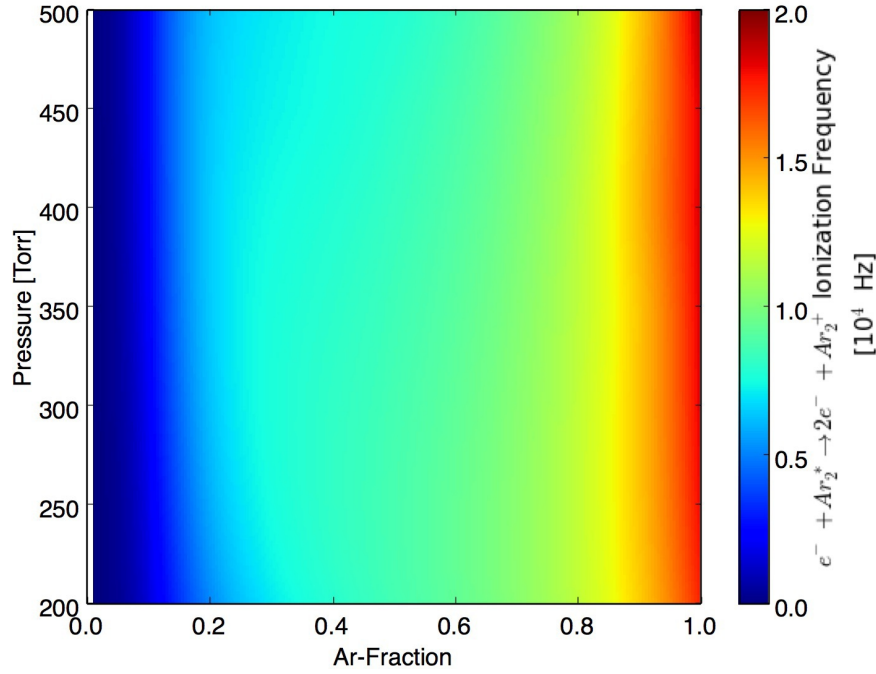
Figure 108. Ionization frequency of \text{Ar}_2^* + e^- \rightarrow \text{Ar}_2^+ + 2e^- as a function of Ar-fraction and pressure.
