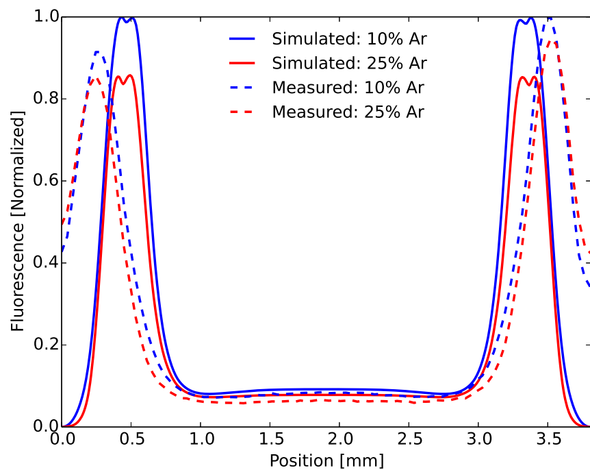
Figure 48. Normalized fluorescence measurements and one-dimensional simulations for 10 and 25% Ar-fractions at 300 Torr. Both the measurements and simulations are indicative of an \alpha -mode discharge.
