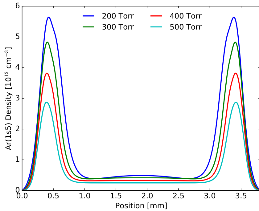
Figure 60. One-dimensional \text{Ar}(1s_5) density simulations for varying pressures in a 15% Ar in He mixture.
