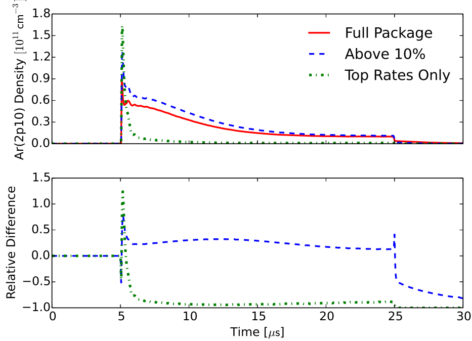
Figure 22. Simulated \text{Ar}(2p_{10}) densities for a 20 \mu\text{s} pulse, using the full reaction rate package and two reduced packages, along with the relative difference between the reduced rate packages compared to the full rate package.
