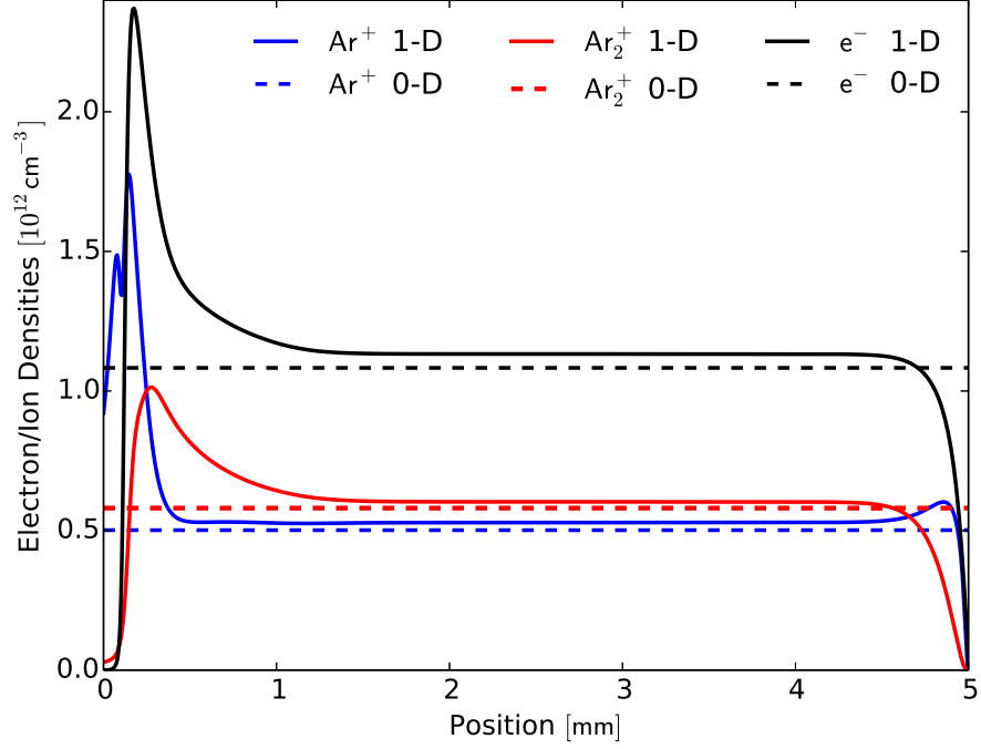
Figure 27. Spatial profile of electron and ion densities at the end of the 20 \mu\text{s} pulse.
