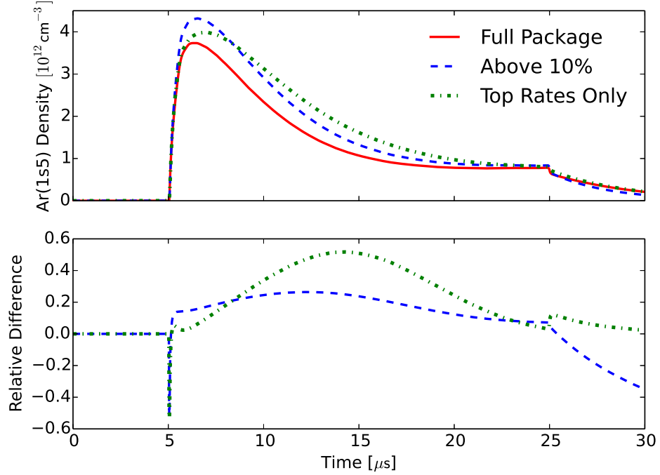
Figure 21. Simulated \text{Ar}(1s_5) densities for a 20 \mu\text{s} pulse, using the full reaction rate package and two reduced packages, along with the relative difference between the reduced rate packages compared to the full rate package.
