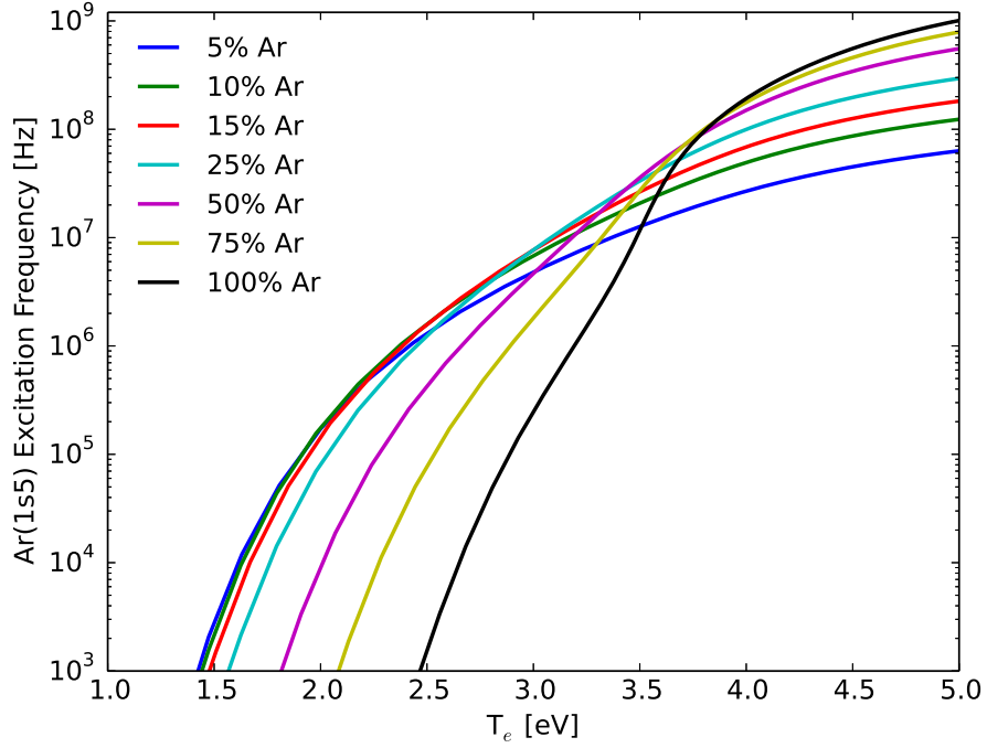
Figure 35. Metastable excitation frequencies, k_{exc}[Ar] , at 200 Torr for varying Ar-He mixtures, as calculated by BOLSIG+.
