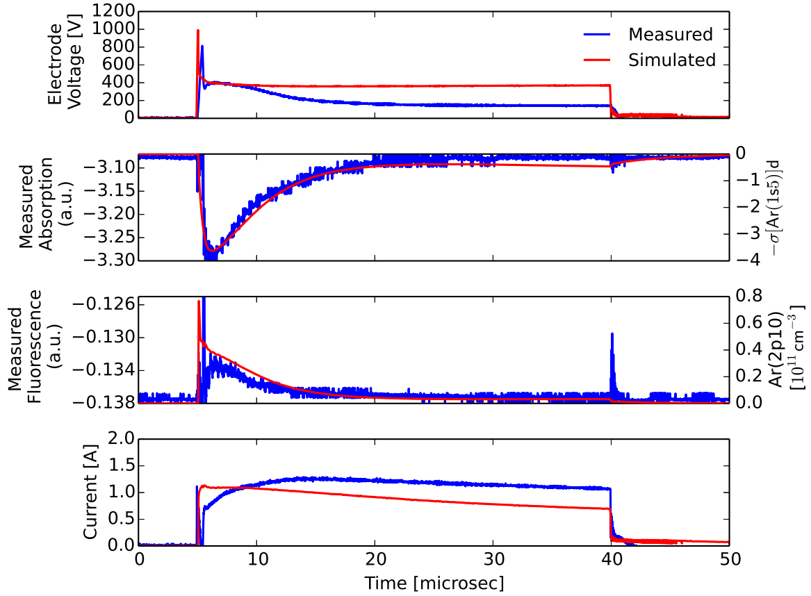
Figure 15. A comparison of the simulated and measured values for electrode voltage, V_E = V_2 - V_3 (top), Ar(1s_5) + \hbar\omega \rightarrow Ar(2p_9) absorption (middle top), Ar(2p_{10}) \rightarrow Ar(1s_5) + \hbar\omega fluorescence (middle bottom), and discharge current I_3 (bottom) for a 35 \mu s pulse.
