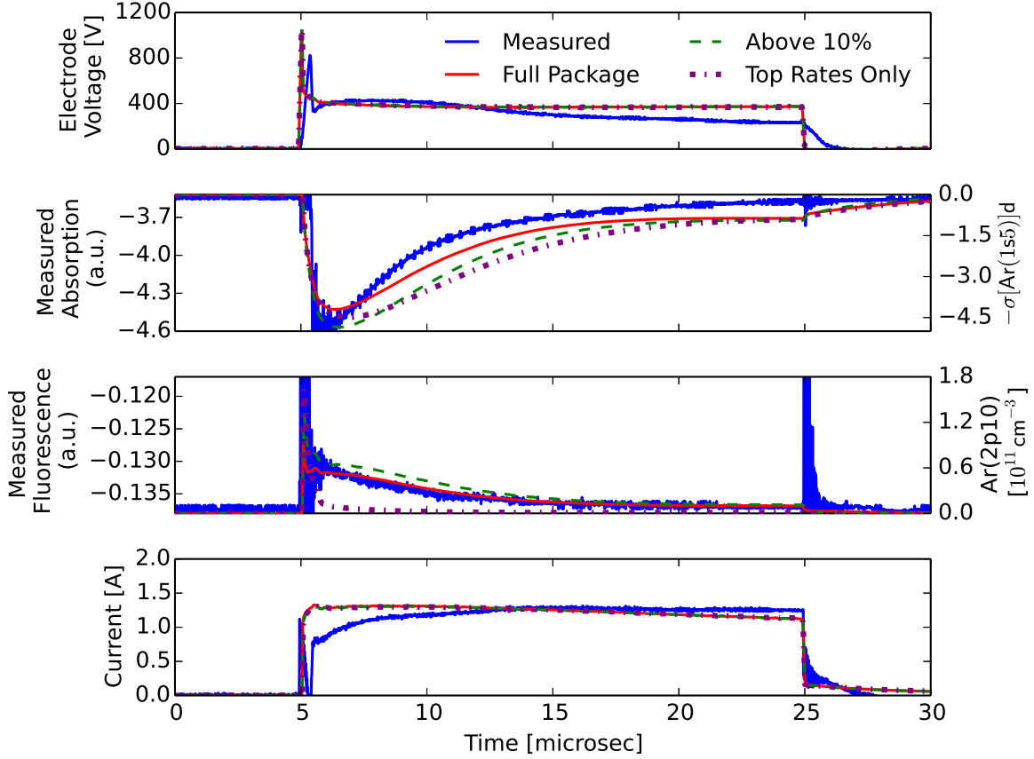
Figure 20. Simulated electrode voltage, absorption, fluorescence, and current for the 20 \mu s pulse scenario using a variety of reaction rate packages: full rate package, excluding pathways below 10% of the total rate for each species, and only the top pathways for each species.
