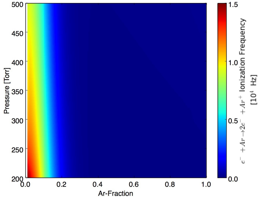
Figure 107. Ionization frequency of \text{Ar} + e^- \rightarrow \text{Ar}^+ + 2e^- as a function of Ar-fraction and pressure.
