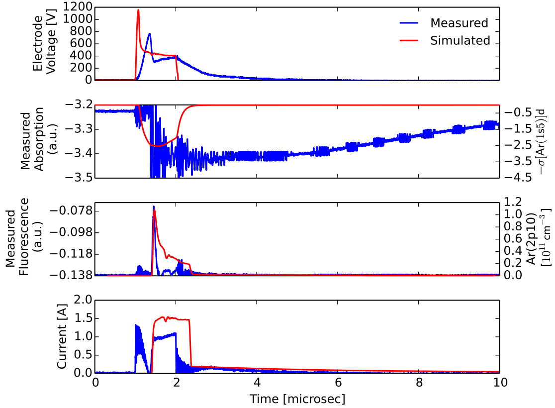
Figure 12. A comparison of the simulated and measured values for electrode voltage, V_E = V_2 - V_3 (top), Ar(1s_5) + \hbar\omega \rightarrow Ar(2p_9) absorption (middle top), Ar(2p_{10}) \rightarrow Ar(1s_5) + \hbar\omega fluorescence (middle bottom), and discharge current I_3 (bottom) for a 1 \mu s pulse. Radiation trapping for the Ar(1s_4) \rightarrow Ar + \hbar\omega transition is not included in this simulation.
