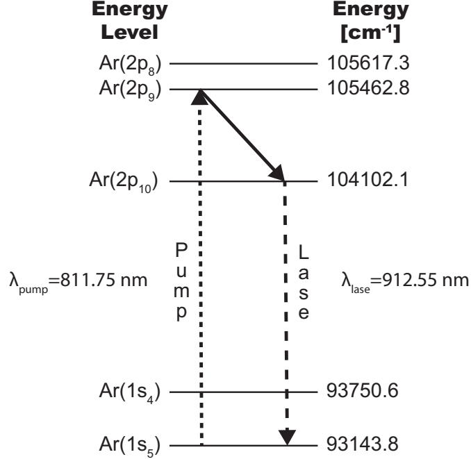
Figure 1. A diagram of energy levels pertinent to an optically pumped rare gas laser with Ar as the rare gas. Optical pumping from Ar(1s_5) to Ar(2p_9) is followed by a non-adiabatic transition to Ar(2p_{10}) and subsequent lasing to Ar(1s_5) . Lasing to Ar(1s_4) is also possible, and Ar(2p_8) is included due to its proximity to the pumping level Ar(2p_9) .
