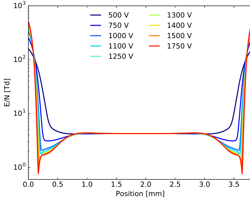
Figure 83. RMS E/N magnitudes for a variety of applied voltages at a pressure of 200 Torr and a 15% Ar-fraction using a secondary emission coefficient of 0.1.
