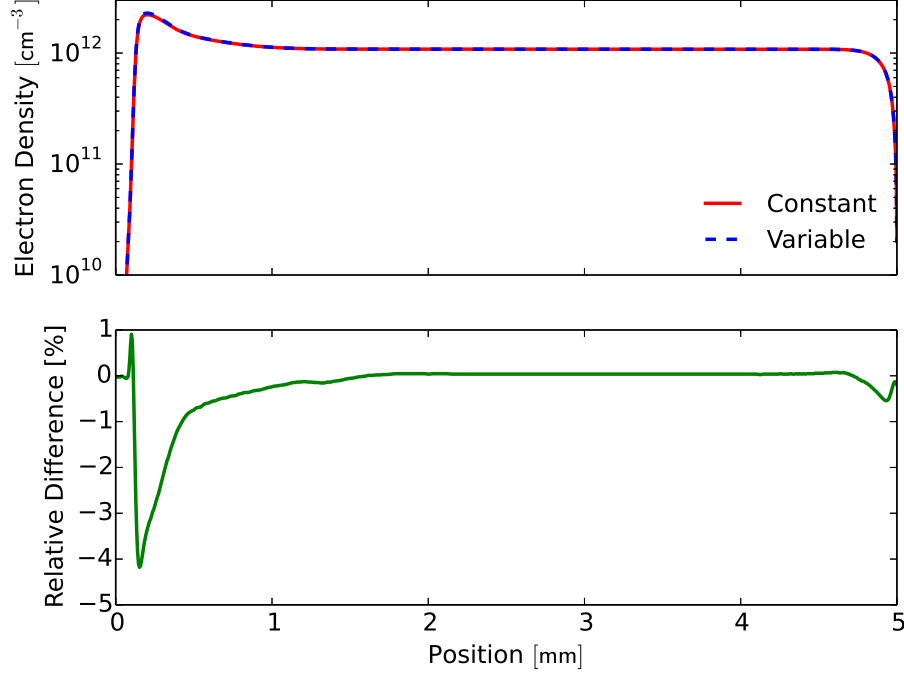
Figure 30. Spatial electron density profiles 10 \mu\text{s} after pulse initiation using constant and variable EEDF calculations.
