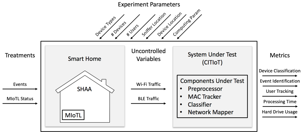
Figure 33. System Under Test and Component Under Test diagram
