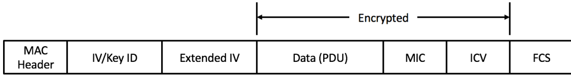
Figure 1. MPDU format when using WPA2 [3]
