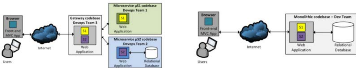
Figure 5: Microservices Architecture vs. Monolithic Architecture [51]
