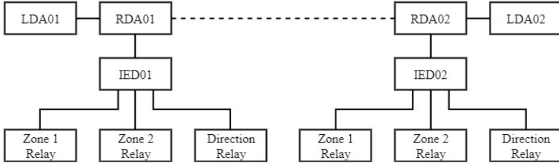
Figure 4. WABPS Physical Implementation
