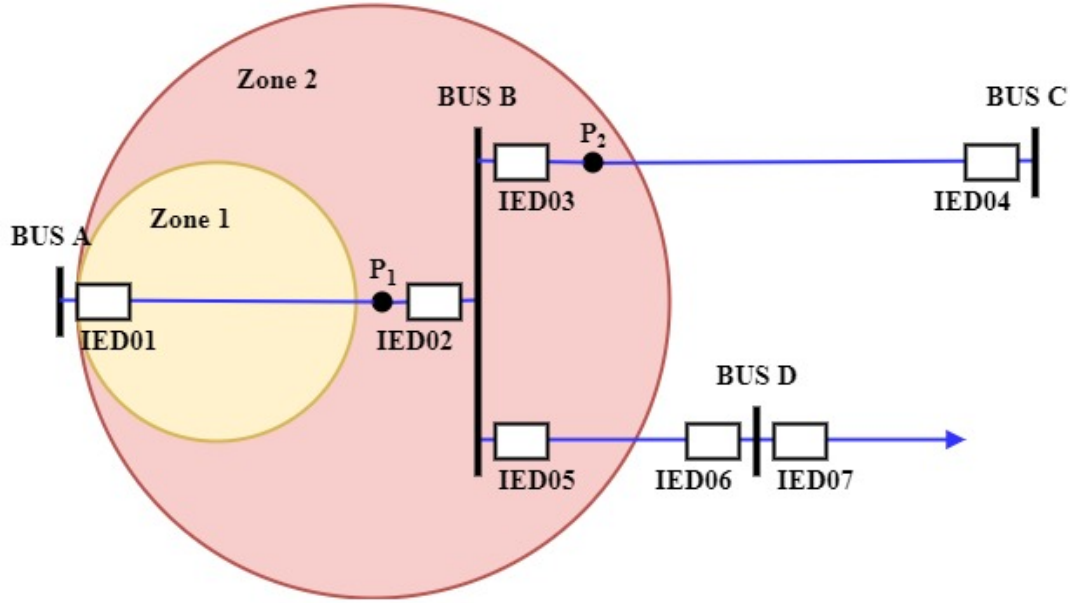
Figure 1. Range of Zone Distance Relays
