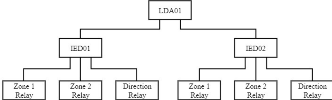
Figure 5. WABPS Model Implementation
