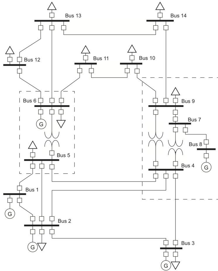
Figure 2. IEEE 14-Bus System
