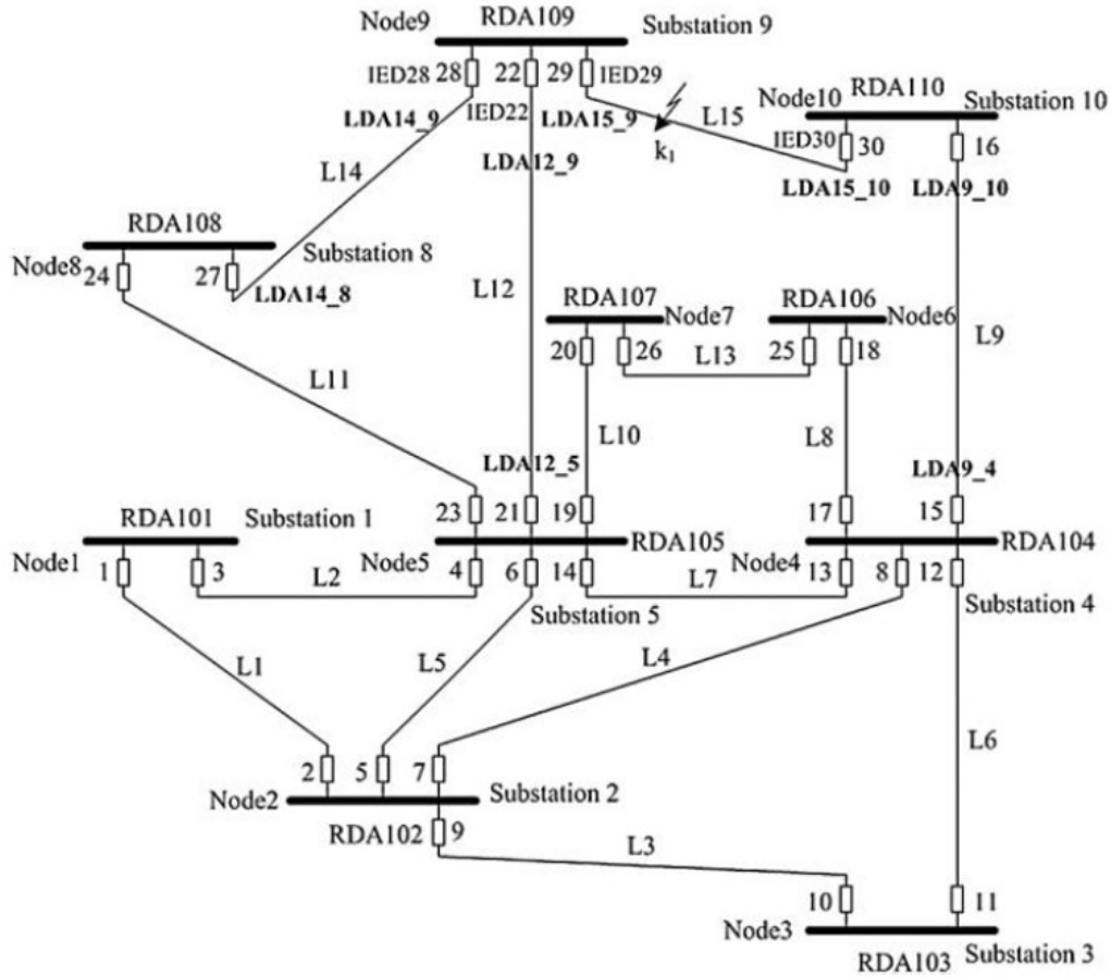
Figure 3. WABPS Modified IEEE 14-Bus System [41]
