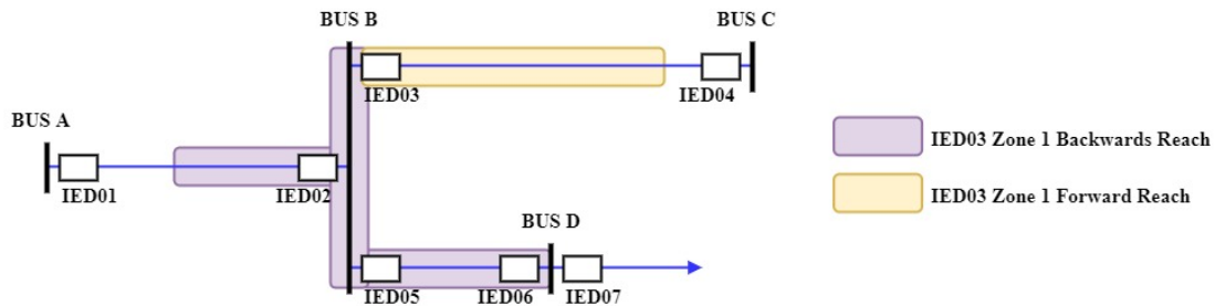
Figure 6. Back Reach of Zone Distance Relays
