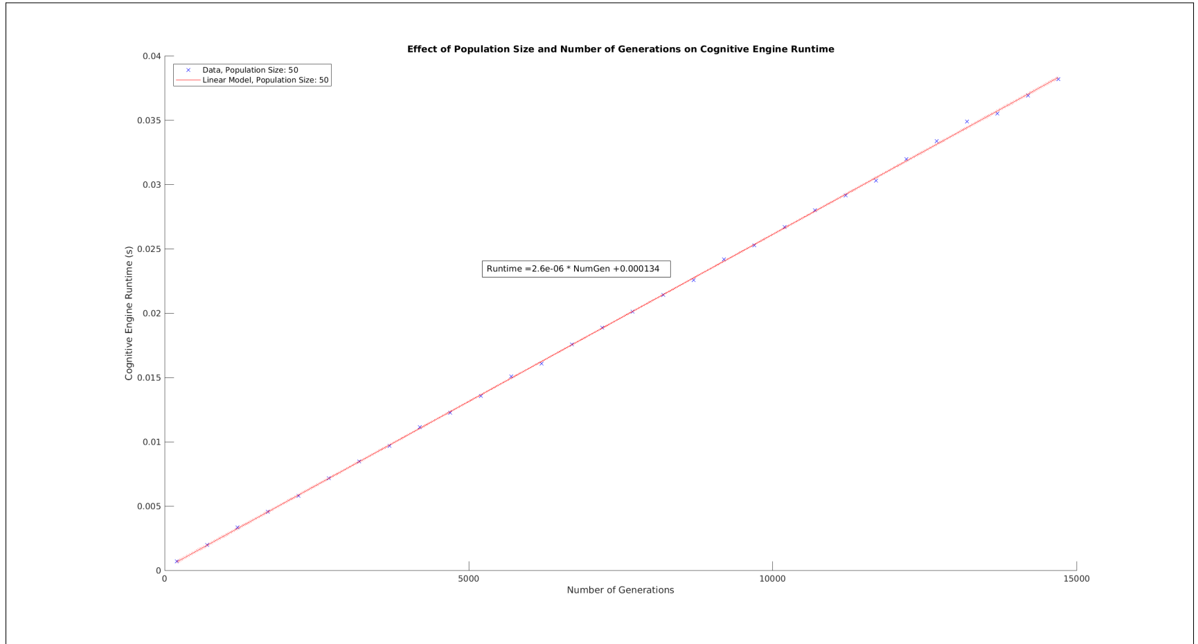
Figure 26. OMNeT++ engine runtime performance with respect to umber of generations used to evolve solutions
