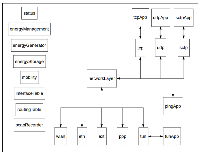
Figure 13. Internal structure of the “Adhoc Host” module type
