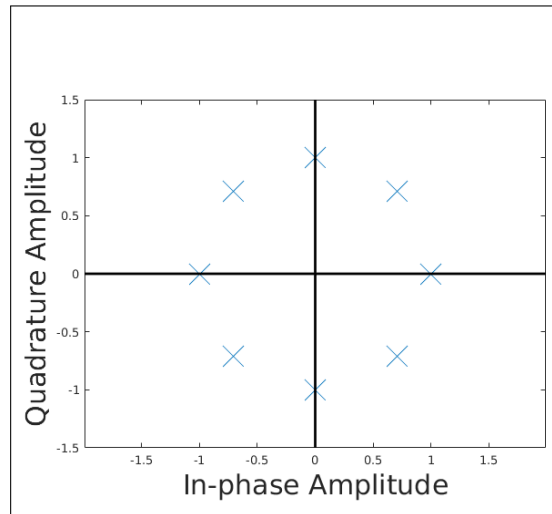
Figure 10. Example PSK modulation scheme constellation using a modulation order of 8 with each symbol representing 3 bits
