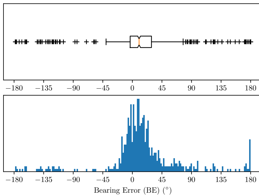
Figure 31. Bearing Error Histogram with a Focused Capture Width of 84^\circ
