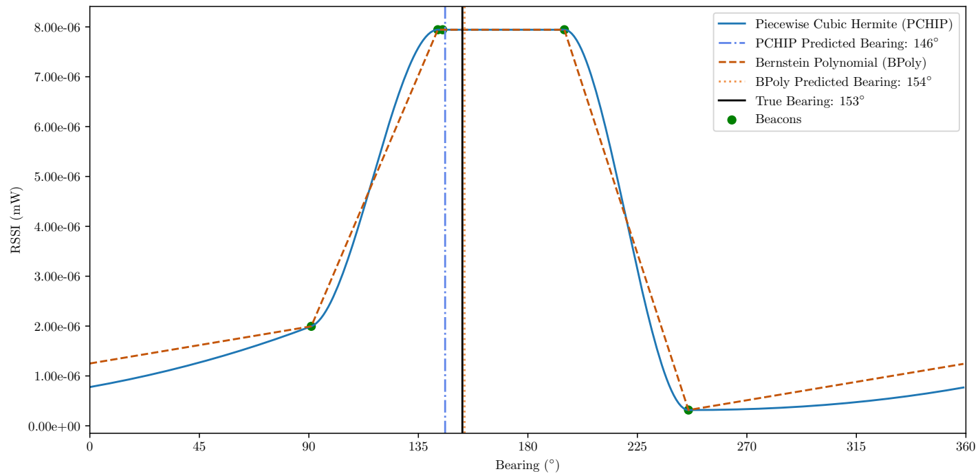
Figure 21. Interpolation of 5-Sample Capture using PCHIP and BPoly Interpolation Methods
