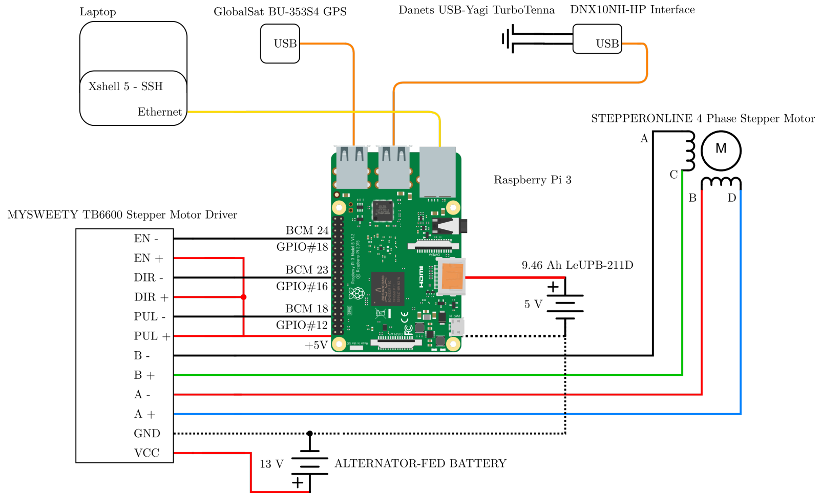
Figure 10. Prototype Schematic
