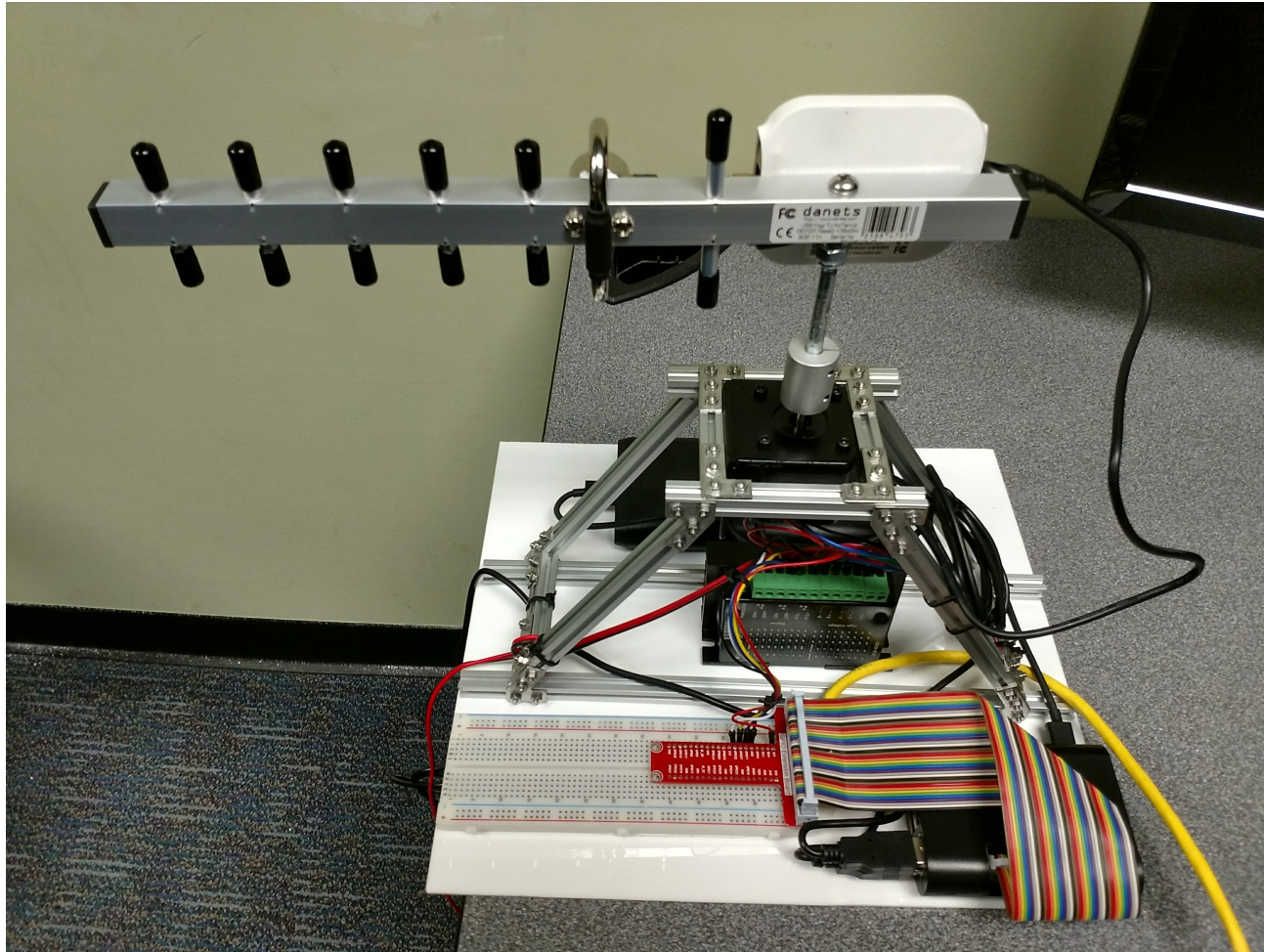
Figure 12. Assembled Prototype
