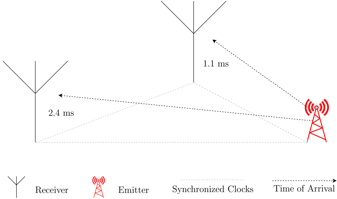
Figure 4. Time of Arrival - One Receiver for Distance, Two Receivers for Location
