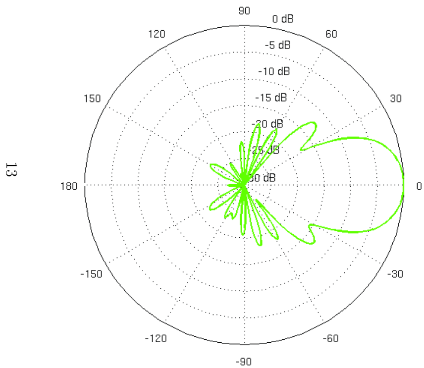
(a) Yagi Azimuth Plane Pattern
