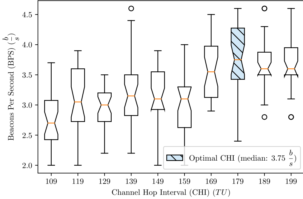
Figure 19. Channel Hop Interval (CHI) Treatment Results
