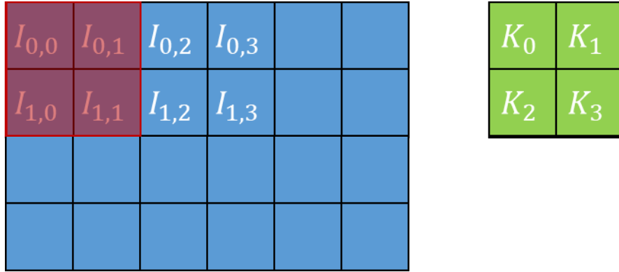
Figure 5. Visual representation of the convolution operation, with the kernel parameters in green, the window in red, and the input matrix in blue.
