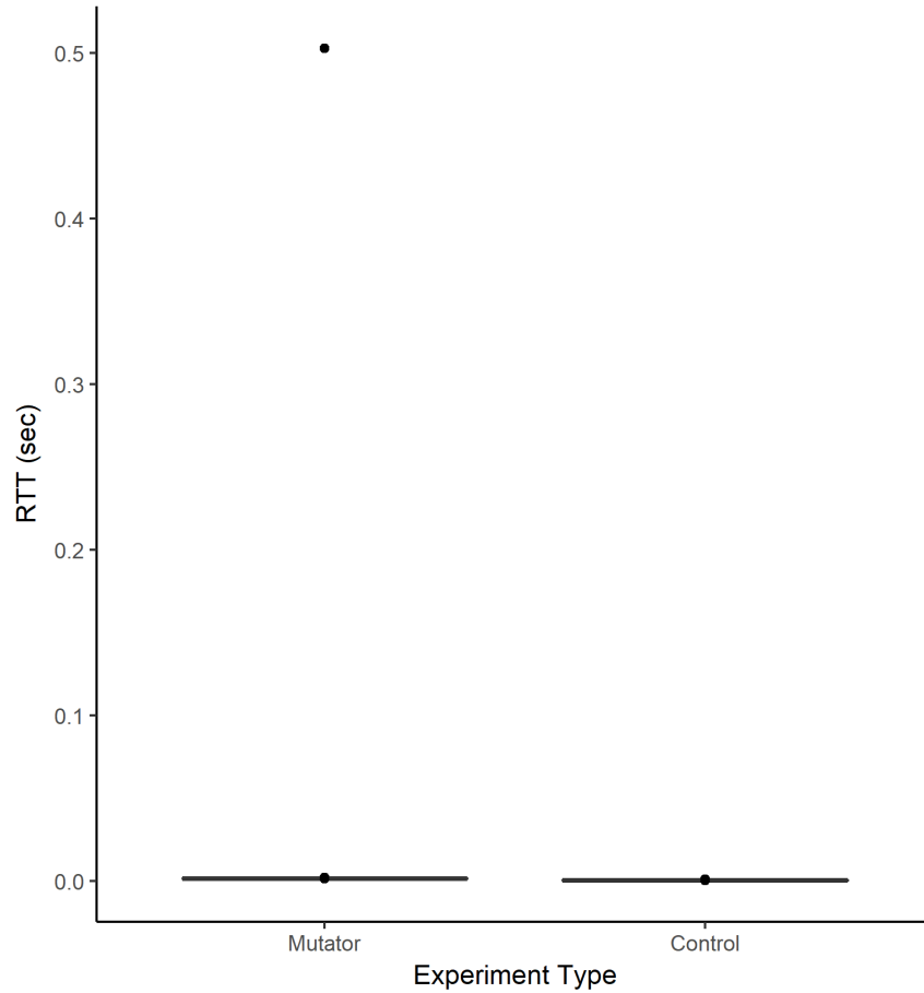
Figure 26. Box & Whisker Plot of RTT Between Control and Mutator Trials for IMAP
