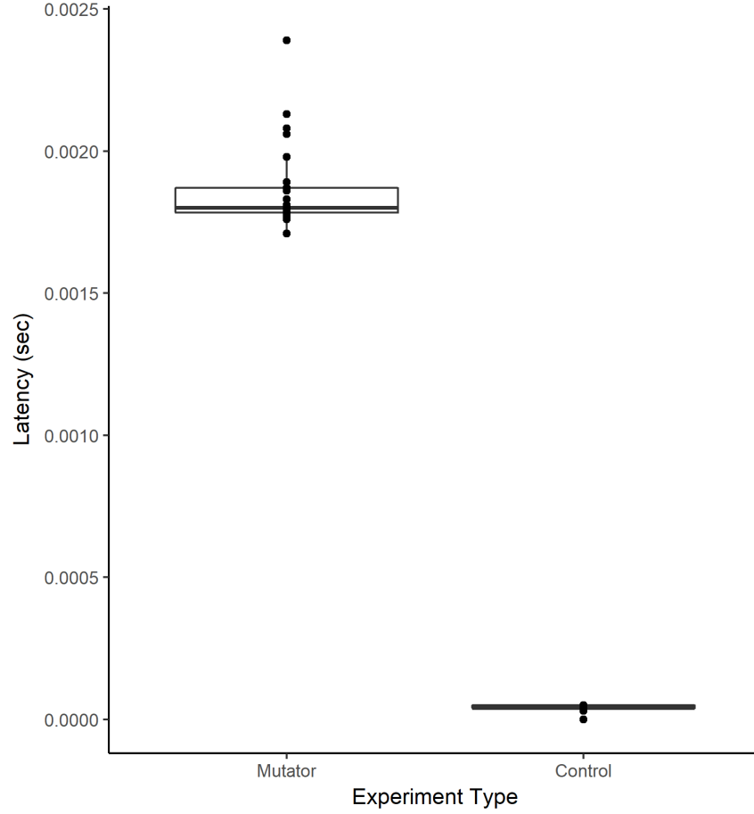
Figure 21. Box & Whisker Plot of Latency Between Control and Mutator Trials for HTTP
