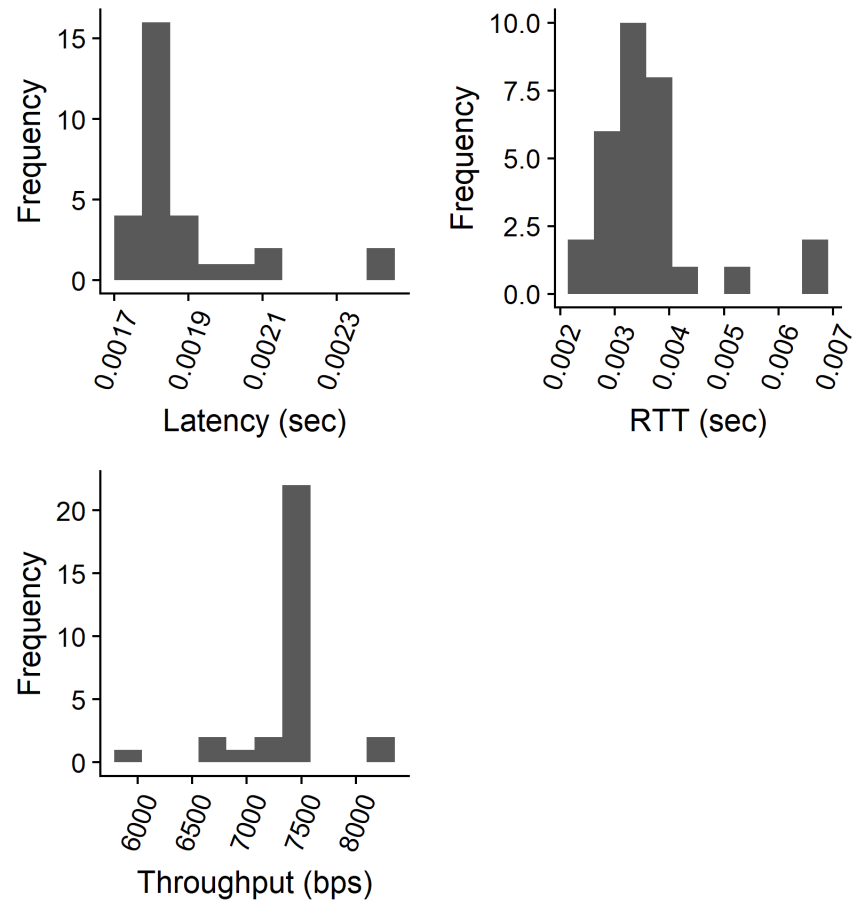
Figure 46. Histograms of HTTP QoS Mutator Data
