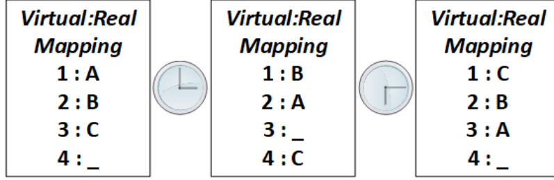
Figure 10. rIP:vIP Mutations Example
