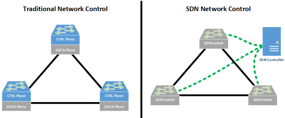
Figure 1. Separation of Control and Data Planes in Traditional Networks Versus a SDN [2]
