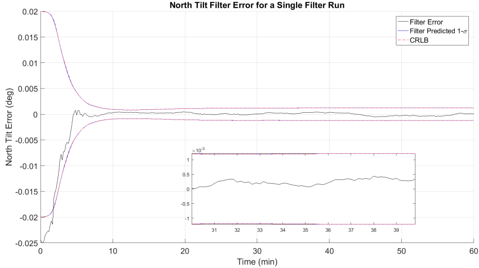
Figure 41. EKF Error in North Tilt Error States for the TEN-NAV Case
