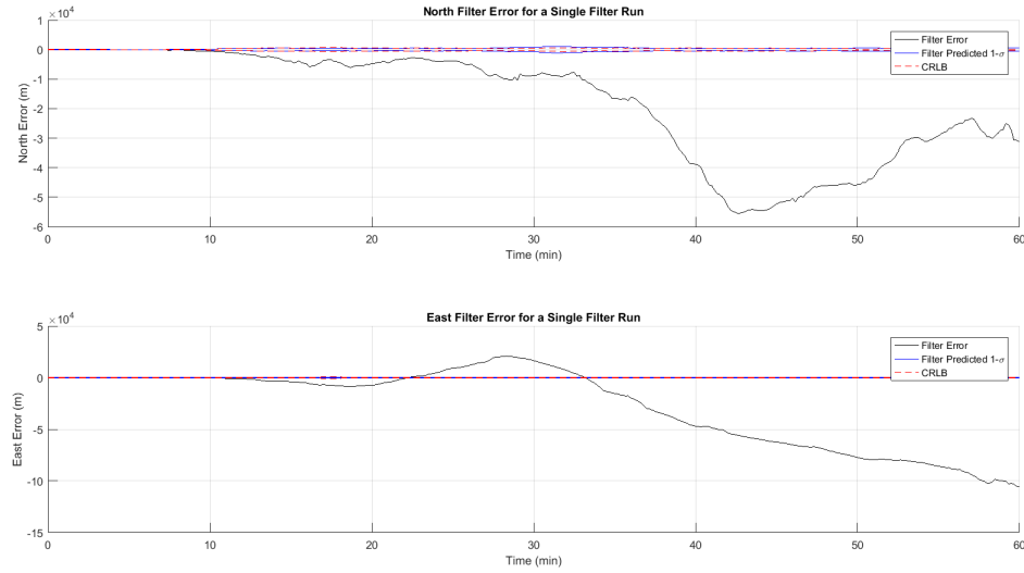
Figure 59. EKF Error in Horizontal Position States for a Single Run - TEN-TACT Case
