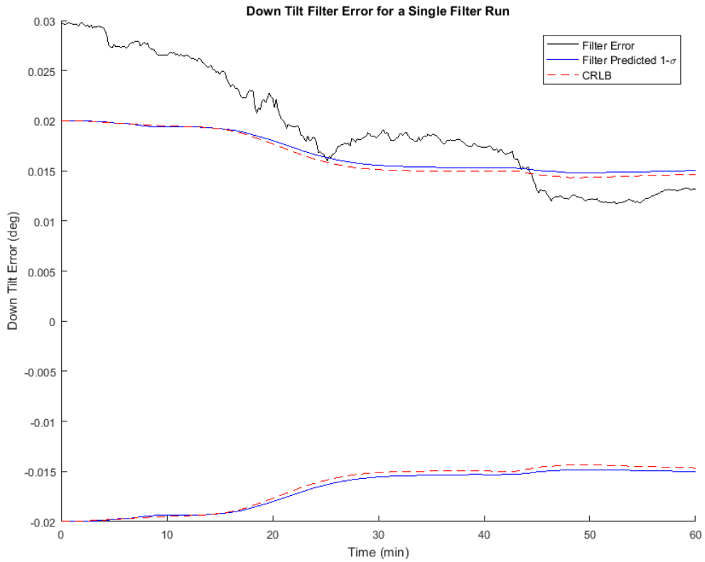
Figure 43. EKF Error in Down Tilt Error States for the TEN-NAV Case
