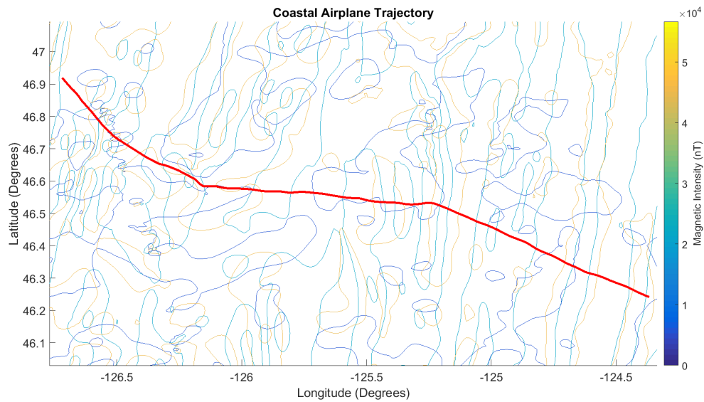
Figure 45. Airplane Trajectory Overlayed Onto Vector Field Maps
