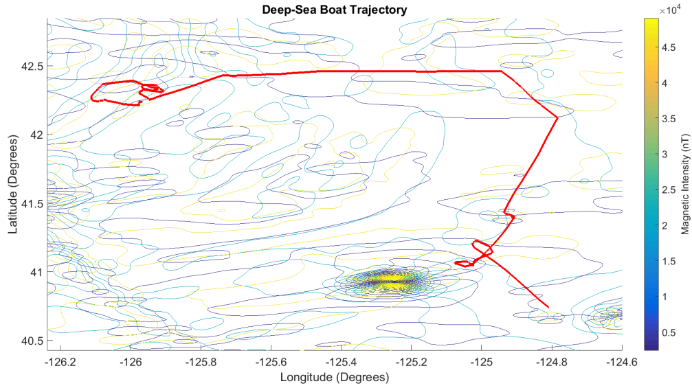
Figure 69. Boat Trajectory Overlayed Onto Vector Field Maps
