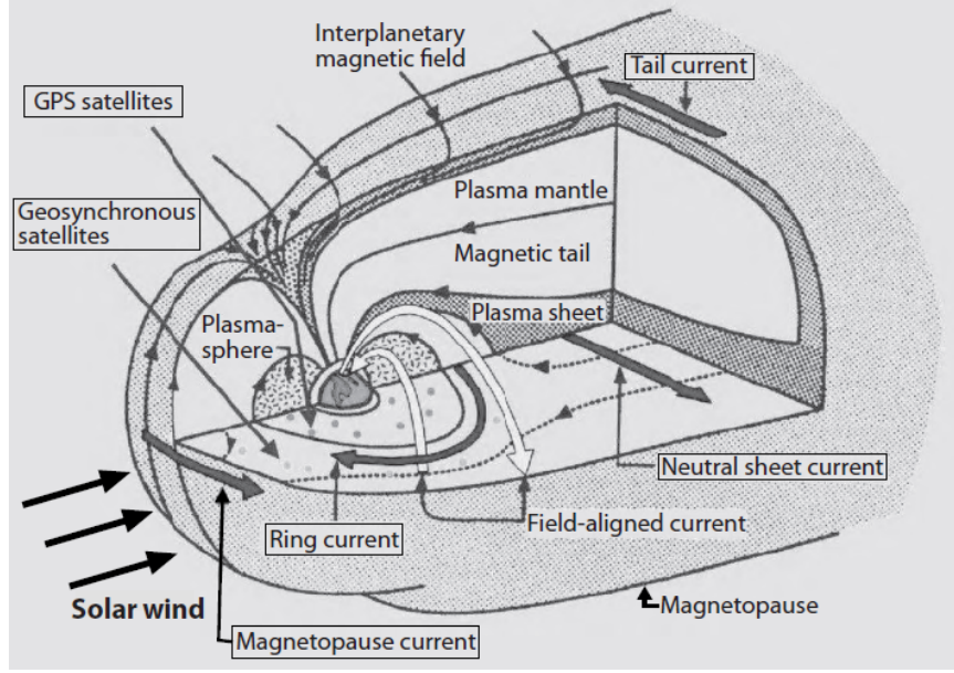
Figure 2. Earth's Magnetosphere [12]
