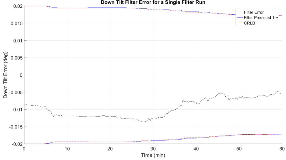
Figure 65. EKF Error in Down Tilt Error States for a Single Run - TEN-NAV Case
