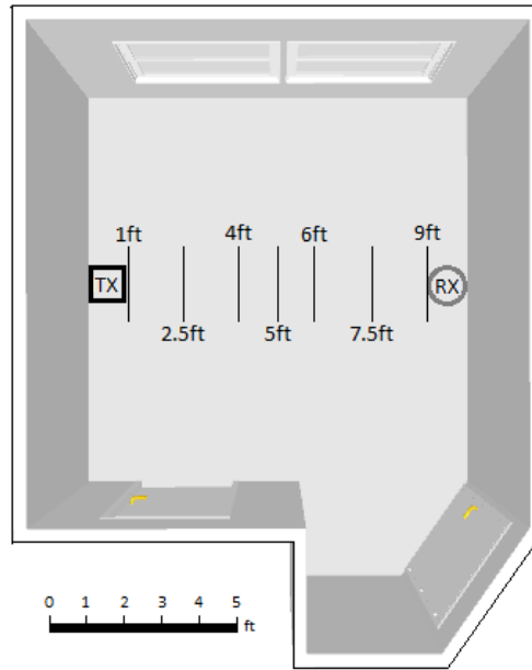
Figure 10. Diagram of apartment room without furniture, with one transmitting device (TX) and one receiving device (RX), and with LOS distances marked
