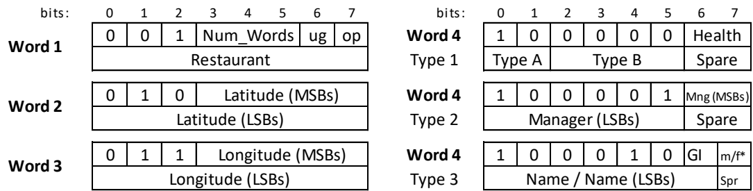
Figure 41. Bit maps for the words in the Restaurant Locator Protocol
