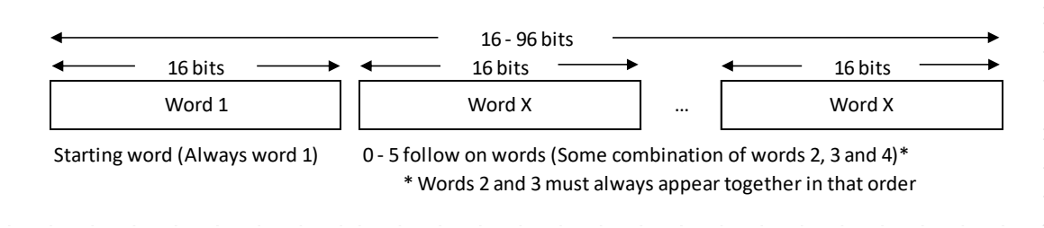
Figure 40. The structure of a message in the Restaurant Locator Protocol
