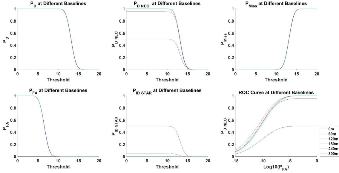
Figure 27: Algorithm Performance with Satellite Present in Data Frame and SNR of 3
