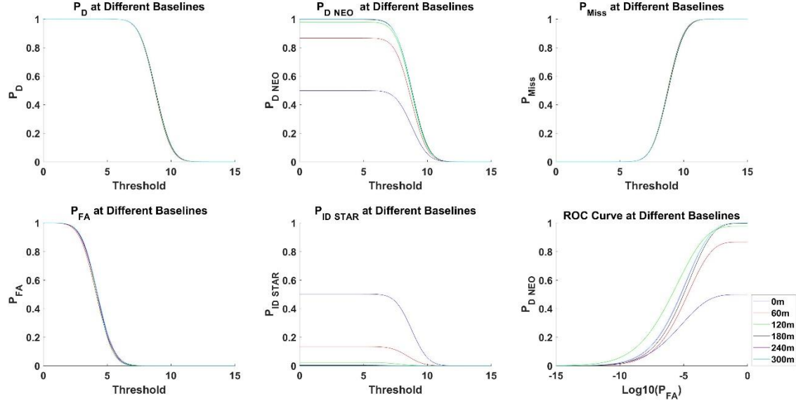
Figure 28: Algorithm Performance with Satellite Present in Data Frame and SNR of 2
