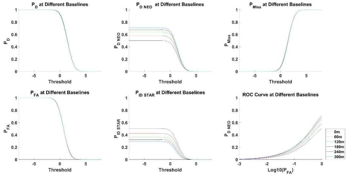
Figure 31: Algorithm Performance with Satellite Present in Data Frame and SNR of 1/3
