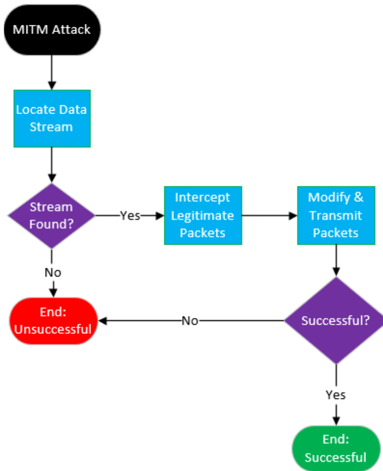
Figure 8. Man-in-the-Middle Attack
