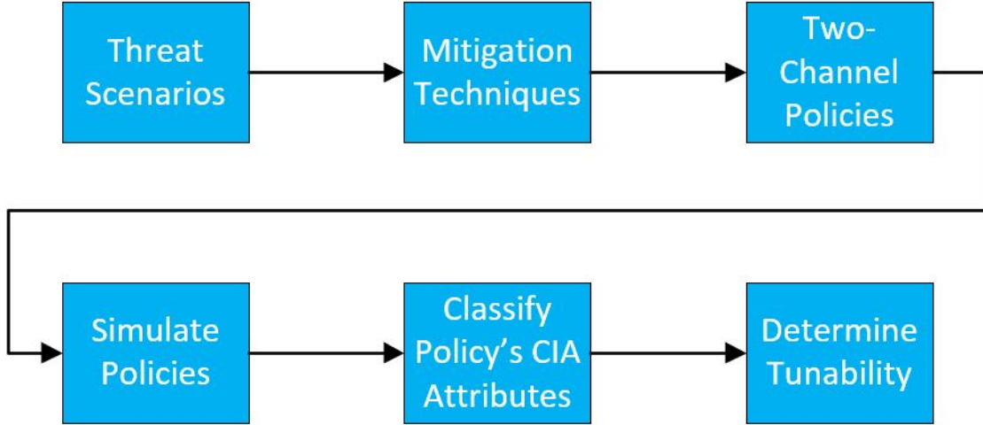
Figure 5. Methodology Flowchart
