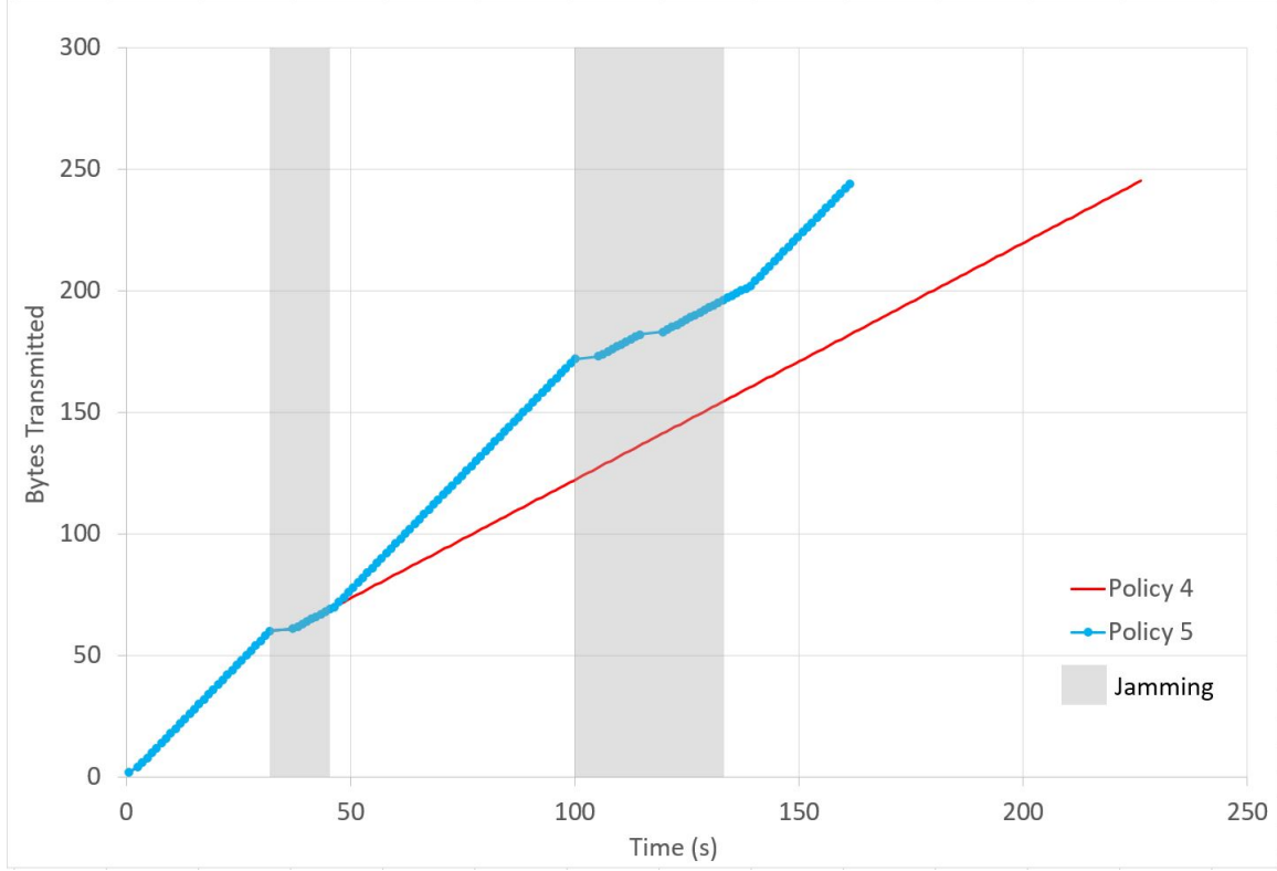
Figure 12. Jamming Scenario Throughput Comparison
